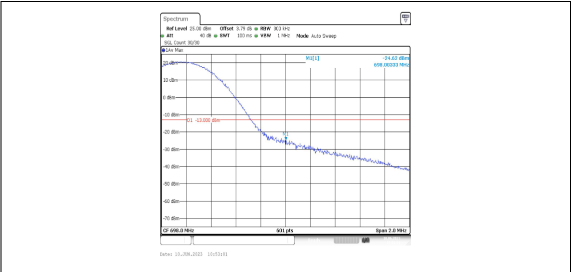
Band71-15MHz-16QAM-133397-1RB#74
