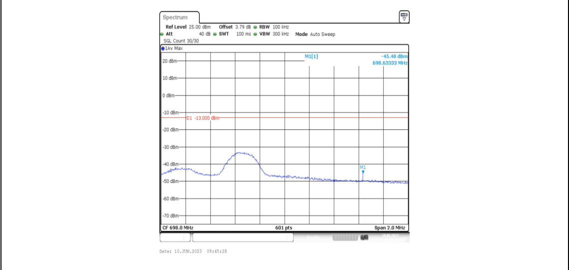
Band71-5MHz-16QAM-133447-1RB#0
