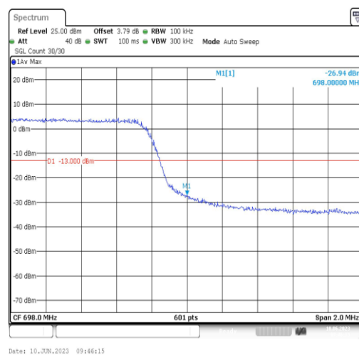
Band71-5MHz-16QAM-133447-25RB#0
