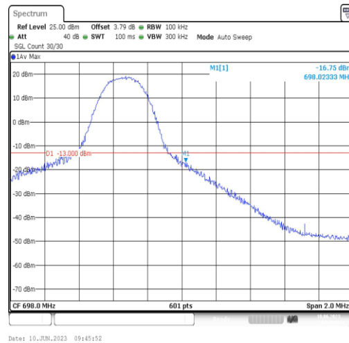
Band71-5MHz-16QAM-133447-1RB#24
