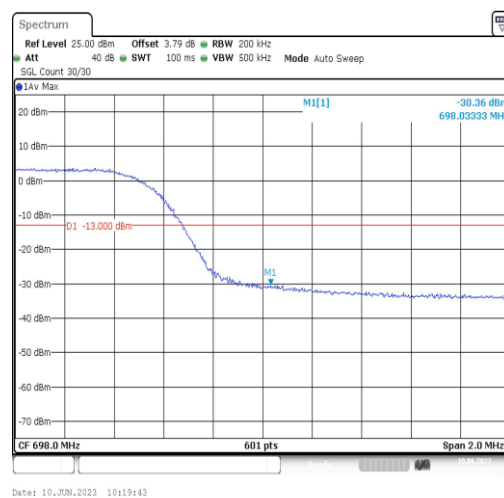
Band71-10MHz-16QAM-133422-50RB#0
