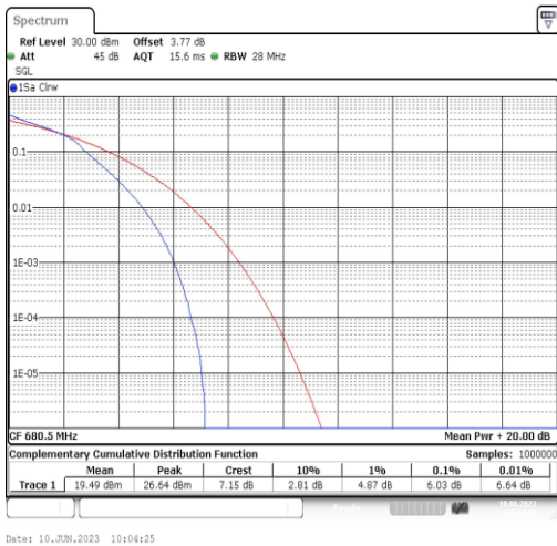
Band71-5MHz-16QAM-133297-25RB#0
