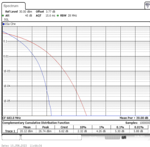
Band71-20MHz-QPSK-133322-100RB#0
