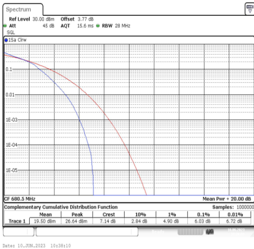
Band71-10MHz-16QAM-133297-50RB#0
