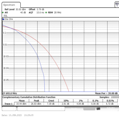
Band71-10MHz-16QAM-133422-50RB#0
