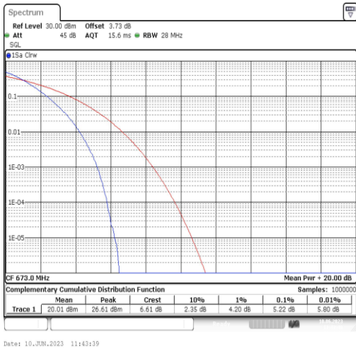
Band71-20MHz-QPSK-133222-100RB#0
