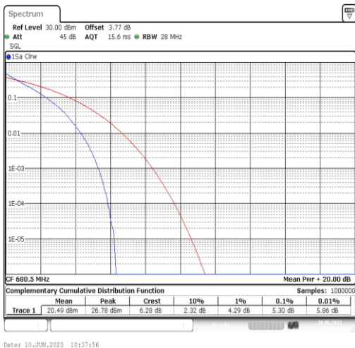
Band71-10MHz-QPSK-133297-50RB#0
