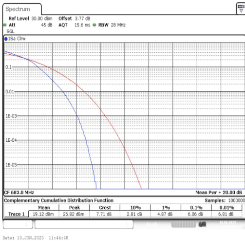
Band71-20MHz-16QAM-133322-100RB#0
