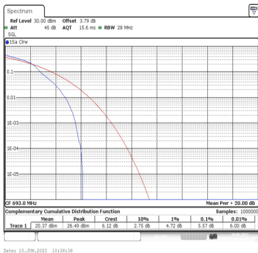
Band71-10MHz-16QAM-133422-1RB#0
