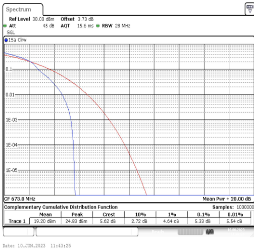
Band71-20MHz-16QAM-133222-1RB#0
