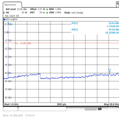
Band66-5MHz-QPSK-132322-1RB#0-Range4:1000~20000MHz
