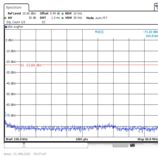
Band66-10MHz-QPSK-132322-1RB#0-Range2:0.15~30MHz
