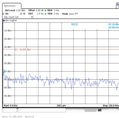
Band66-1.4MHz-QPSK-132665-1RB#0-Range1:0.009~0.15MHz
