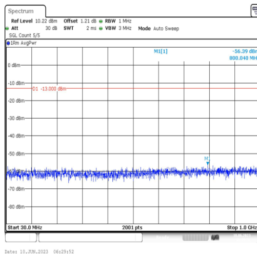
Band66-1.4MHz-16QAM-132322-1RB#0-Range3:30~1000MHz
