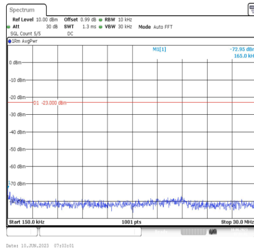
Band66-3MHz-QPSK-132657-1RB#0-Range2:0.15~30MHz
