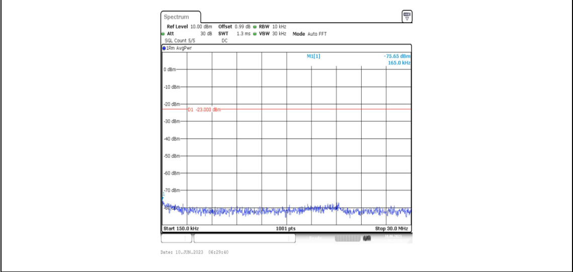
Band66-1.4MHz-16QAM-132322-1RB#0-Range2:0.15~30MHz
