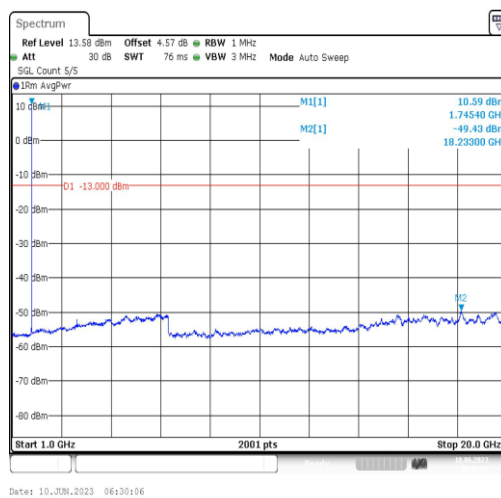
Band66-1.4MHz-16QAM-132322-1RB#0-Range4:1000~20000MHz
