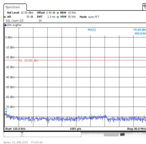
Band66-5MHz-16QAM-132322-1RB#0-Range2:0.15~30MHz
