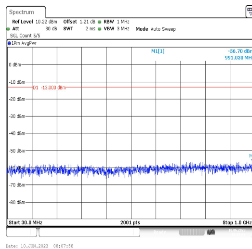
Band66-10MHz-QPSK-132322-1RB#0-Range3:30~1000MHz
