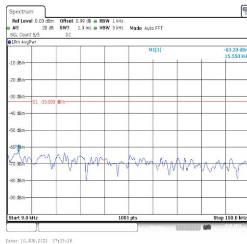
Band66-5MHz-16QAM-132322-1RB#0-Range1:0.009~0.15MHz
