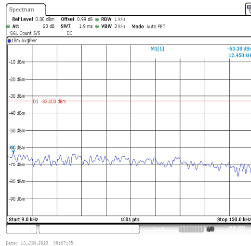
Band66-10MHz-QPSK-132322-1RB#0-Range1:0.009~0.15MHz
