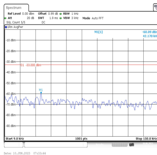
Band66-5MHz-16QAM-131997-1RB#0-Range1:0.009~0.15MHz
