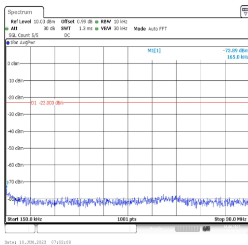
Band66-3MHz-16QAM-132322-1RB#0-Range2:0.15~30MHz
