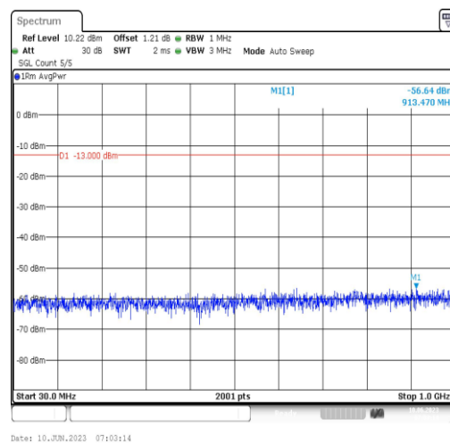
Band66-3MHz-QPSK-132657-1RB#0-Range3:30~1000MHz
