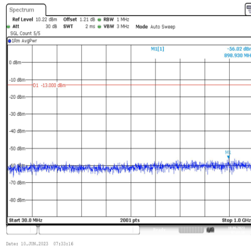
Band66-5MHz-QPSK-131997-1RB#0-Range3:30~1000MHz
