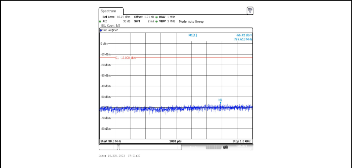
Band66-3MHz-QPSK-132322-1RB#0-Range3:30~1000MHz
