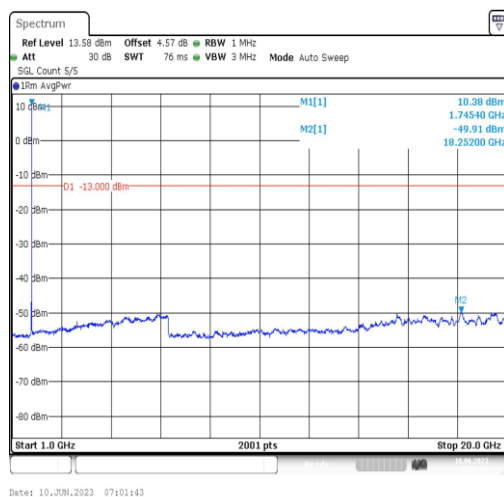
Band66-3MHz-QPSK-132322-1RB#0-Range4:1000~20000MHz
