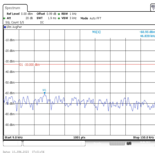
Band66-3MHz-16QAM-132322-1RB#0-Range1:0.009~0.15MHz
