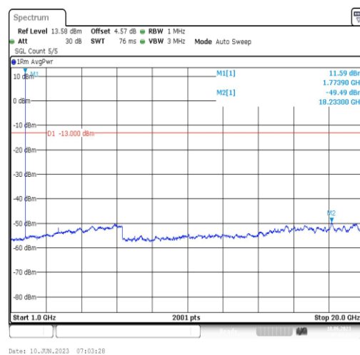
Band66-3MHz-QPSK-132657-1RB#0-Range4:1000~20000MHz
