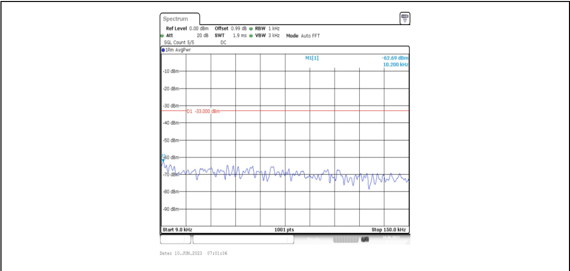
Band66-3MHz-QPSK-132322-1RB#0-Range1:0.009~0.15MHz
