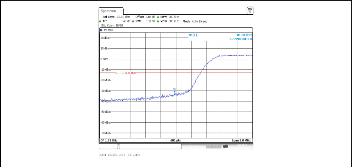
Band66-10MHz-16QAM-132022-50RB#0
