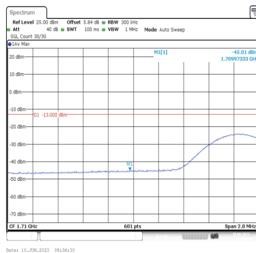
Band66-15MHz-QPSK-132047-1RB#74
