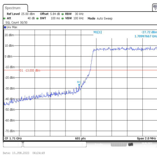
Band66-1.4MHz-QPSK-131979-6RB#0
