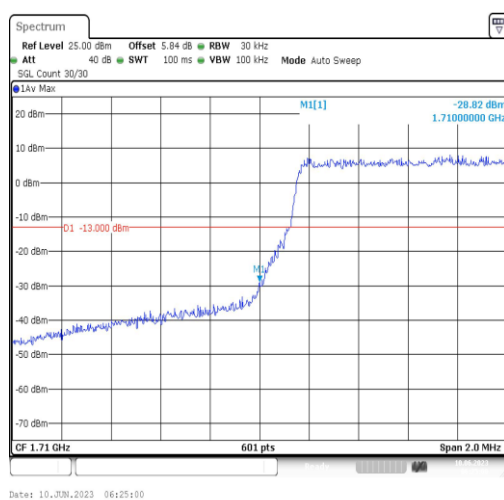
Band66-1.4MHz-16QAM-131979-6RB#0
