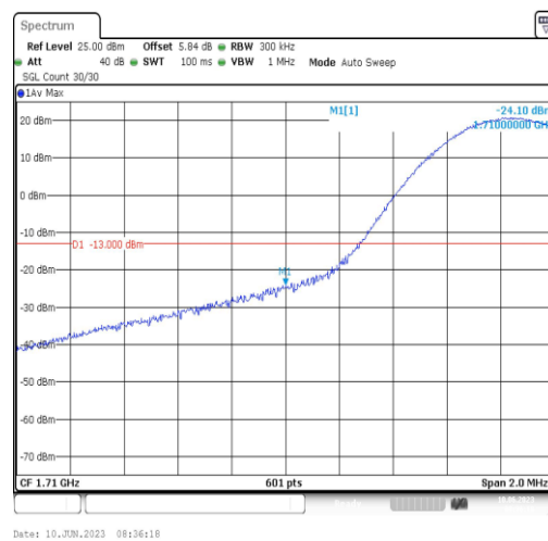
Band66-15MHz-16QAM-132047-1RB#0
