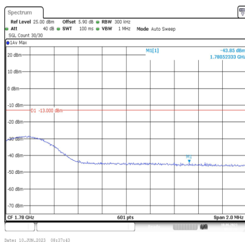
Band66-15MHz-16QAM-132597-1RB#0
