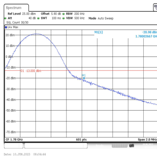
Band66-10MHz-QPSK-132622-1RB#49
