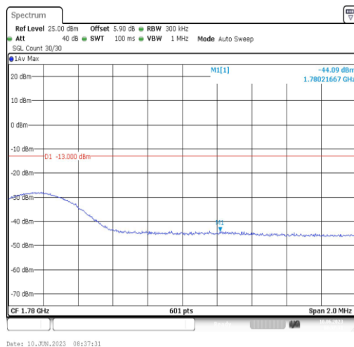
Band66-15MHz-QPSK-132597-1RB#0
