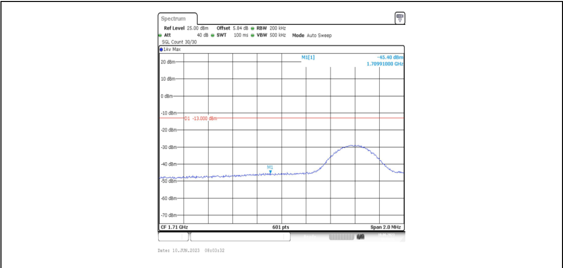
Band66-10MHz-16QAM-132022-1RB#49
