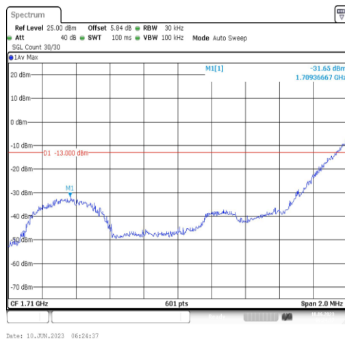
Band66-1.4MHz-16QAM-131979-1RB#5
