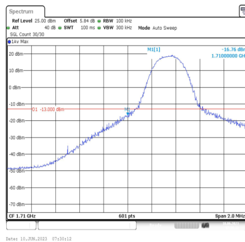
Band66-5MHz-16QAM-131997-1RB#0
