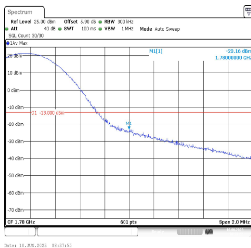
Band66-15MHz-QPSK-132597-1RB#74
