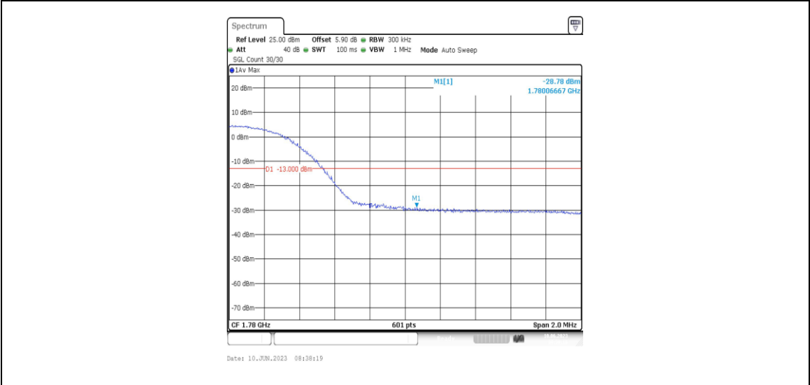
Band66-15MHz-QPSK-132597-75RB#0
