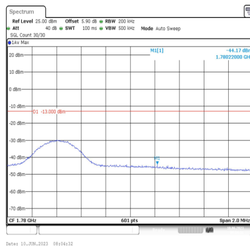
Band66-10MHz-16QAM-132622-1RB#0
