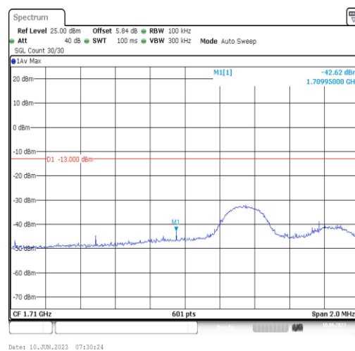
Band66-5MHz-QPSK-131997-1RB#24
