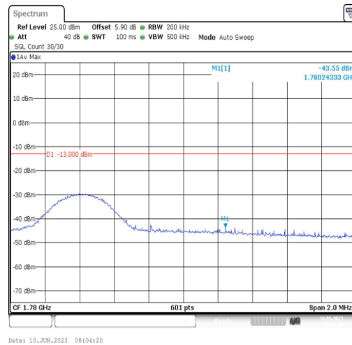
Band66-10MHz-QPSK-132622-1RB#0
