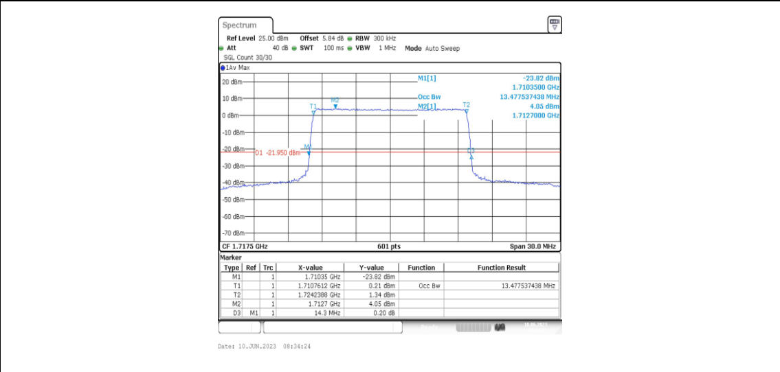
Band66-15MHz-16QAM-132047-75RB#0-13.478
