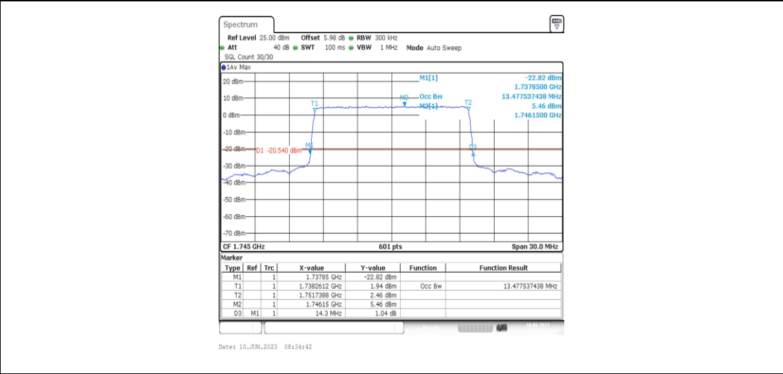
Band66-15MHz-QPSK-132322-75RB#0-13.478
