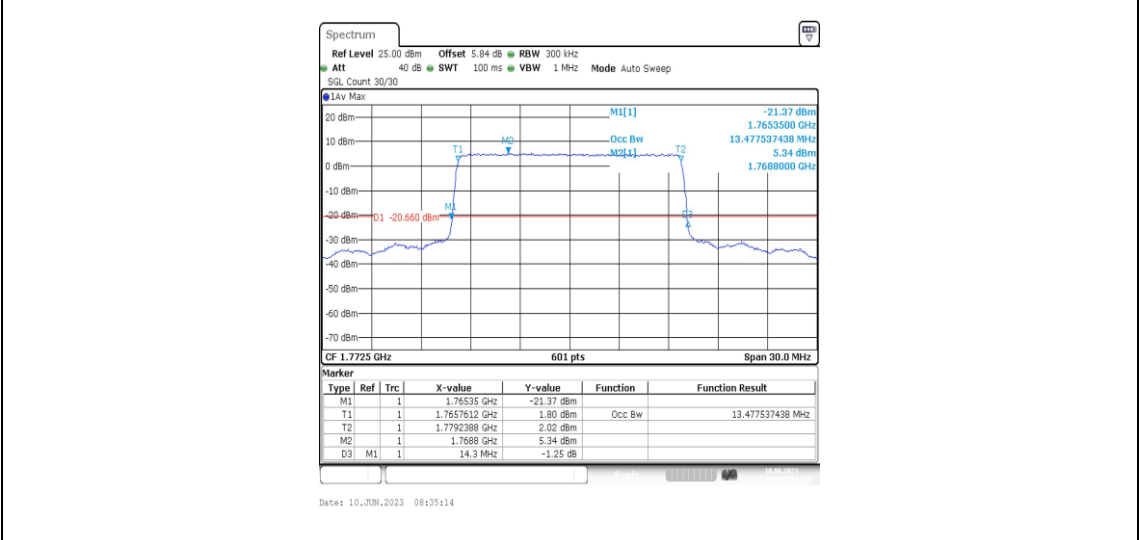
Band66-15MHz-QPSK-132597-75RB#0-13.478
