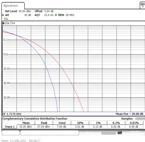
Band66-15MHz-16QAM-132047-75RB#0
