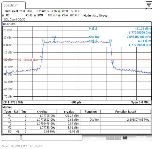
Band66-3MHz-16QAM-132657-15RB#0-2.696
