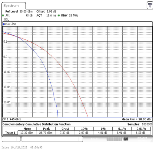
Band66-20MHz-16QAM-132322-100RB#0
