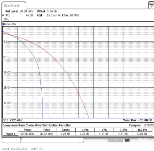
Band66-15MHz-QPSK-132597-1RB#0
