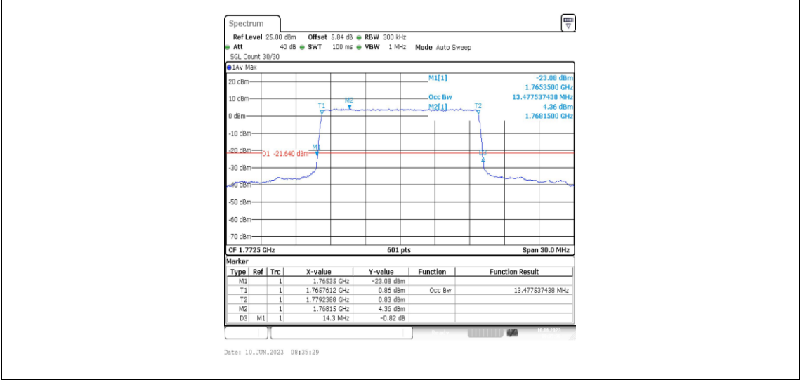
Band66-15MHz-16QAM-132597-75RB#0-13.478
