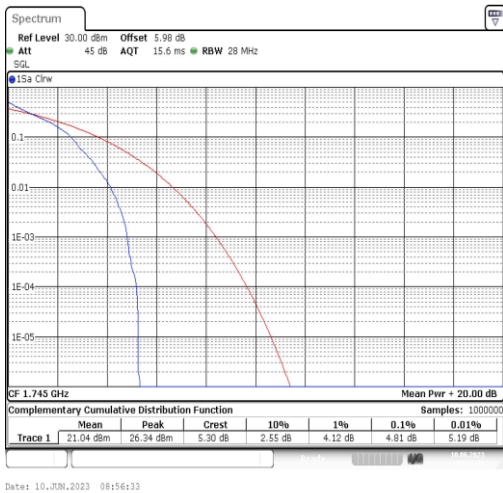
Band66-15MHz-QPSK-132322-1RB#0
