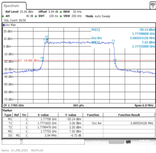
Band66-3MHz-QPSK-132657-15RB#0-2.686
