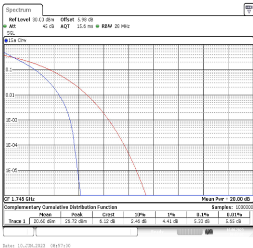
Band66-15MHz-QPSK-132322-75RB#0
