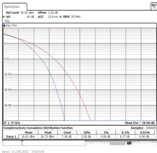
Band66-20MHz-16QAM-132072-100RB#0
