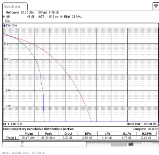
Band66-20MHz-QPSK-132322-1RB#0
