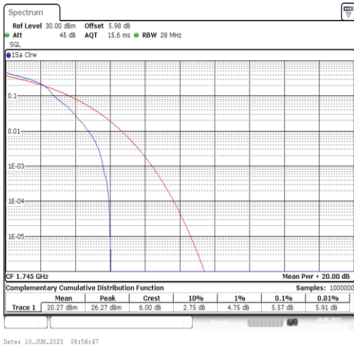
Band66-15MHz-16QAM-132322-1RB#0
