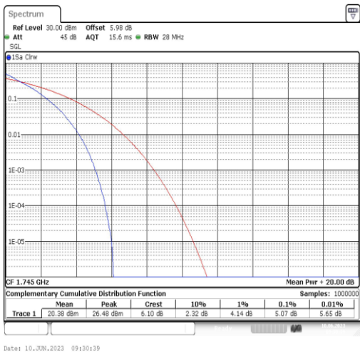
Band66-20MHz-QPSK-132322-100RB#0
