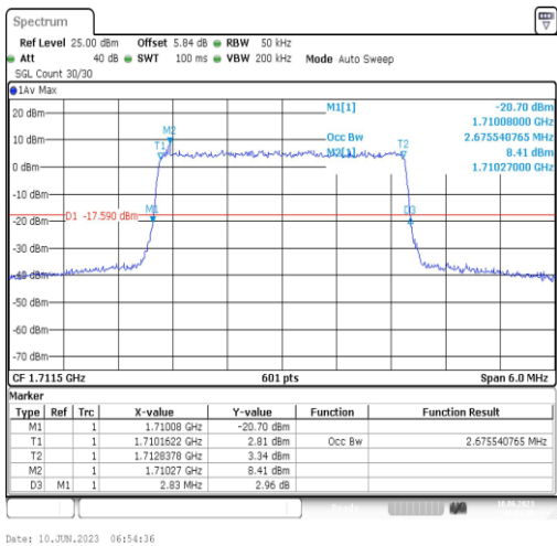
Band66-3MHz-QPSK-131987-15RB#0-2.676
