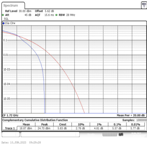
Band66-20MHz-16QAM-132072-1RB#0
