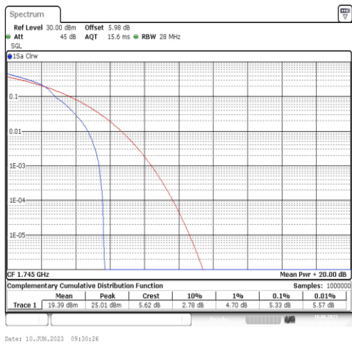
Band66-20MHz-16QAM-132322-1RB#0
