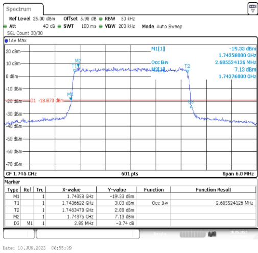
Band66-3MHz-QPSK-132322-15RB#0-2.686
