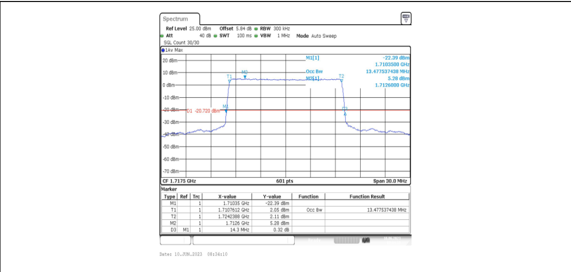
Band66-15MHz-QPSK-132047-75RB#0-13.478
