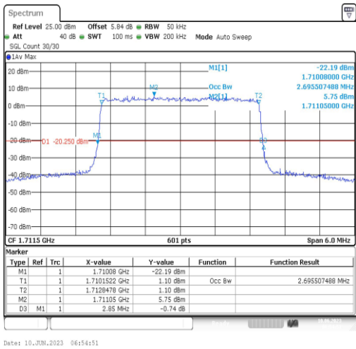
Band66-3MHz-16QAM-131987-15RB#0-2.696
