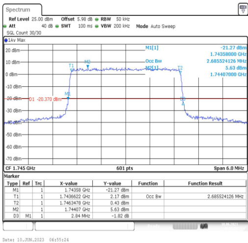
Band66-3MHz-16QAM-132322-15RB#0-2.686
