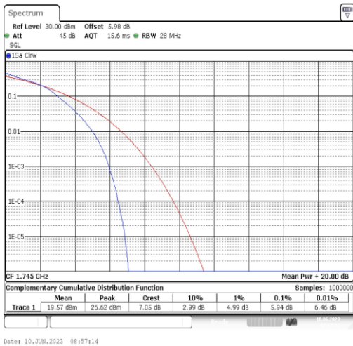
Band66-15MHz-16QAM-132322-75RB#0
