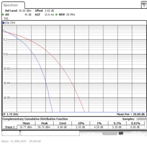
Band66-20MHz-QPSK-132072-100RB#0
