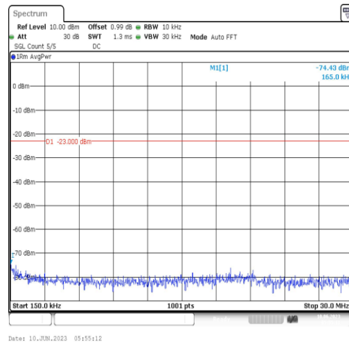
Band12-10MHz-16QAM-23060-1RB#0-Range2:0.15~30MHz
