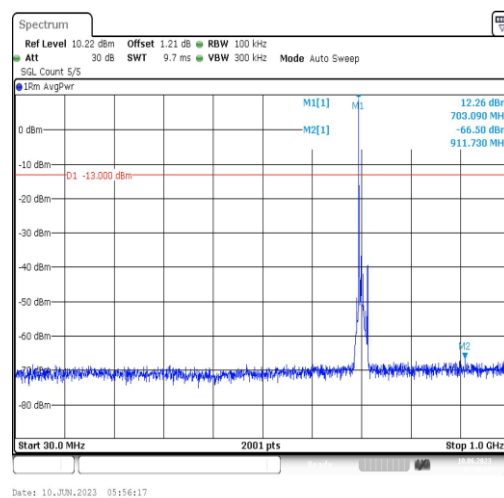
Band12-10MHz-QPSK-23095-1RB#0-Range3:30~1000MHz
