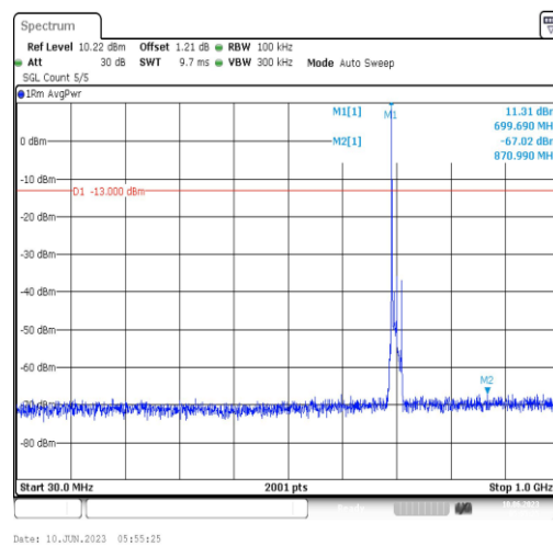
Band12-10MHz-16QAM-23060-1RB#0-Range3:30~1000MHz
