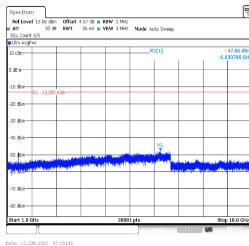
Band12-10MHz-16QAM-23060-1RB#0-Range4:1000~10000MHz
