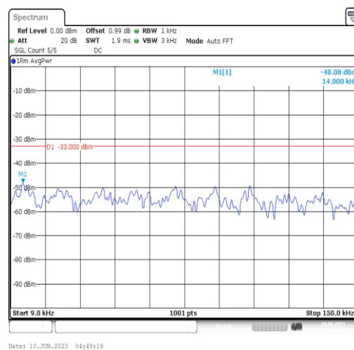
Band12-3MHz-16QAM-23025-1RB#0-Range1:0.009~0.15MHz
