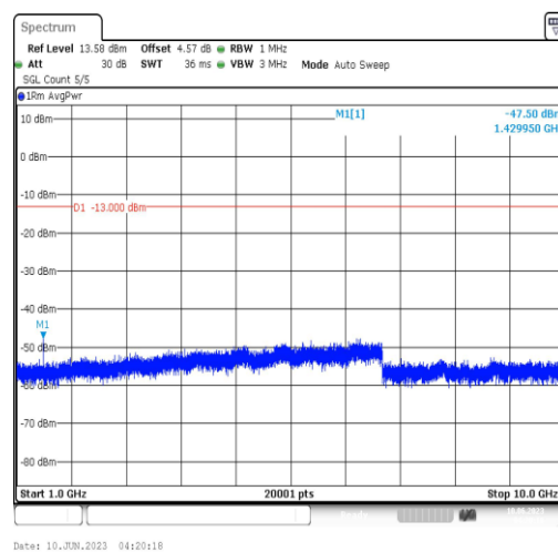
Band12-1.4MHz-QPSK-23173-1RB#0-Range4:1000~10000MHz
