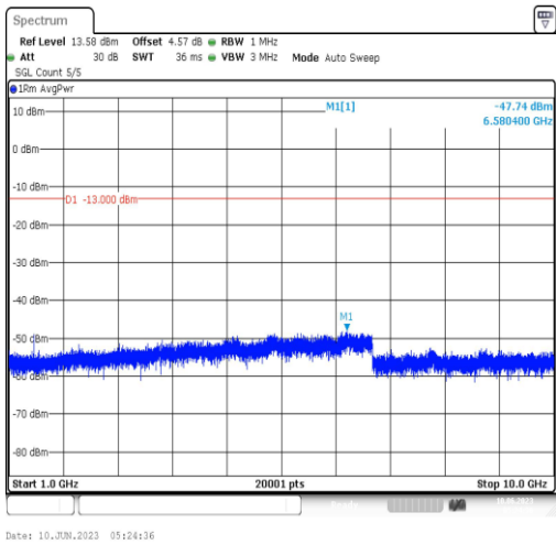
Band12-5MHz-16QAM-23095-1RB#0-Range4:1000~10000MHz
