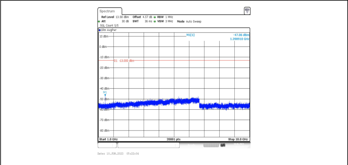
Band12-5MHz-QPSK-23035-1RB#0-Range4:1000~10000MHz
