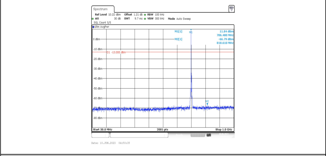
Band12-3MHz-QPSK-23095-1RB#0-Range3:30~1000MHz
