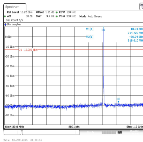
Band12-1.4MHz-QPSK-23173-1RB#0-Range3:30~1000MHz
