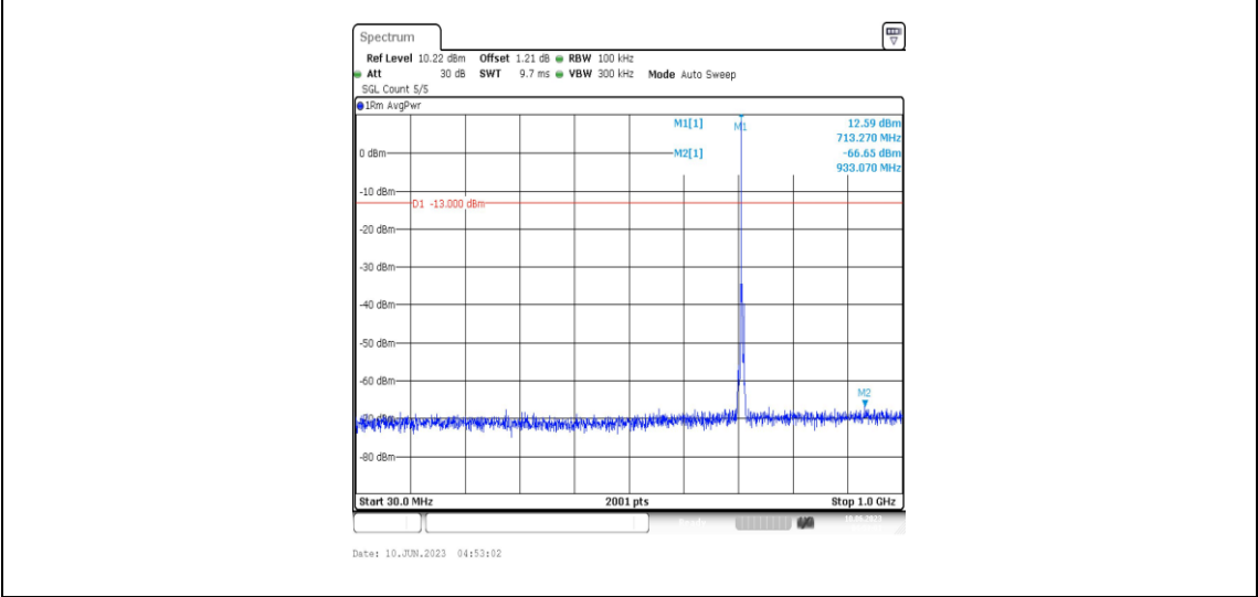
Band12-3MHz-16QAM-23165-1RB#0-Range3:30~1000MHz
