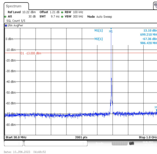
Band12-3MHz-QPSK-23025-1RB#0-Range3:30~1000MHz
