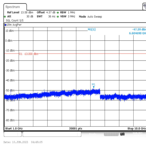
Band12-3MHz-QPSK-23025-1RB#0-Range4:1000~10000MHz
