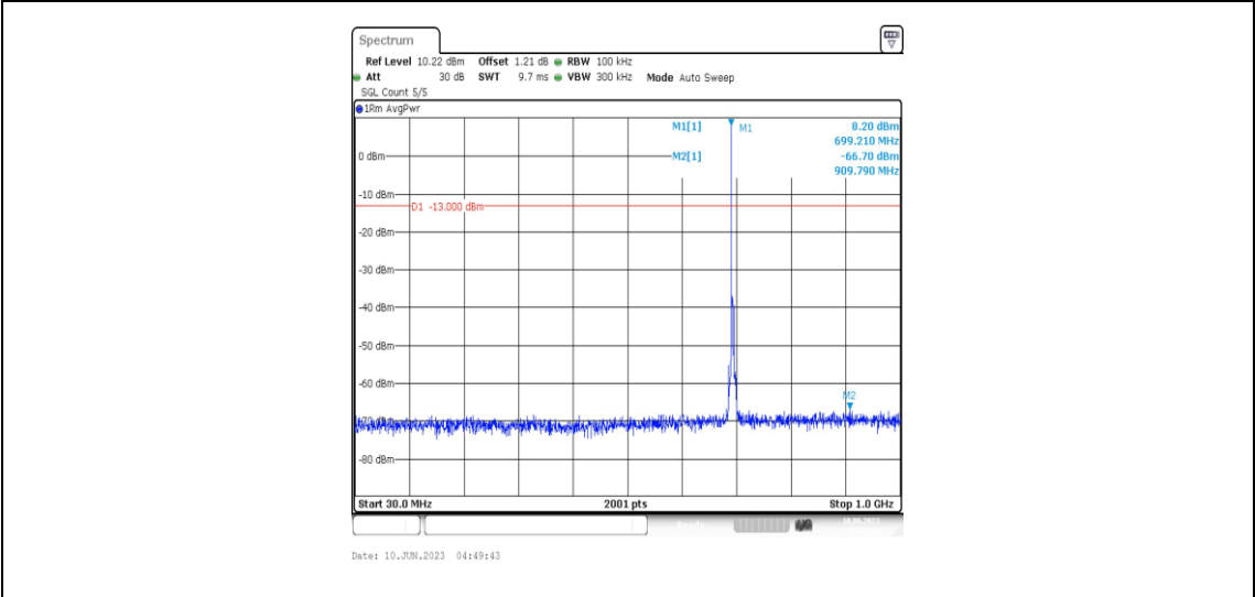
Band12-3MHz-16QAM-23025-1RB#0-Range3:30~1000MHz
