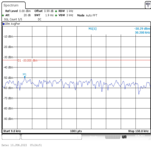
Band12-5MHz-QPSK-23155-1RB#0-Range1:0.009~0.15MHz
