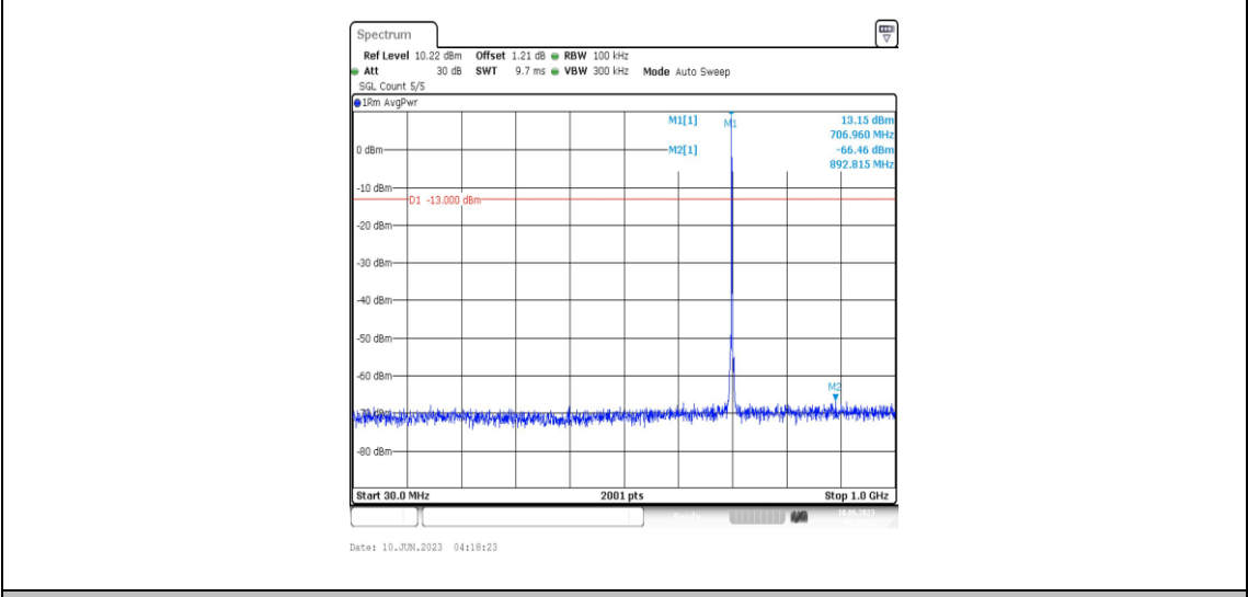
Band12-1.4MHz-QPSK-23095-1RB#0-Range3:30~1000MHz
