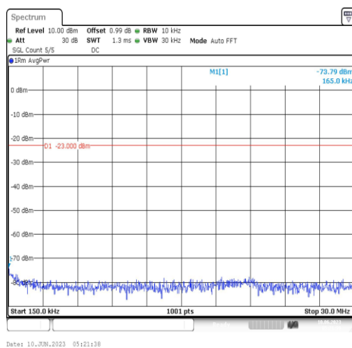
Band12-5MHz-QPSK-23035-1RB#0-Range2:0.15~30MHz
