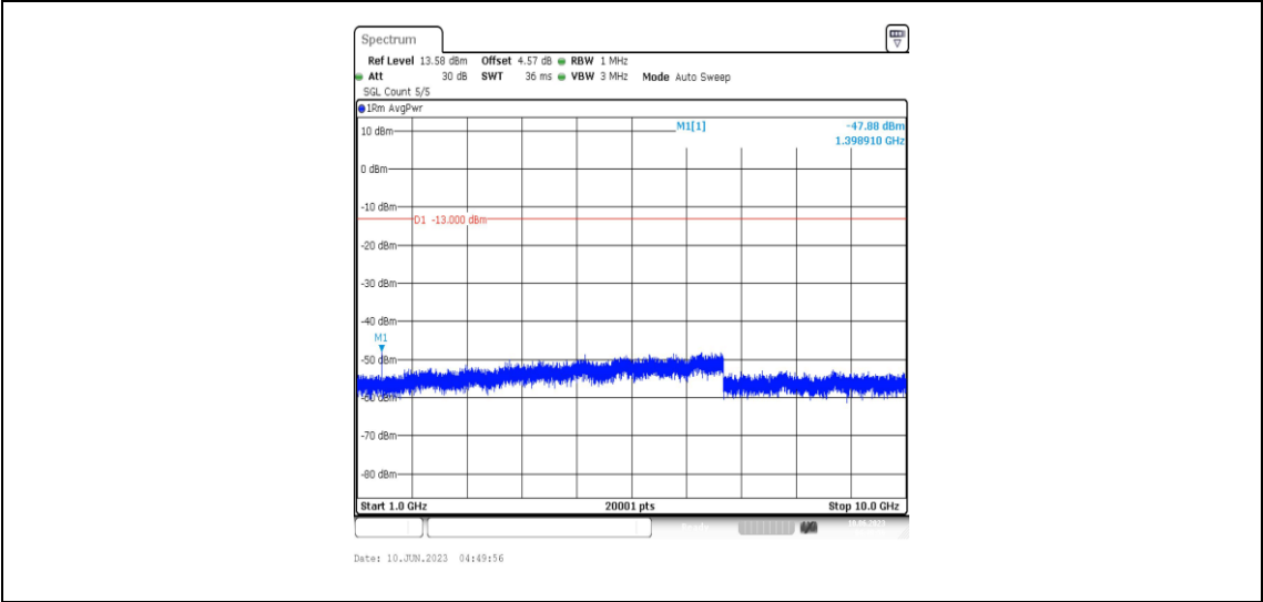
Band12-3MHz-16QAM-23025-1RB#0-Range4:1000~10000MHz
