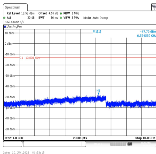
Band12-3MHz-16QAM-23165-1RB#0-Range4:1000~10000MHz
