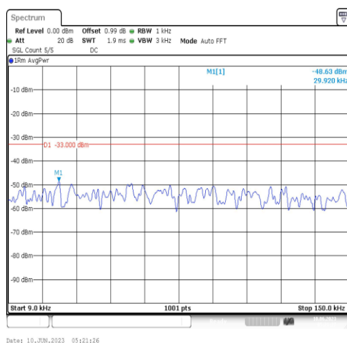
Band12-5MHz-QPSK-23035-1RB#0-Range1:0.009~0.15MHz
