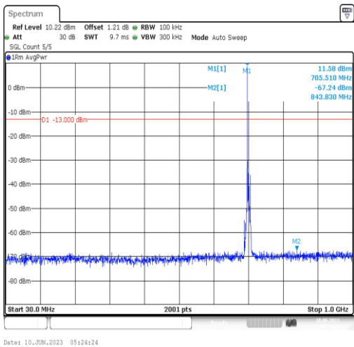
Band12-5MHz-16QAM-23095-1RB#0-Range3:30~1000MHz
