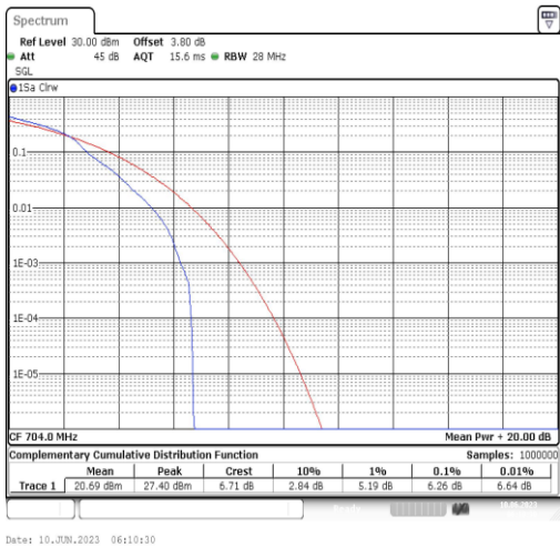
Band12-10MHz-16QAM-23060-1RB#0
