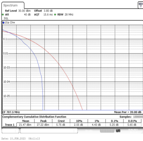
Band12-10MHz-QPSK-23095-1RB#0
