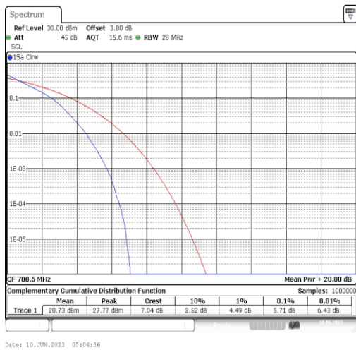
Band12-3MHz-QPSK-23025-15RB#0
