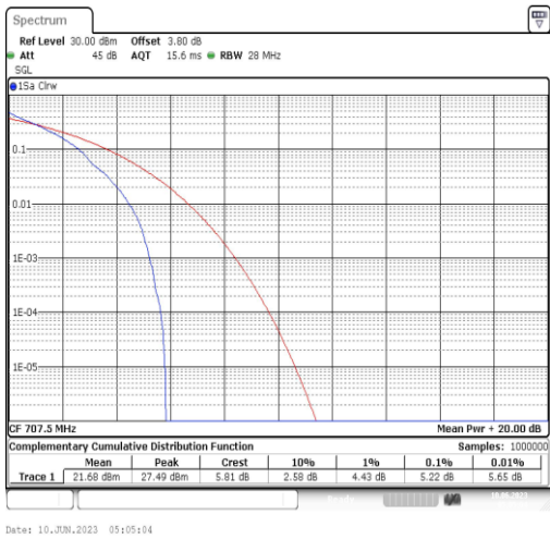
Band12-3MHz-QPSK-23095-1RB#0
