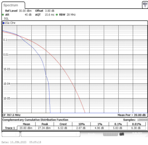
Band12-3MHz-16QAM-23095-1RB#0
