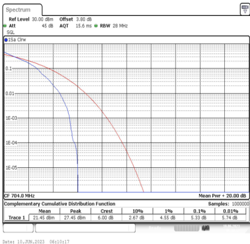
Band12-10MHz-QPSK-23060-1RB#0
