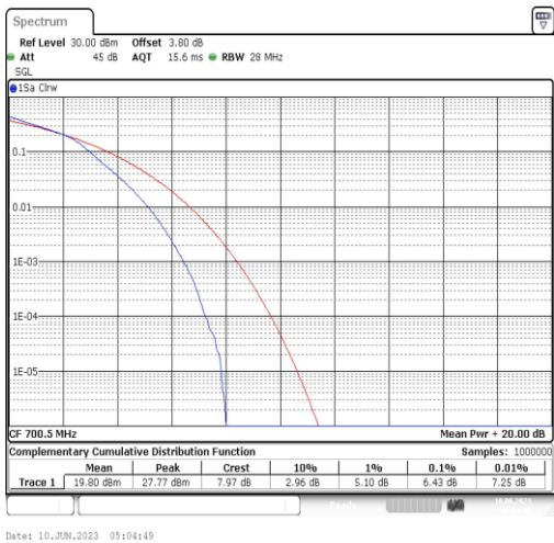
Band12-3MHz-16QAM-23025-15RB#0
