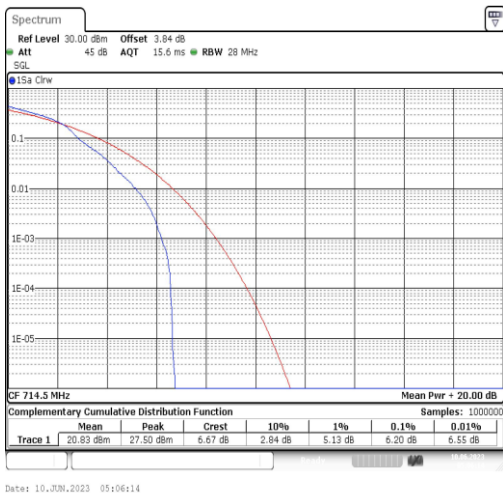
Band12-3MHz-16QAM-23165-1RB#0
