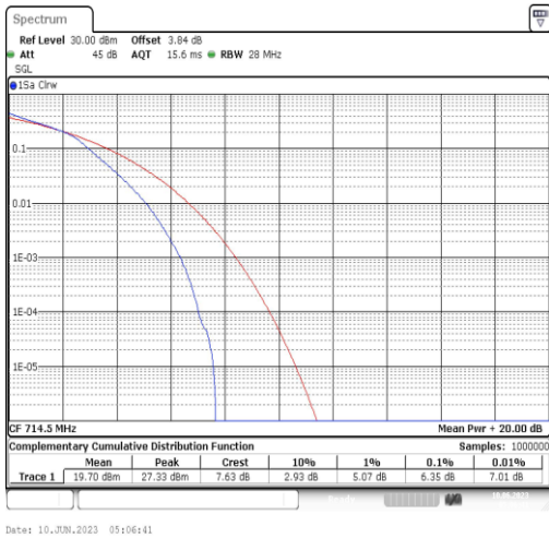
Band12-3MHz-16QAM-23165-15RB#0
