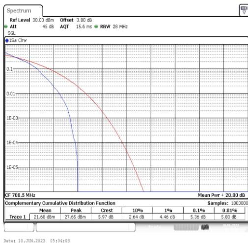
Band12-3MHz-QPSK-23025-1RB#0
