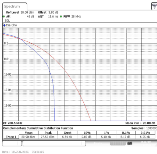
Band12-3MHz-16QAM-23025-1RB#0
