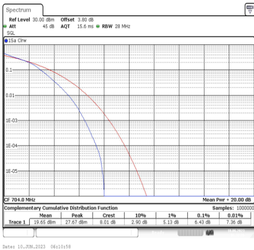
Band12-10MHz-16QAM-23060-50RB#0
