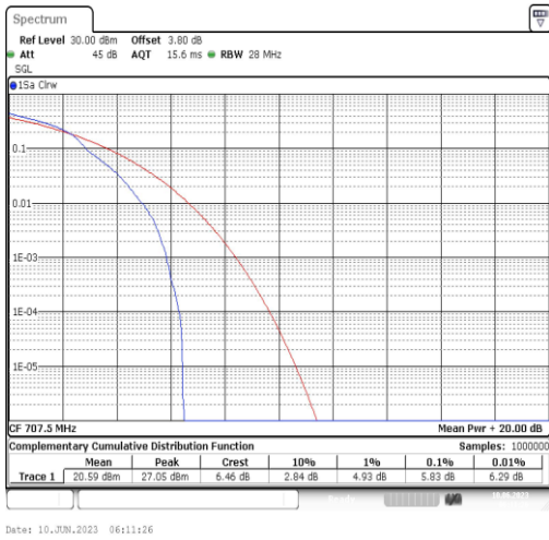
Band12-10MHz-16QAM-23095-1RB#0
