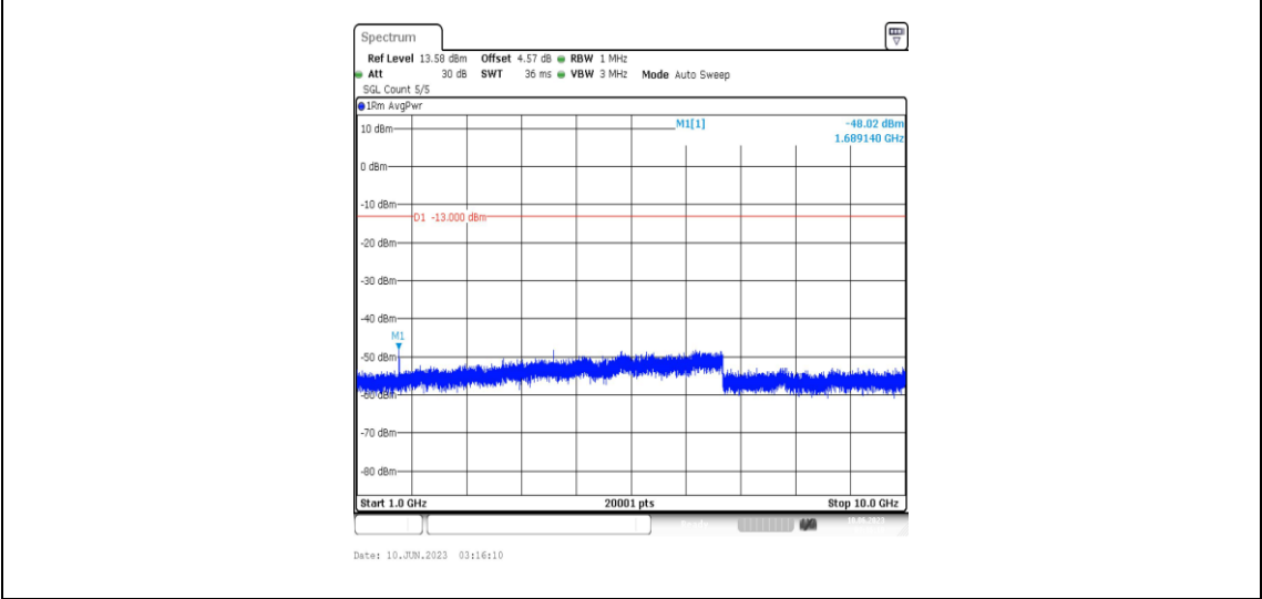
Band5-5MHz-16QAM-20625-1RB#0-Range4:1000~10000MHz
