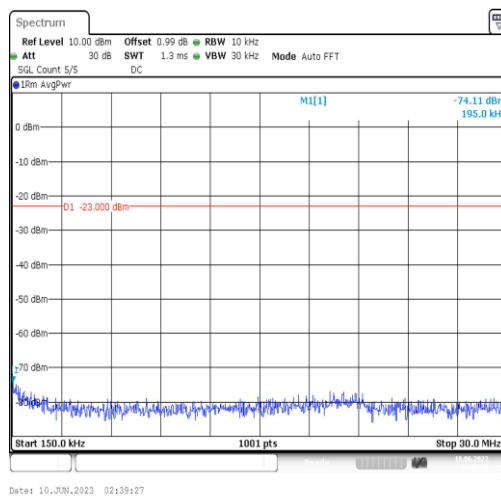
Band5-3MHz-16QAM-20415-1RB#0-Range2:0.15~30MHz
