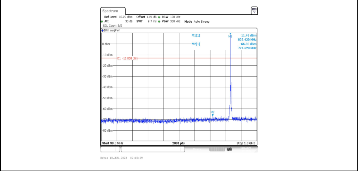
Band5-3MHz-QPSK-20525-1RB#0-Range3:30~1000MHz
