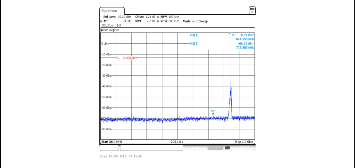
Band5-5MHz-16QAM-20625-1RB#0-Range3:30~1000MHz
