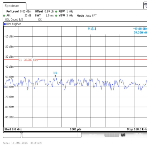
Band5-5MHz-QPSK-20425-1RB#0-Range1:0.009~0.15MHz
