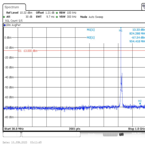
Band5-5MHz-QPSK-20425-1RB#0-Range3:30~1000MHz
