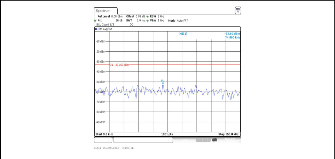
Band5-1.4MHz-QPSK-20643-1RB#0-Range1:0.009~0.15MHz
