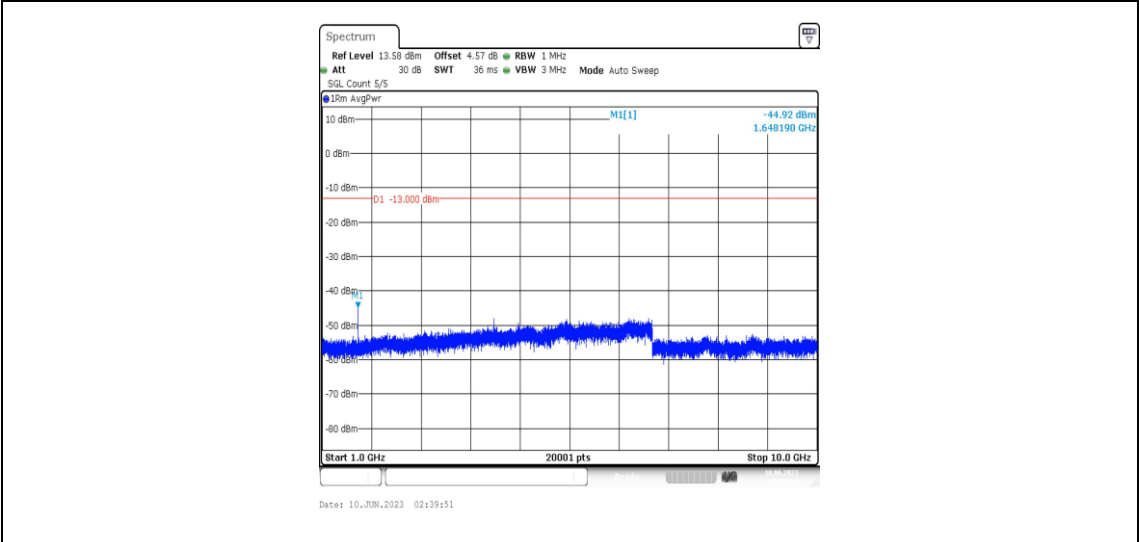
Band5-3MHz-16QAM-20415-1RB#0-Range4:1000~10000MHz
