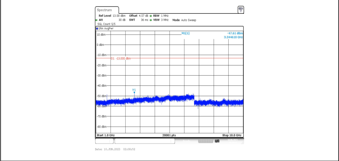
Band5-1.4MHz-QPSK-20525-1RB#0-Range4:1000~10000MHz
