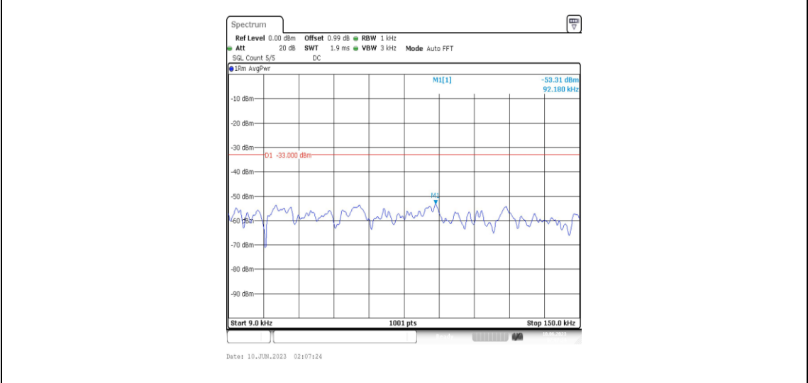
Band5-1.4MHz-16QAM-20407-1RB#0-Range1:0.009~0.15MHz
