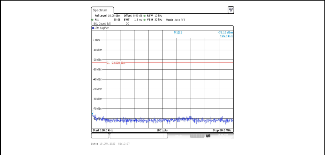
Band5-1.4MHz-QPSK-20643-1RB#0-Range2:0.15~30MHz
