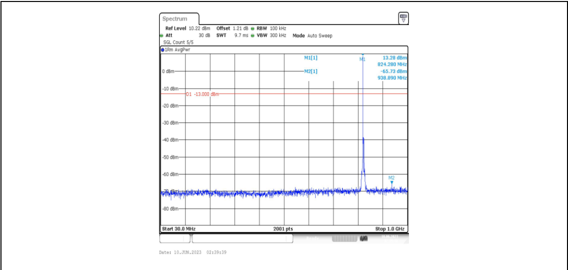
Band5-3MHz-16QAM-20415-1RB#0-Range3:30~1000MHz
