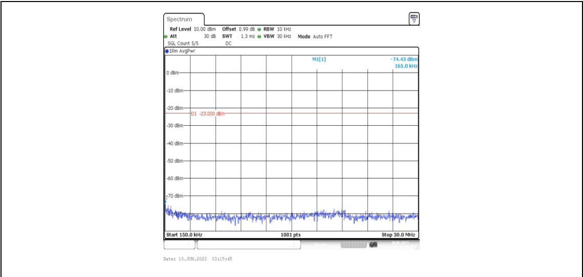
Band5-5MHz-16QAM-20625-1RB#0-Range2:0.15~30MHz
