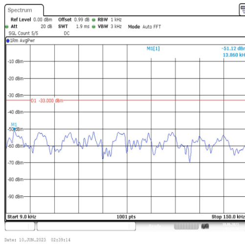
Band5-3MHz-16QAM-20415-1RB#0-Range1:0.009~0.15MHz
