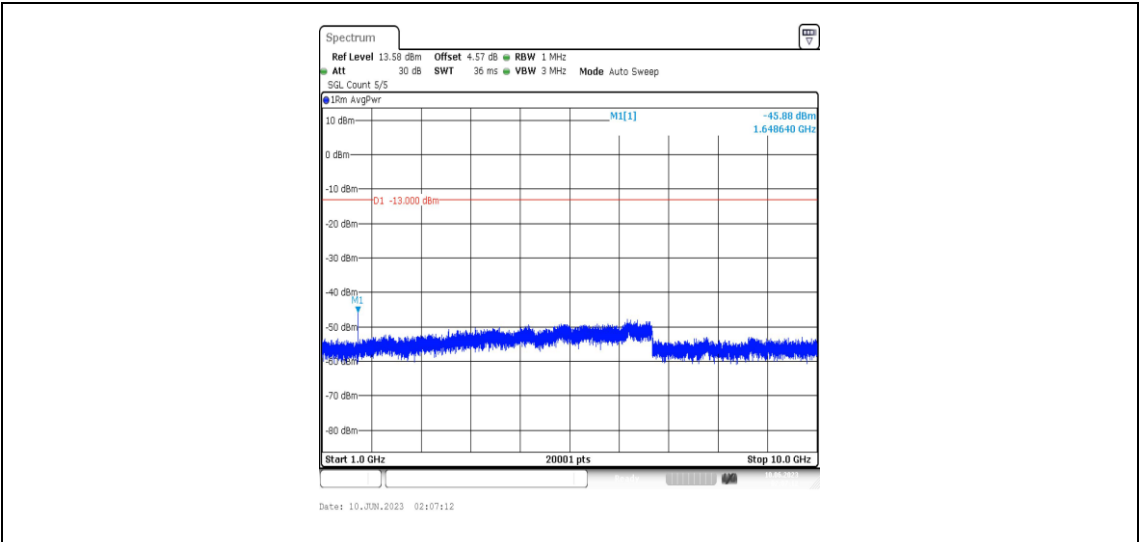
Band5-1.4MHz-QPSK-20407-1RB#0-Range4:1000~10000MHz
