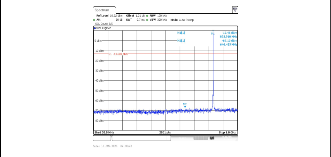
Band5-1.4MHz-QPSK-20525-1RB#0-Range3:30~1000MHz
