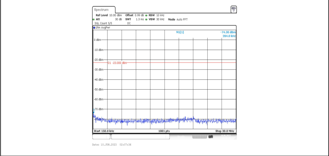
Band5-1.4MHz-16QAM-20407-1RB#0-Range2:0.15~30MHz
