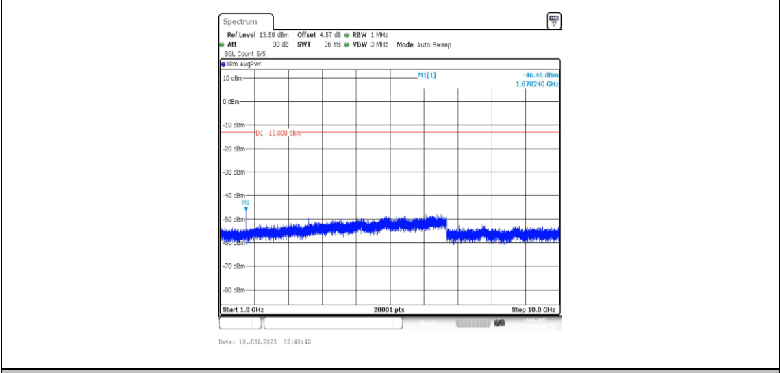
Band5-3MHz-QPSK-20525-1RB#0-Range4:1000~10000MHz
