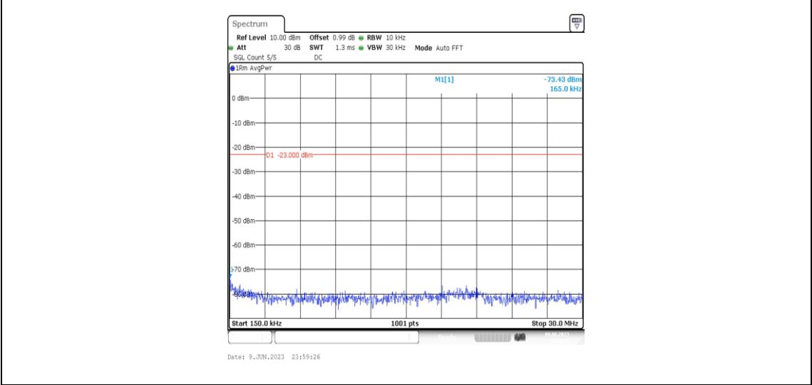
Band4-5MHz-16QAM-20175-1RB#0-Range2:0.15~30MHz
