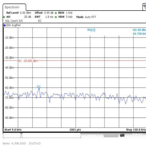
Band4-3MHz-QPSK-20385-1RB#0-Range1:0.009~0.15MHz
