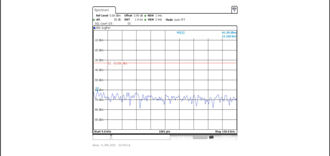
Band4-5MHz-16QAM-20175-1RB#0-Range1:0.009~0.15MHz
