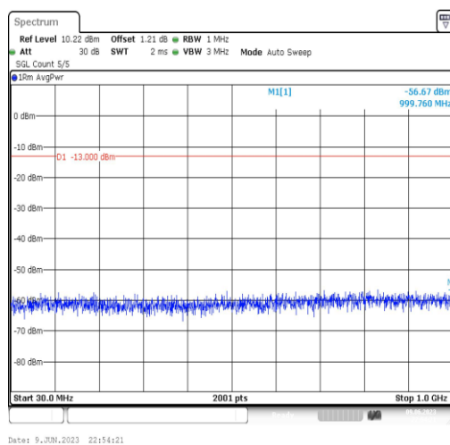
Band4-1.4MHz-QPSK-20175-1RB#0-Range3:30~1000MHz
