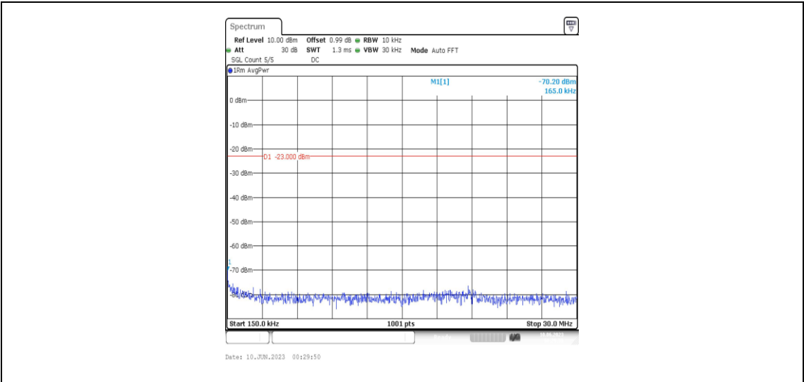
Band4-10MHz-16QAM-20000-1RB#0-Range2:0.15~30MHz
