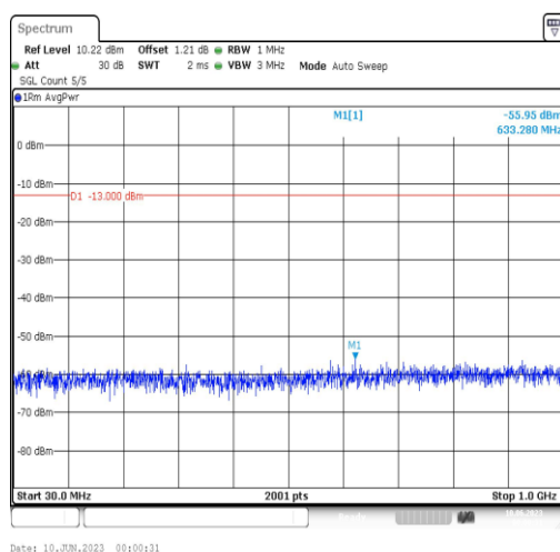
Band4-5MHz-QPSK-20375-1RB#0-Range3:30~1000MHz
