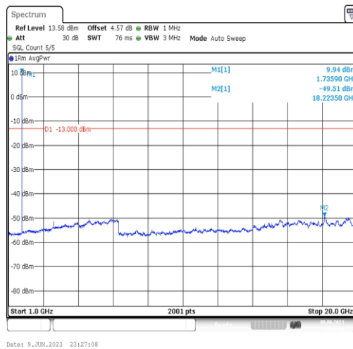
Band4-3MHz-16QAM-20175-1RB#0-Range4:1000~20000MHz
