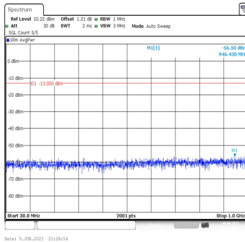
Band4-3MHz-16QAM-20175-1RB#0-Range3:30~1000MHz
