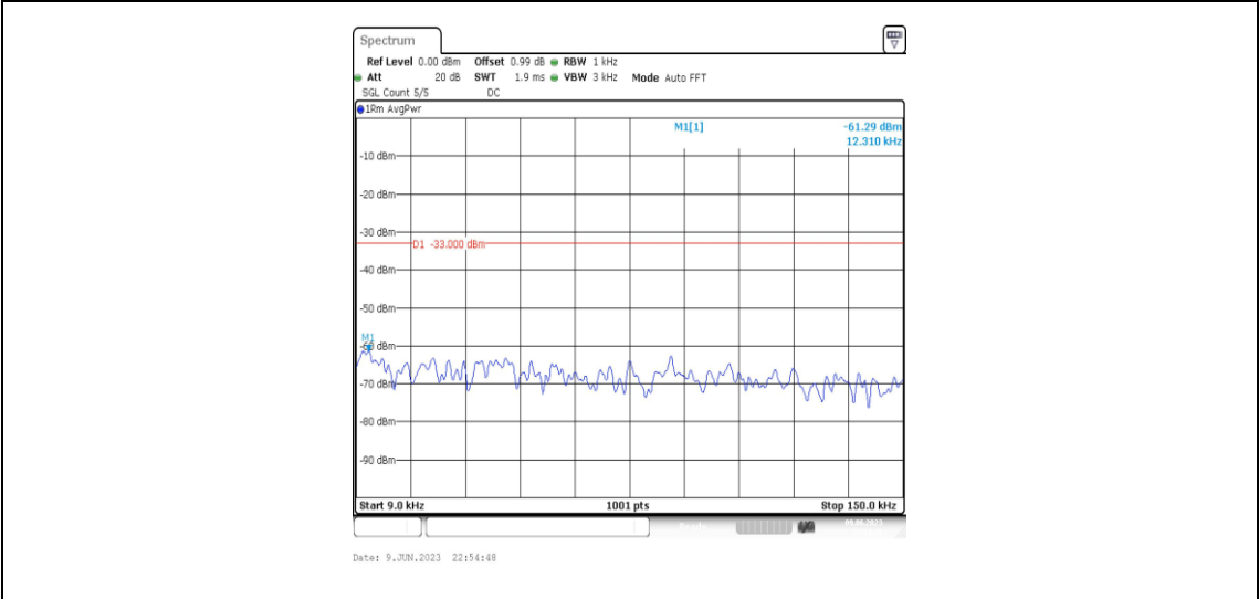
Band4-1.4MHz-16QAM-20175-1RB#0-Range1:0.009~0.15MHz
