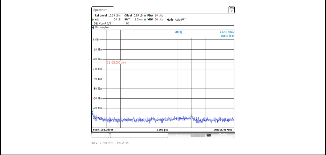
Band4-1.4MHz-16QAM-20393-1RB#0-Range2:0.15~30MHz
