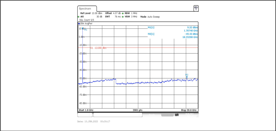
Band4-10MHz-16QAM-20000-1RB#0-Range4:1000~20000MHz
