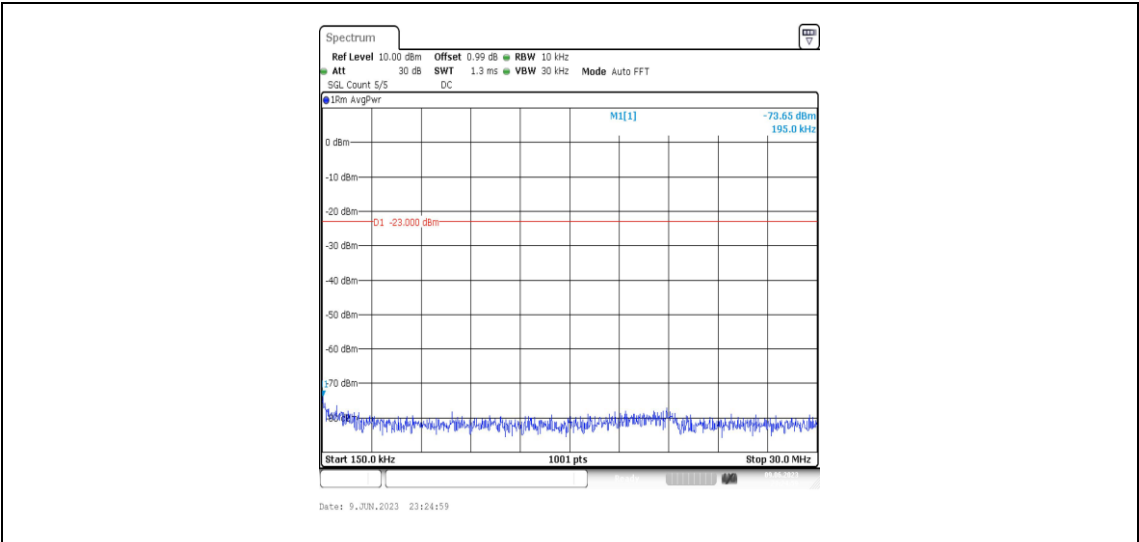
Band4-3MHz-16QAM-19965-1RB#0-Range2:0.15~30MHz
