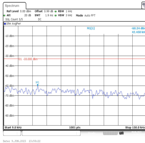
Band4-5MHz-QPSK-20175-1RB#0-Range1:0.009~0.15MHz
