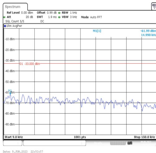
Band4-1.4MHz-QPSK-20175-1RB#0-Range1:0.009~0.15MHz
