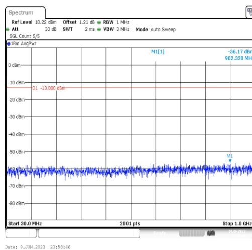
Band4-5MHz-QPSK-20175-1RB#0-Range3:30~1000MHz
