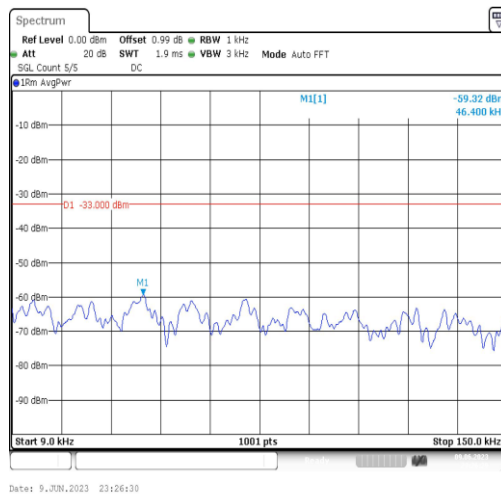
Band4-3MHz-16QAM-20175-1RB#0-Range1:0.009~0.15MHz
