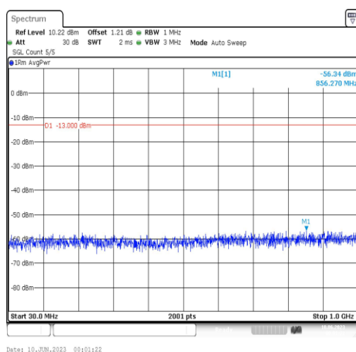
Band4-5MHz-16QAM-20375-1RB#0-Range3:30~1000MHz
