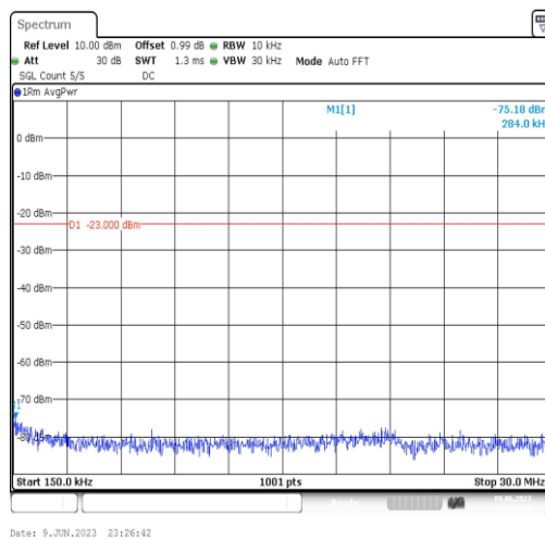
Band4-3MHz-16QAM-20175-1RB#0-Range2:0.15~30MHz
