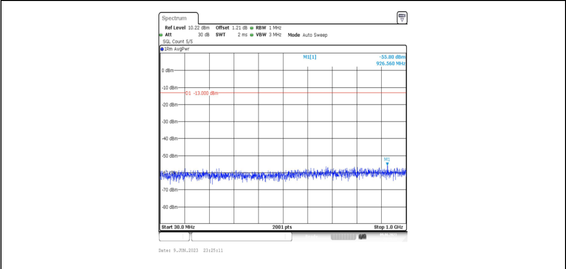
Band4-3MHz-16QAM-19965-1RB#0-Range3:30~1000MHz
