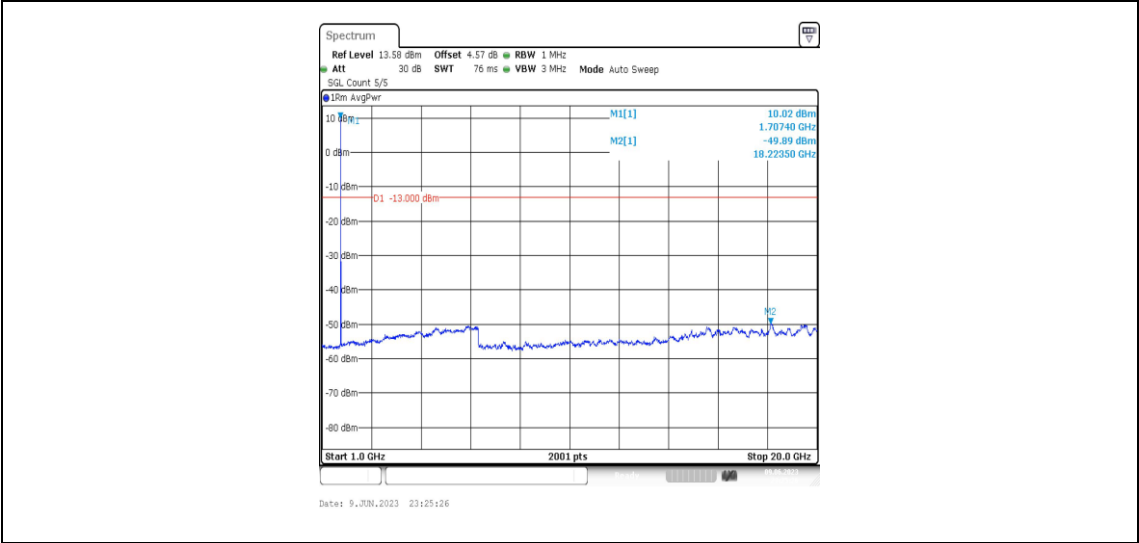
Band4-3MHz-16QAM-19965-1RB#0-Range4:1000~20000MHz
