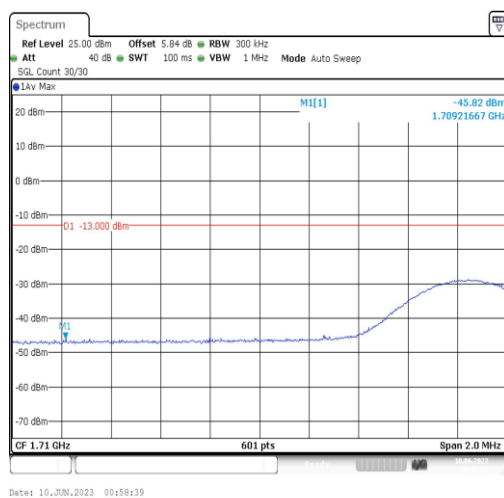
Band4-15MHz-QPSK-20025-1RB#74
