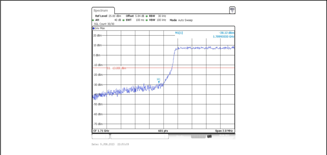
Band4-1.4MHz-QPSK-19957-6RB#0
