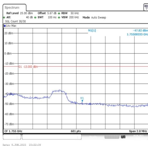
Band4-3MHz-16QAM-20385-1RB#0
