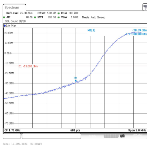
Band4-15MHz-16QAM-20025-1RB#0
