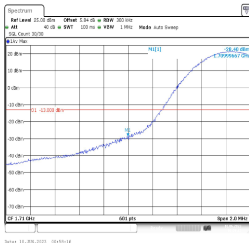
Band4-15MHz-QPSK-20025-1RB#0
