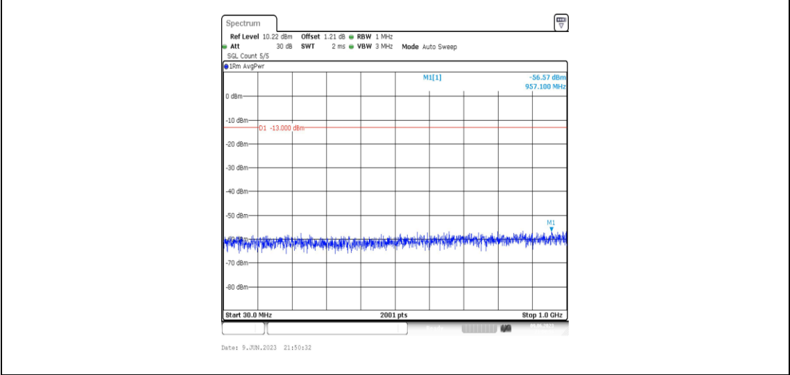
Band2-15MHz-16QAM-18900-1RB#0-Range3:30~1000MHz
