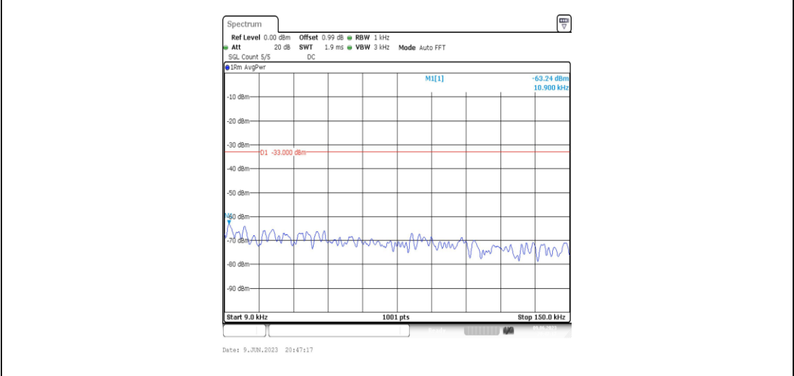
Band2-5MHz-QPSK-19175-1RB#0-Range1:0.009~0.15MHz
