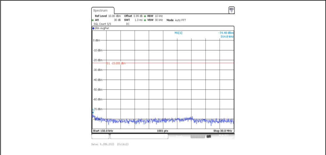
Band2-3MHz-16QAM-18900-1RB#0-Range2:0.15~30MHz
