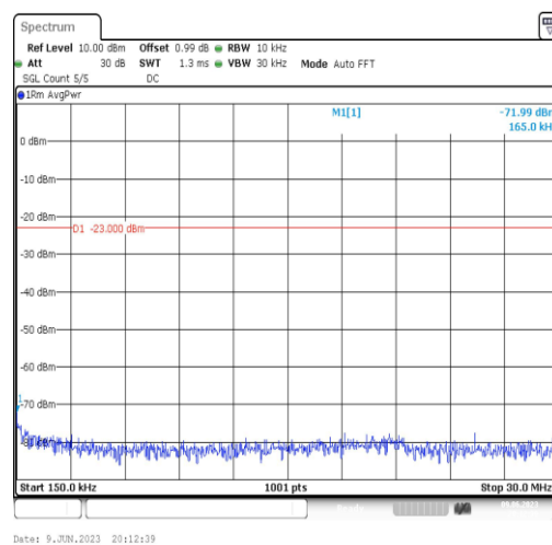
Band2-3MHz-16QAM-18615-1RB#0-Range2:0.15~30MHz
