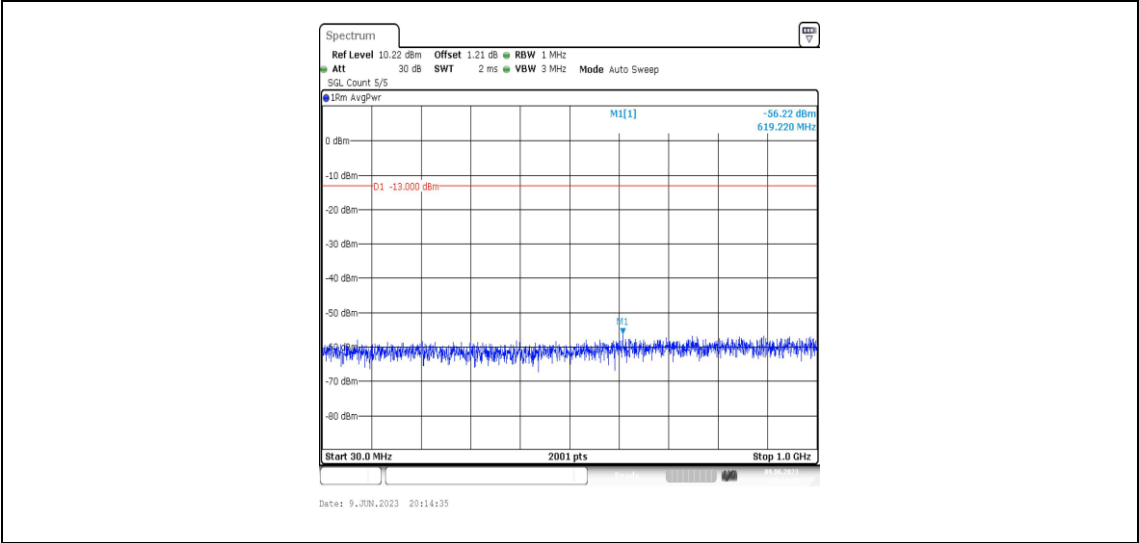
Band2-3MHz-16QAM-18900-1RB#0-Range3:30~1000MHz
