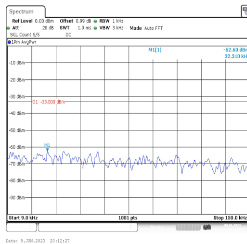
Band2-3MHz-16QAM-18615-1RB#0-Range1:0.009~0.15MHz
