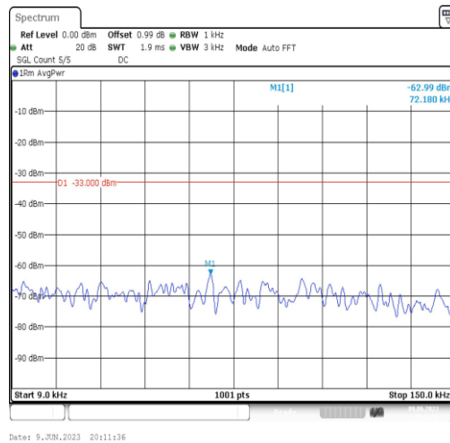
Band2-3MHz-QPSK-18615-1RB#0-Range1:0.009~0.15MHz
