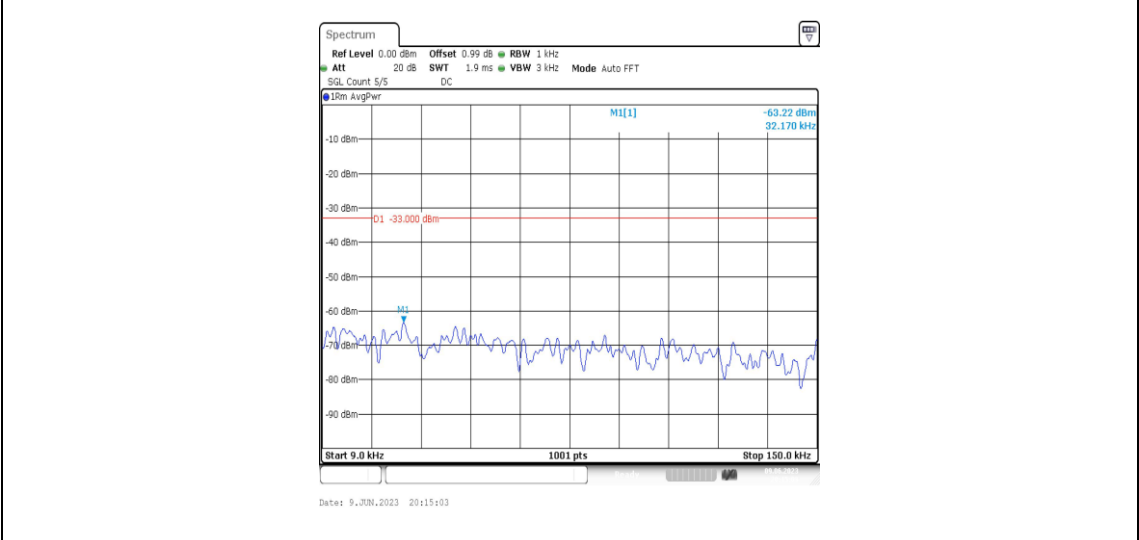
Band2-3MHz-QPSK-19185-1RB#0-Range1:0.009~0.15MHz
