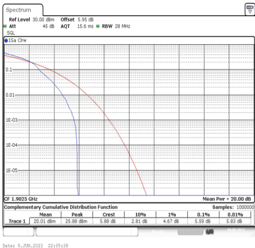
Band2-15MHz-16QAM-19125-1RB#0
