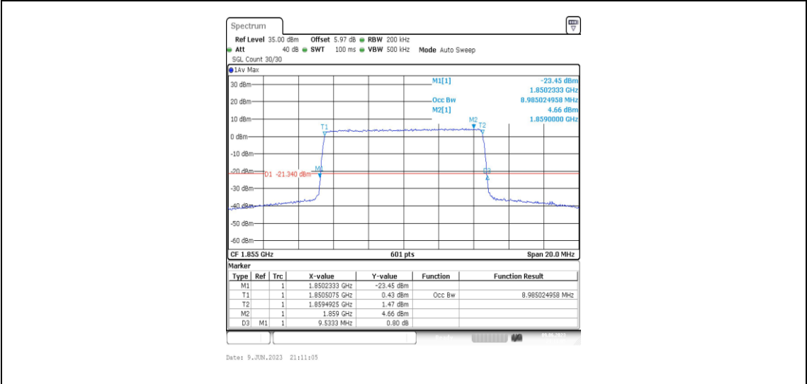
Band2-10MHz-16QAM-18650-50RB#0-8.985
