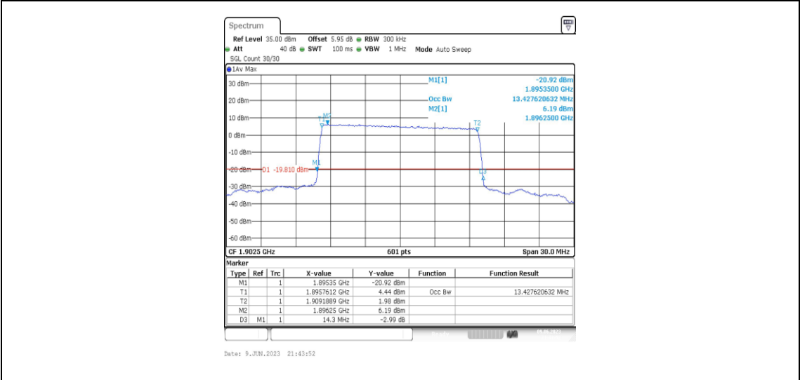
Band2-15MHz-QPSK-19125-75RB#0-13.428
