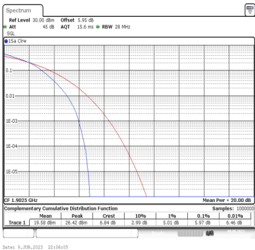
Band2-15MHz-16QAM-19125-75RB#0
