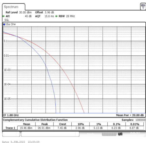
Band2-15MHz-16QAM-18900-75RB#0
