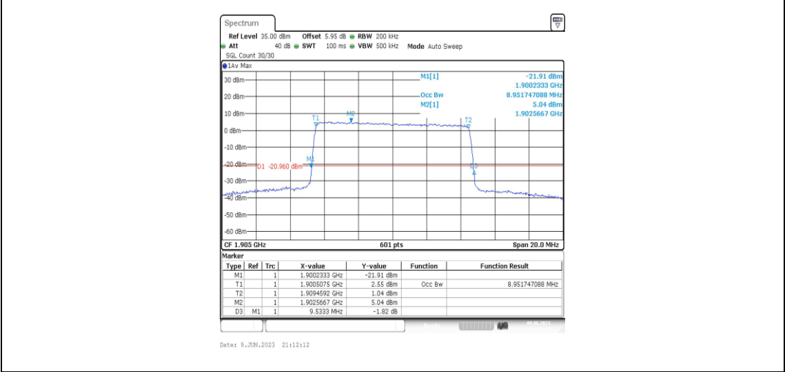
Band2-10MHz-16QAM-19150-50RB#0-8.952
