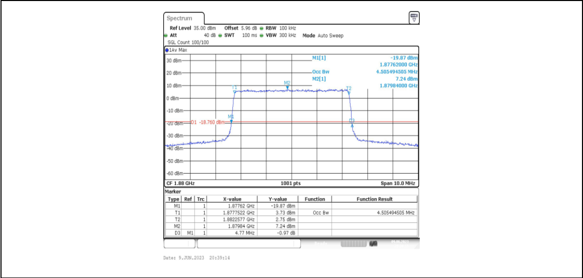
Band2-5MHz-QPSK-18900-25RB#0-4.505
