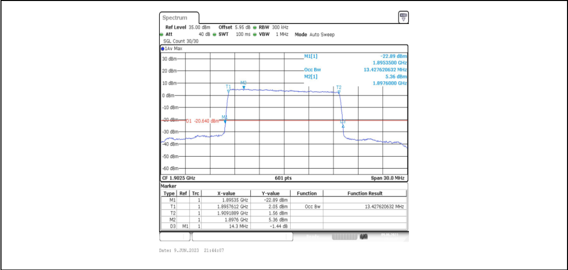
Band2-15MHz-16QAM-19125-75RB#0-13.428
