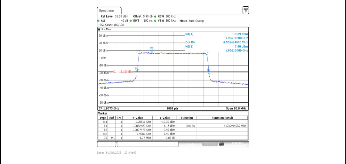
Band2-5MHz-QPSK-19175-25RB#0-4.505
