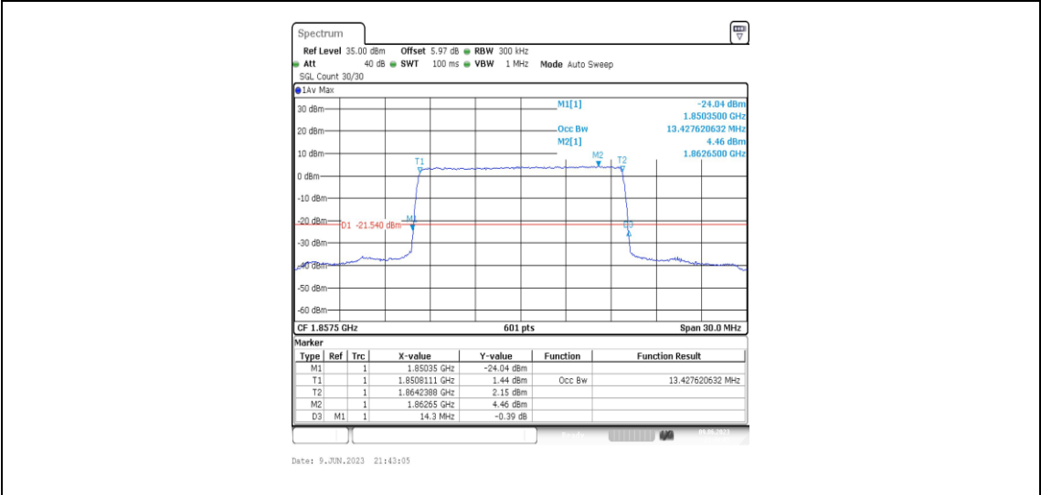
Band2-15MHz-16QAM-18675-75RB#0-13.428
