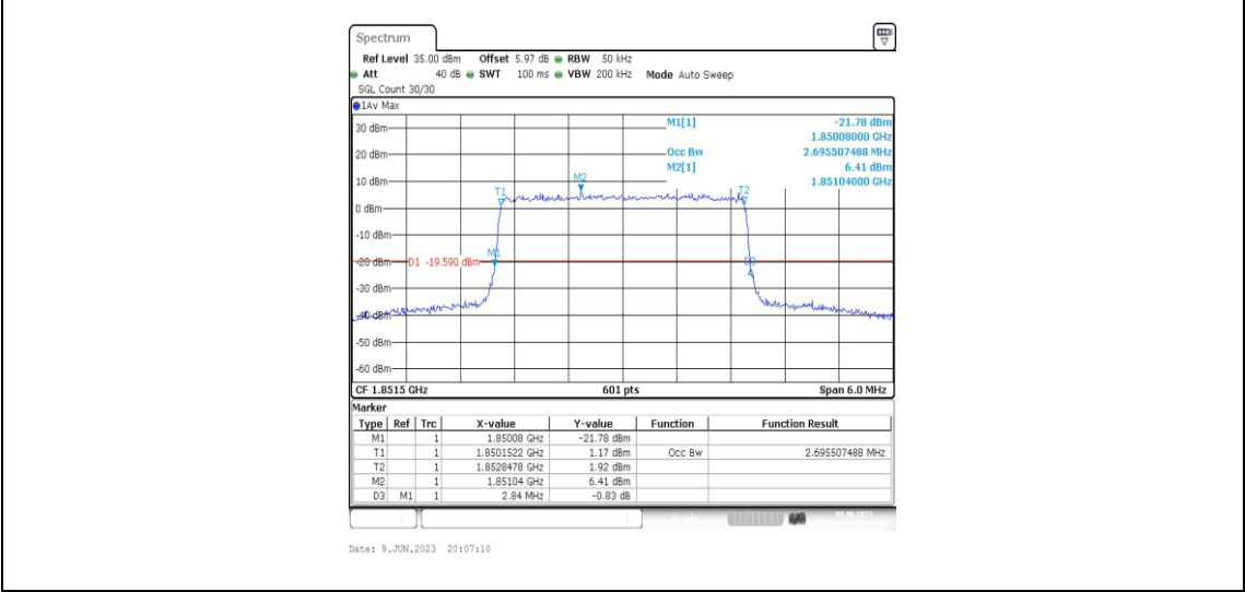
Band2-3MHz-16QAM-18615-15RB#0-2.696
