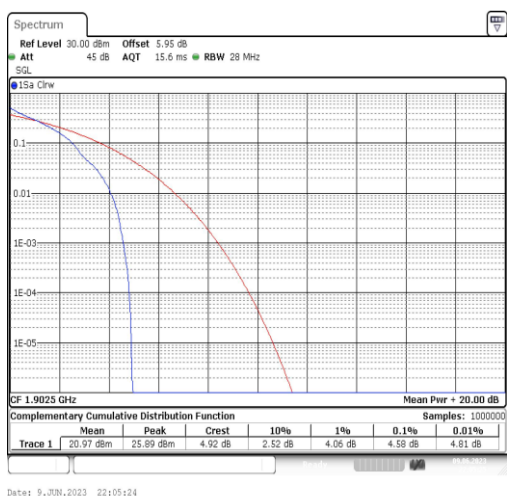
Band2-15MHz-QPSK-19125-1RB#0
