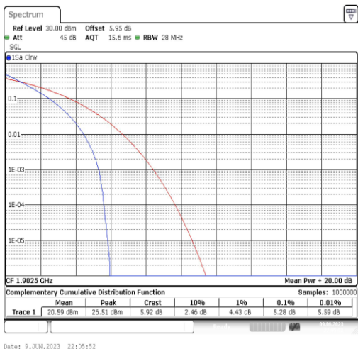
Band2-15MHz-QPSK-19125-75RB#0
