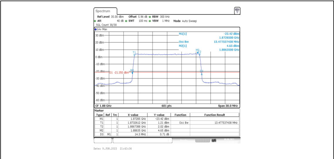
Band2-15MHz-16QAM-18900-75RB#0-13.478
