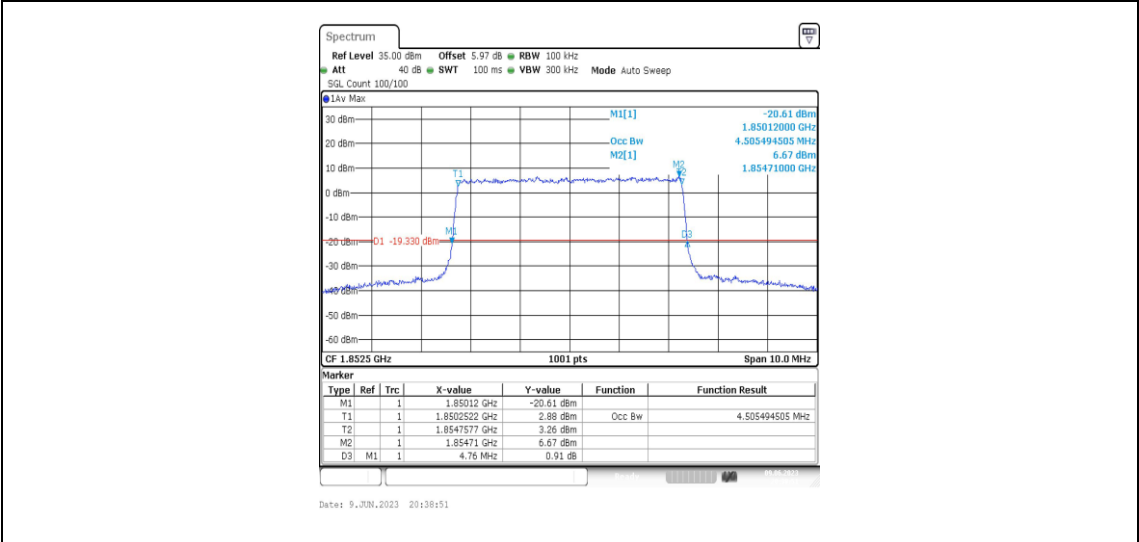
Band2-5MHz-16QAM-18625-25RB#0-4.505
