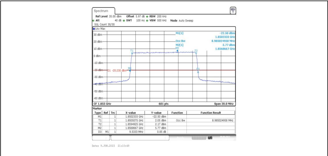
Band2-10MHz-QPSK-18650-50RB#0-8.985
