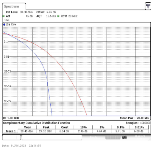
Band2-15MHz-QPSK-18900-75RB#0
