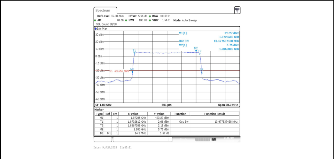
Band2-15MHz-QPSK-18900-75RB#0-13.478
