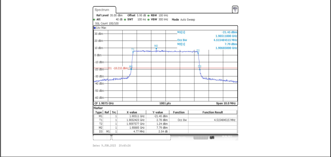
Band2-5MHz-16QAM-19175-25RB#0-4.515
