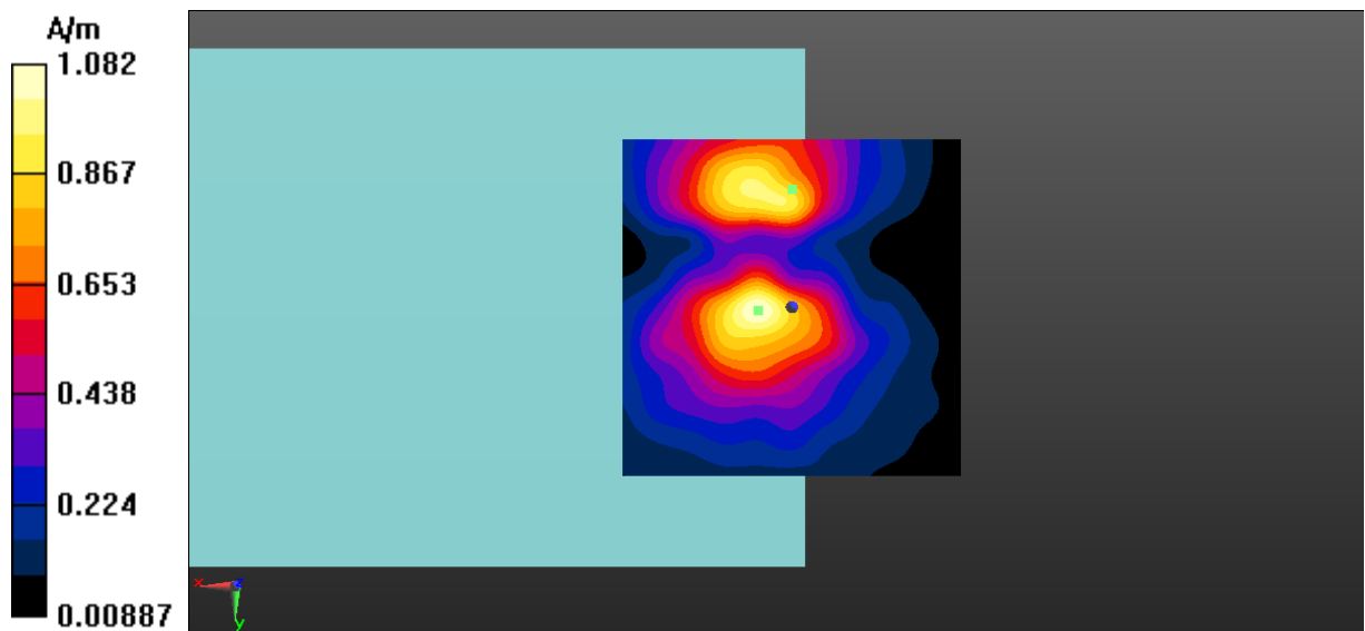
Fig A.20 T-Coil WLAN 2.4GHz-Y
