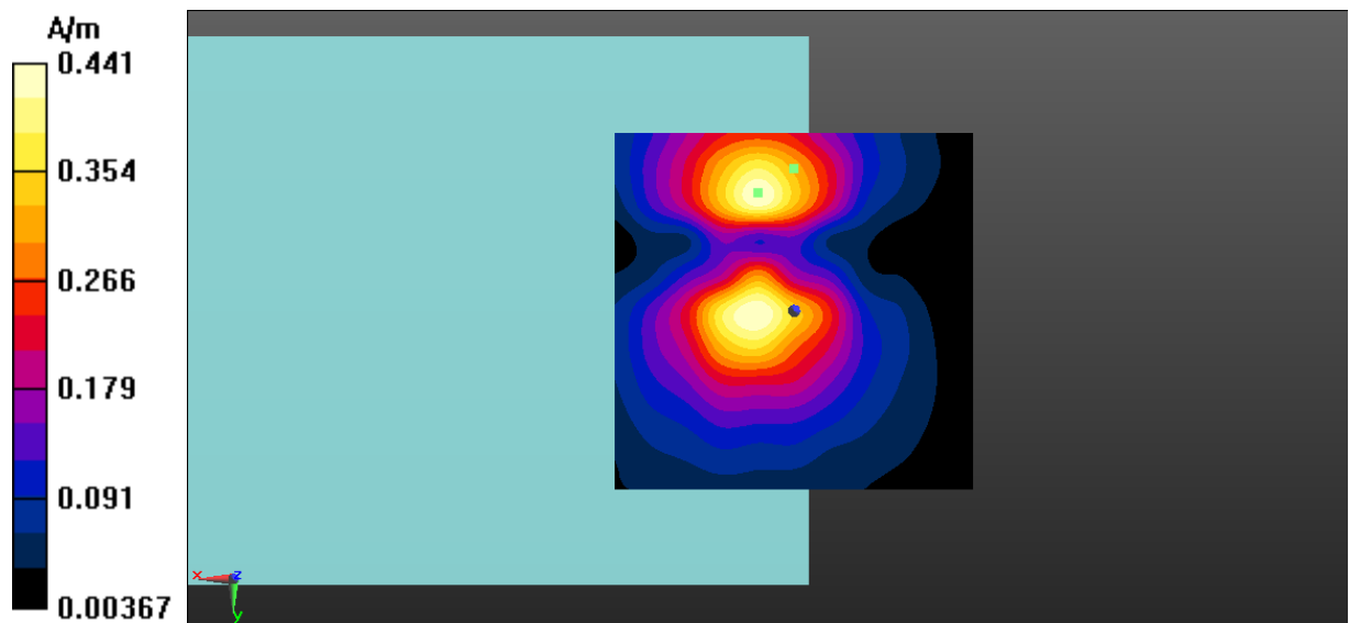
Fig A.9 T-Coil LTE-Band 12-Y
