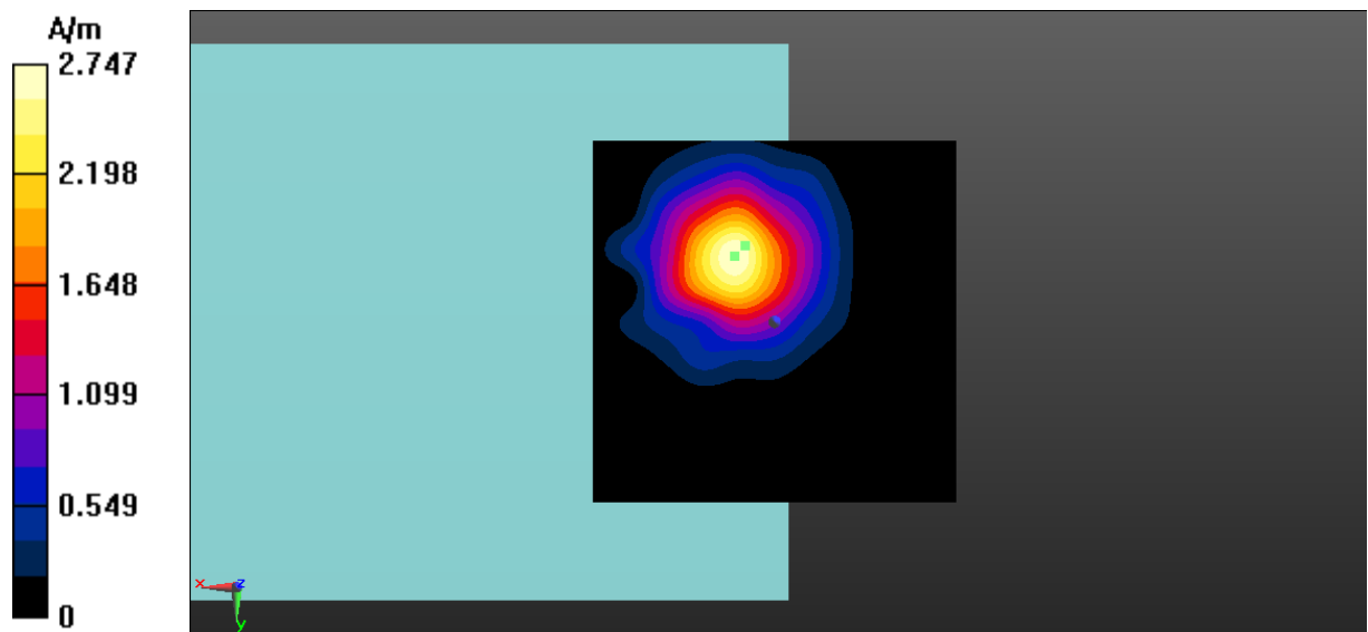
Fig A.20 T-Coil WLAN 2.4GHz-Z
