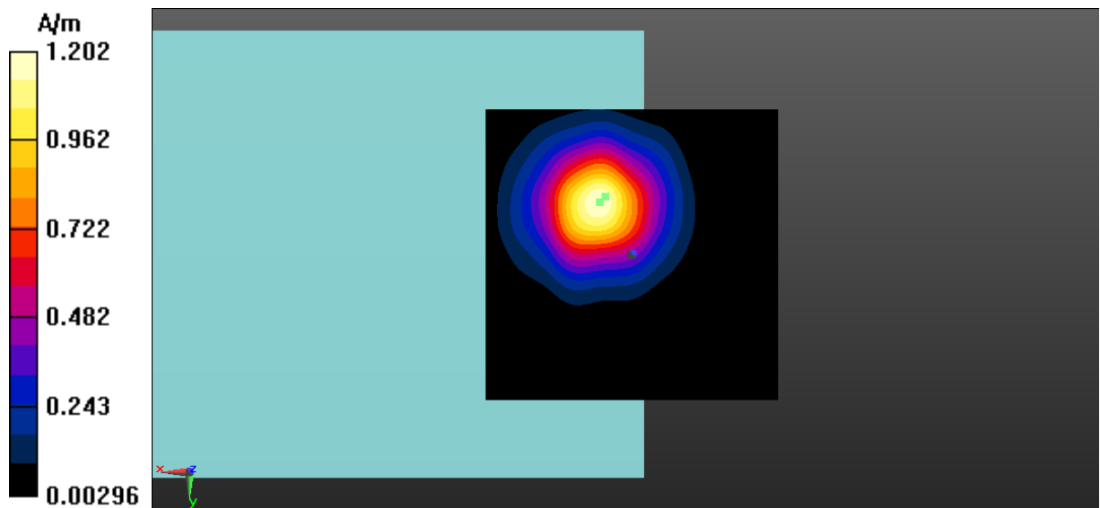
Fig A.13 T-Coil WLAN 5.2GHz-Z
