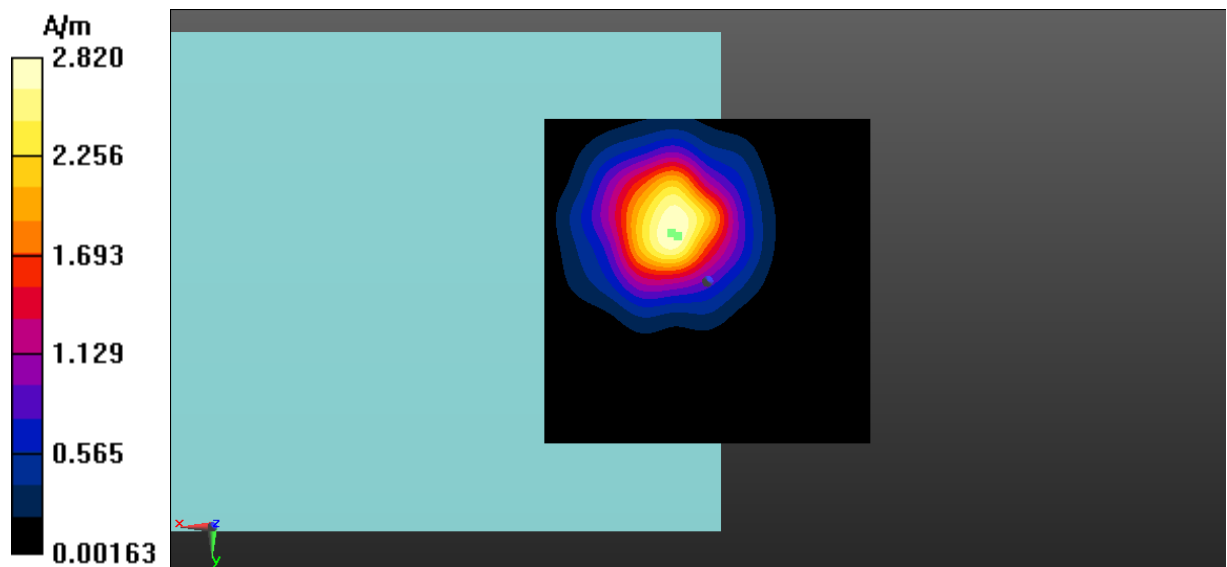
Fig A.19 T-Coil LTE-Band 66-Z
