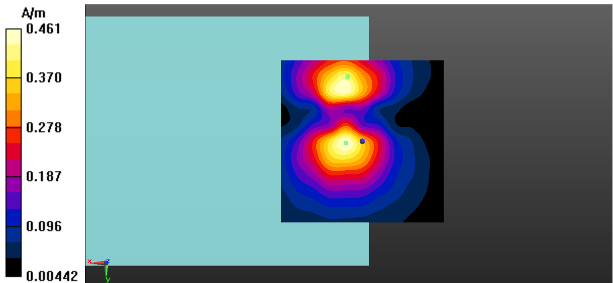
Fig A.14 T-Coil WLAN 5.3GHz-Y
