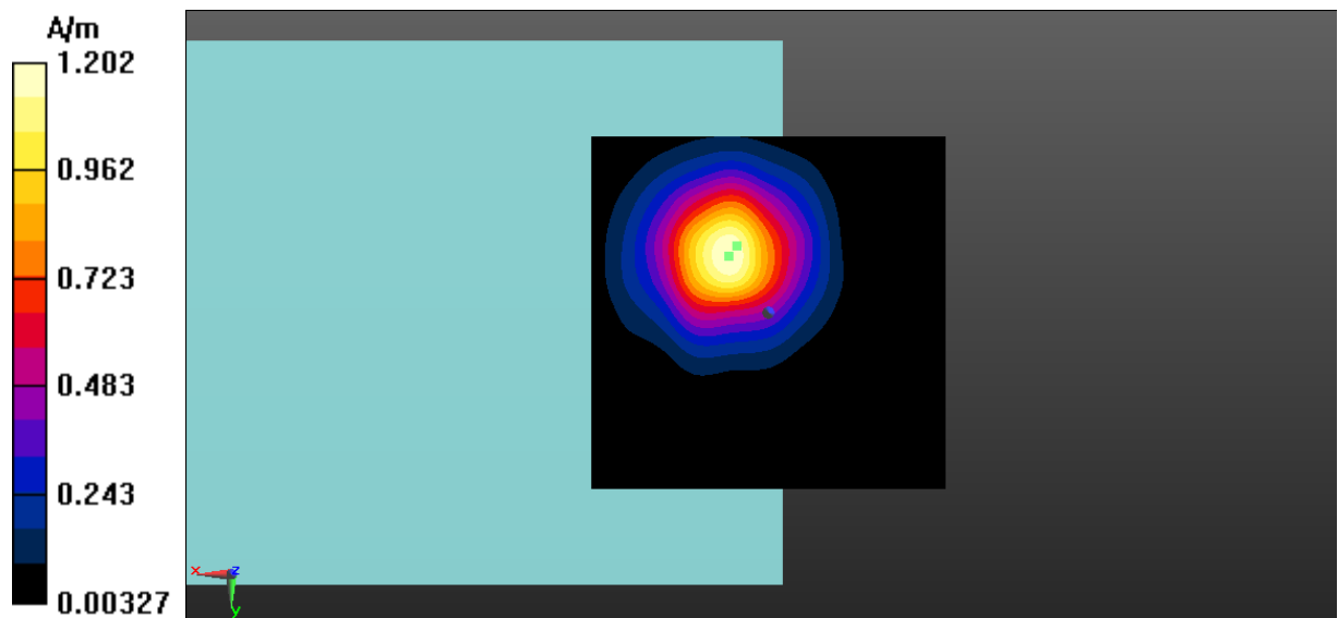
Fig A.15 T-Coil WLAN 5.5GHz-Z
