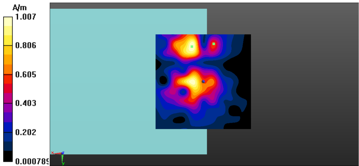
Fig A.18 T-Coil WCDMA Band 4-Y
