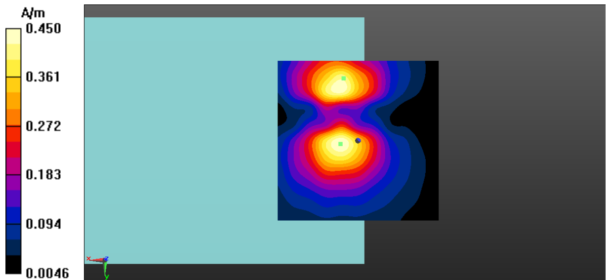
Fig A.16 T-Coil WLAN 5.8GHz-Y
