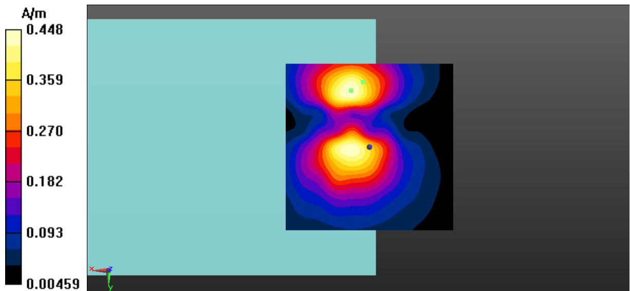
Fig A.13 T-Coil WLAN 5.2GHz-Y
