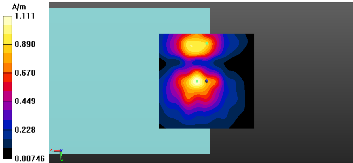
Fig A.19 T-Coil LTE-Band 66-Y
