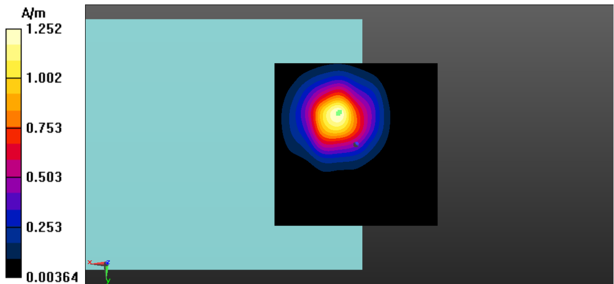
Fig A.16 T-Coil WLAN 5.8GHz-Z
