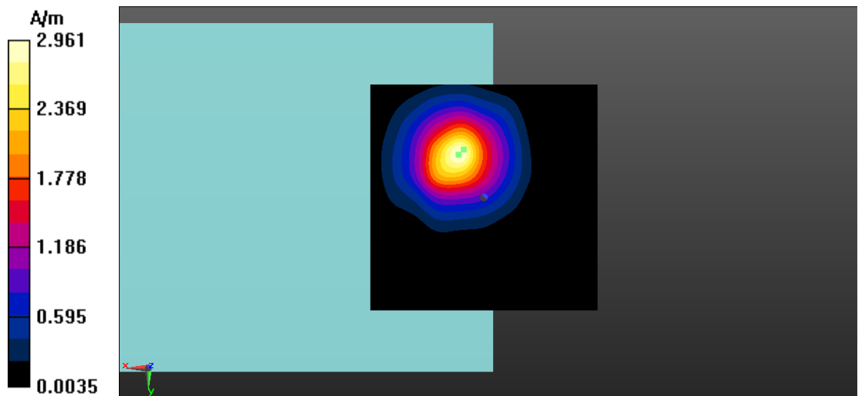
Fig A.18 T-Coil WCDMA Band 4-Z
