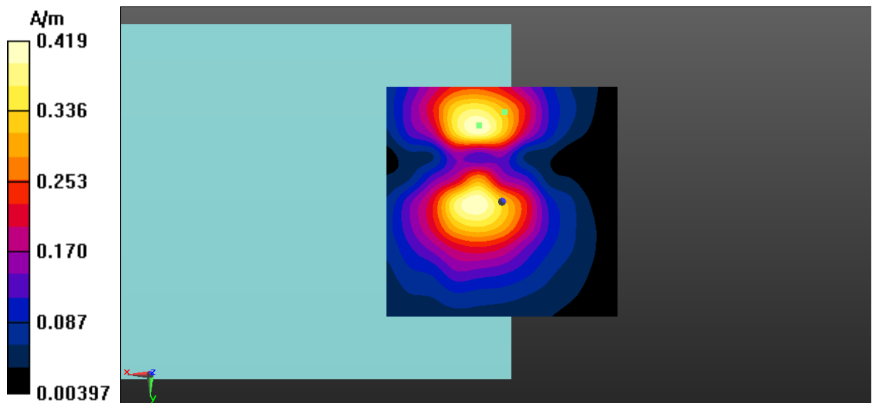
Fig A.10 T-Coil LTE-Band 66-Y
