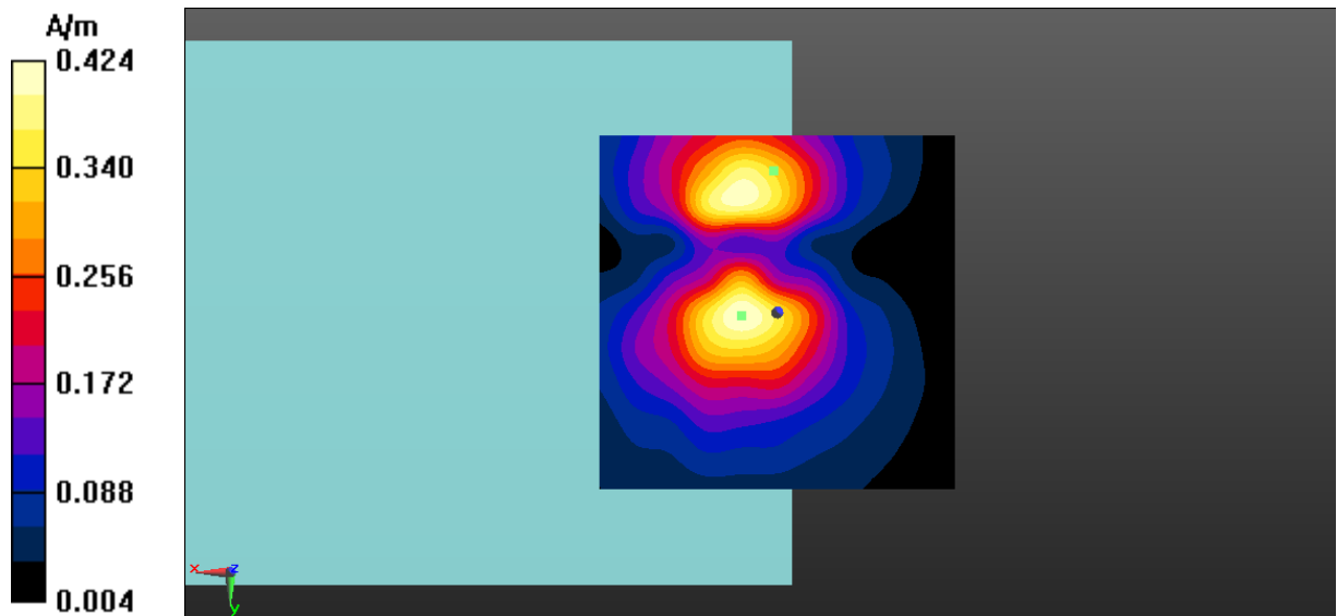
Fig A.11 T-Coil LTE-Band 71-Y
