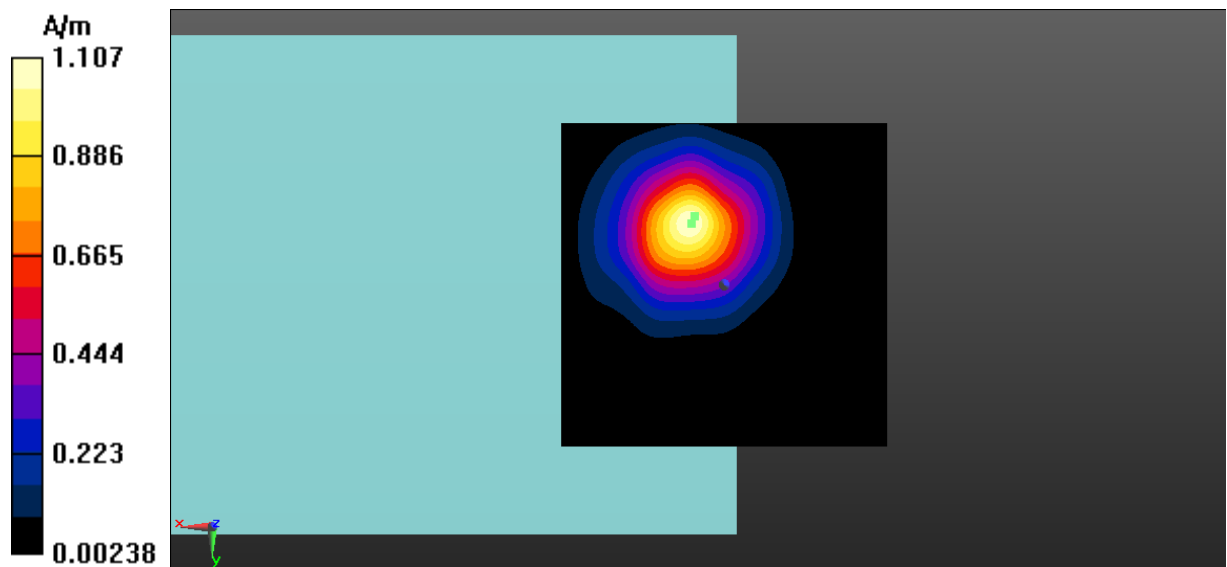
Fig A.11 T-Coil LTE-Band 71-Z
