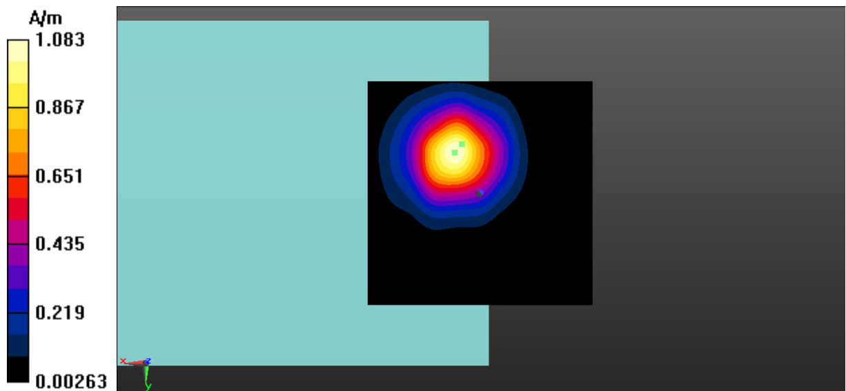
Fig A.9 T-Coil LTE-Band 12-Z
