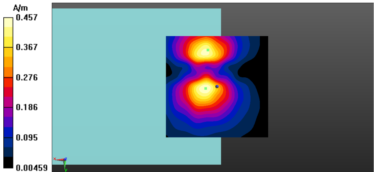
Fig A.15 T-Coil WLAN 5.5GHz-Y
