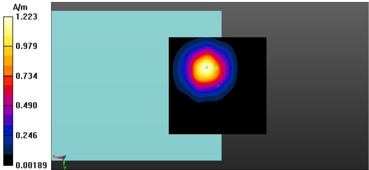
Fig A.12 T-Coil WLAN 2.4GHz-Z
