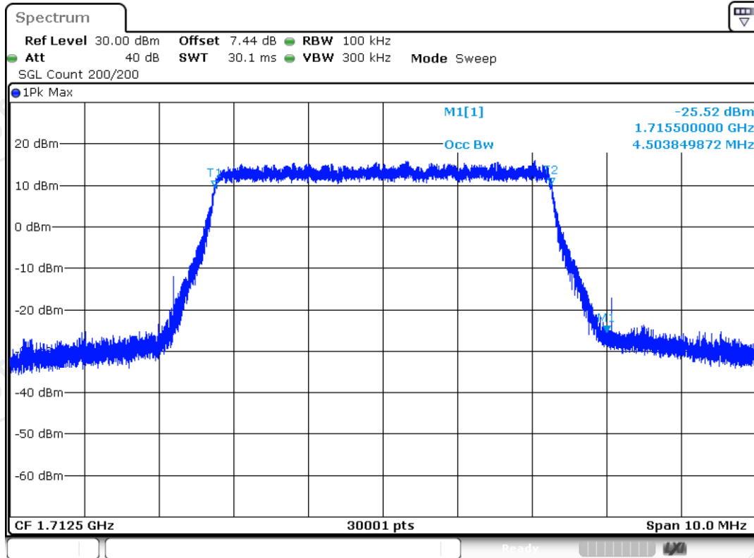
Band66 16QAM BW=5MHz Channel=131997 RB Size=25 Position=#0
