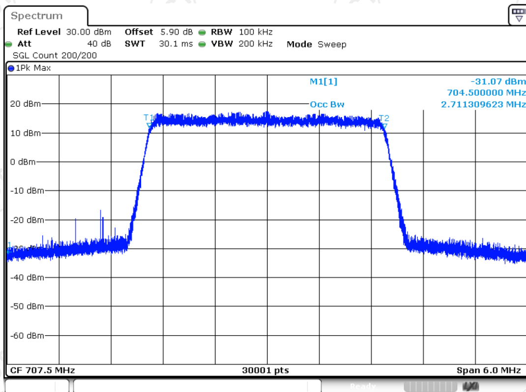
Band12 16QAM BW=3MHz Channel=23095 RB Size=15 Position=#0
