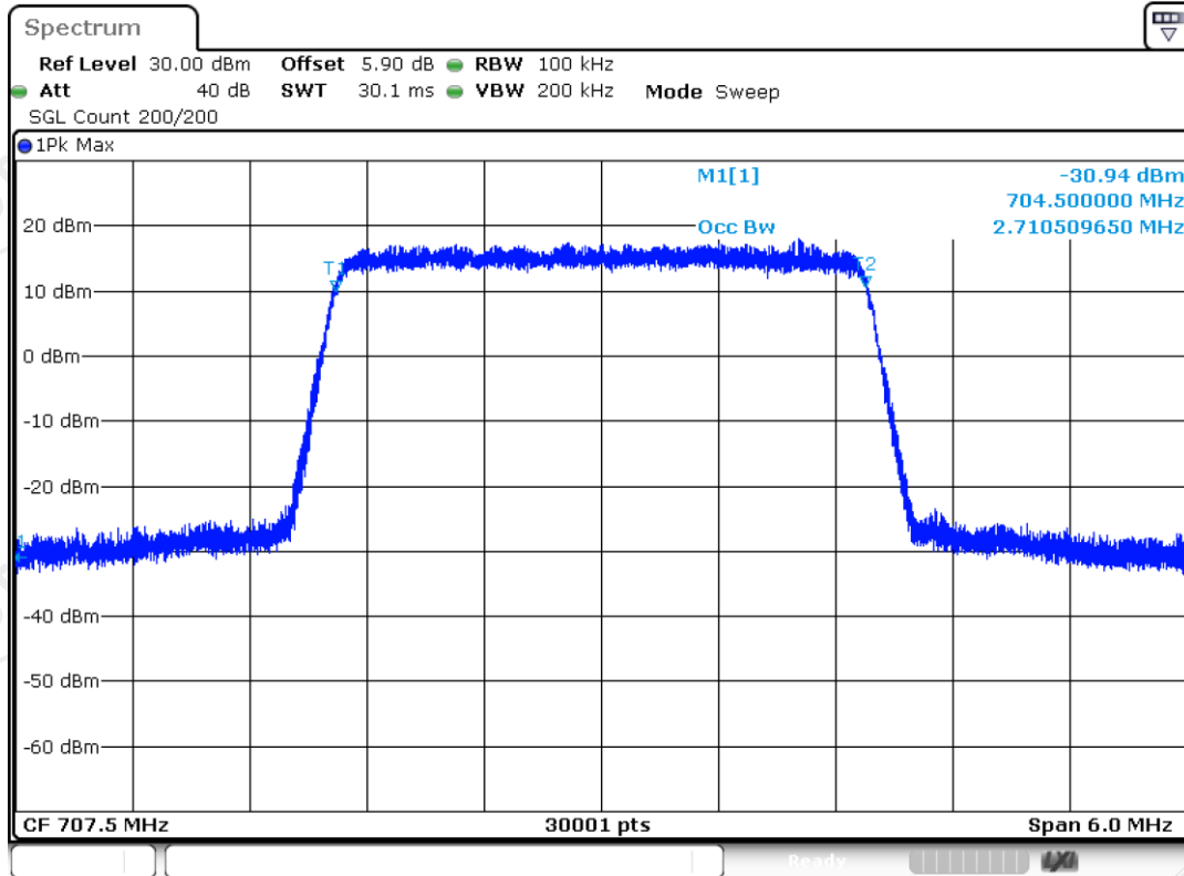
Band12 16QAM BW=3MHz Channel=23095 RB Size=15 Position=#0
