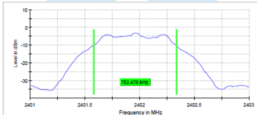
6 dB Bandwidth Plot on Configuration : 0 ch
