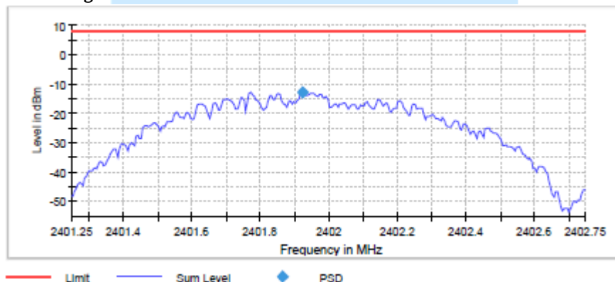
Power Density Plot on configuration : 0 ch
