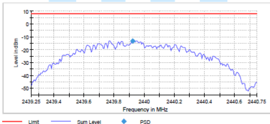
Power Density Plot on configuration : 19 ch
