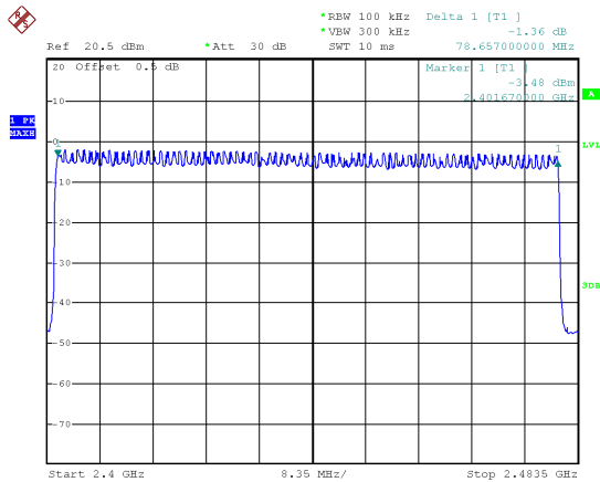
Modulation: 8DPSK
