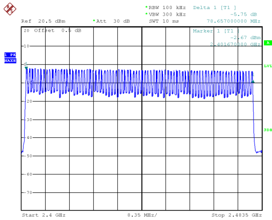
Modulation: GFSK
