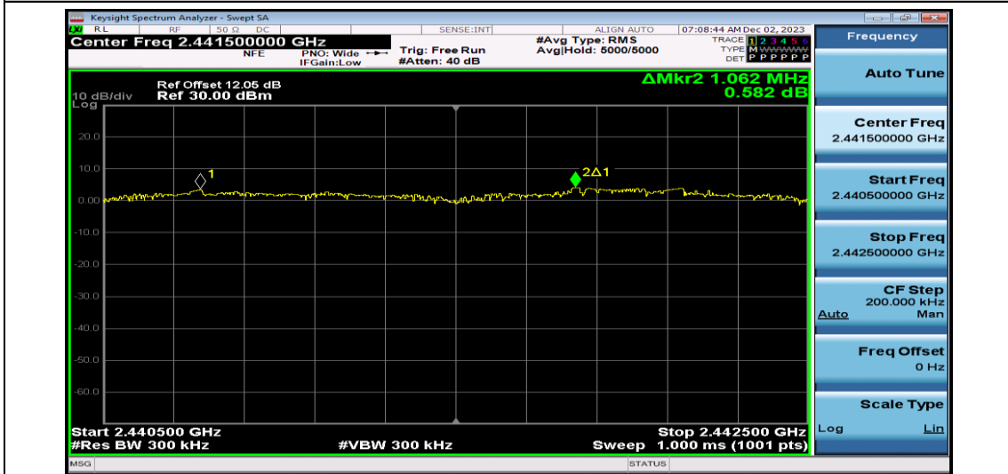
2DH5-Ant1-Hop
