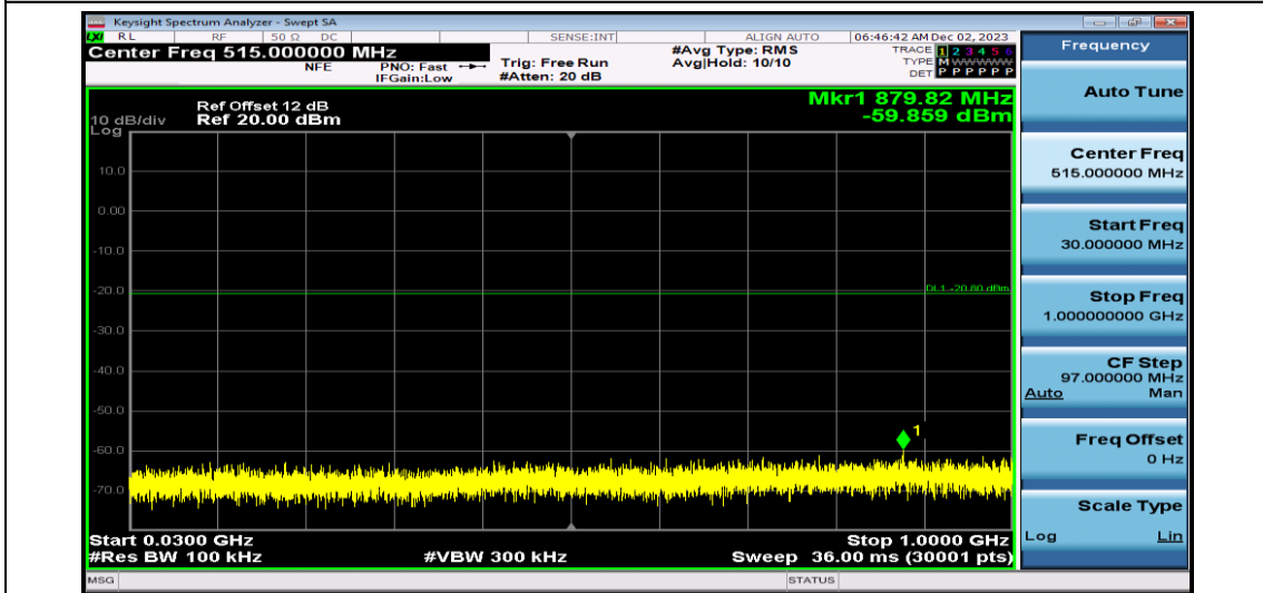
2DH5-Ant1-2480-30~1000
