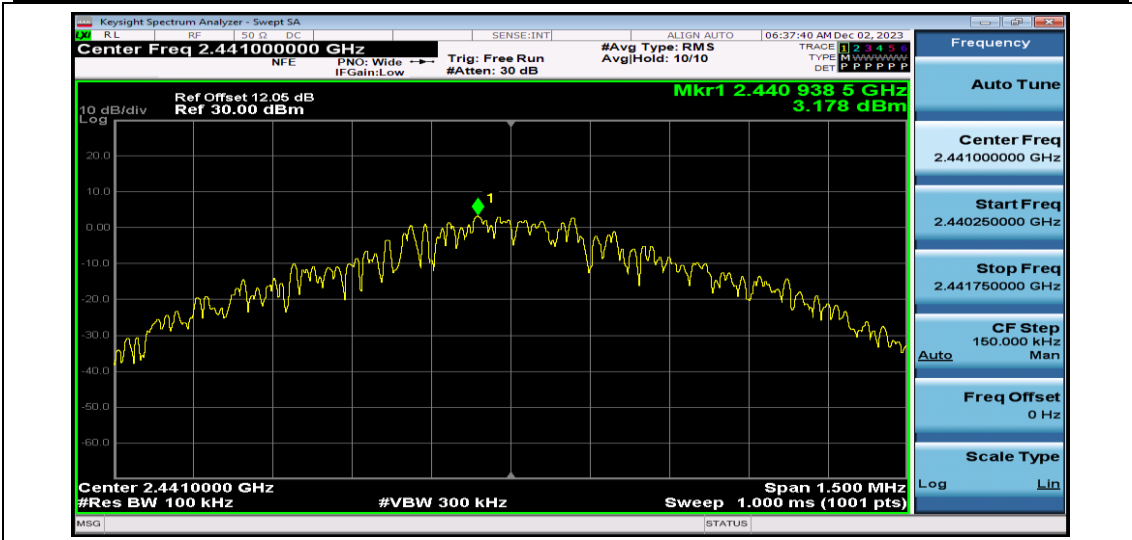
DH5-Ant1-2441-0~Reference
