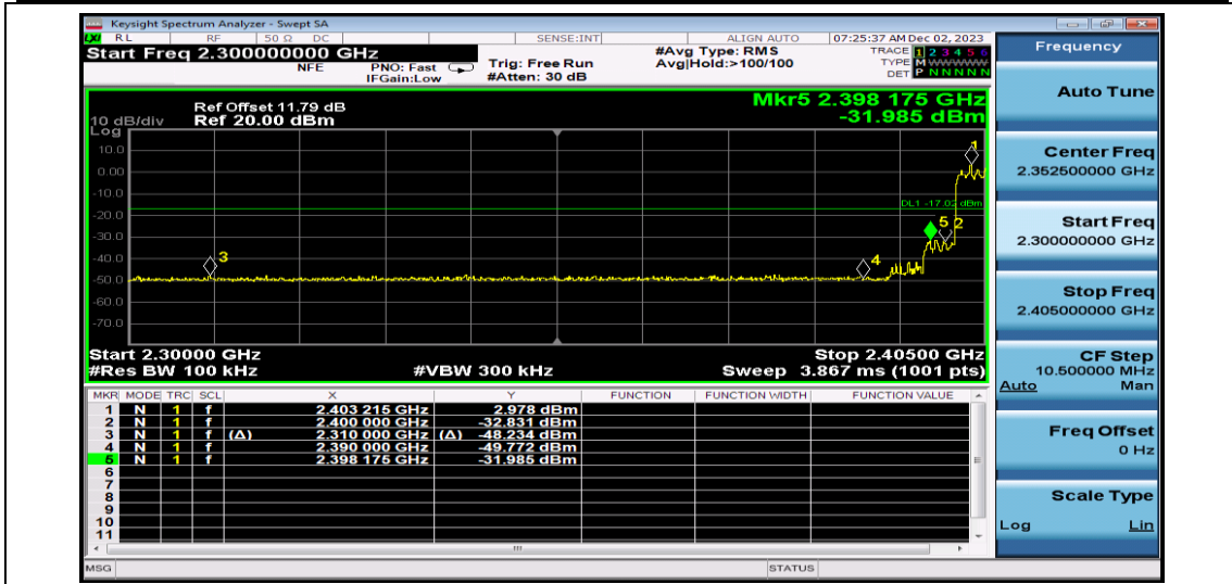
2DH5-Ant1-Hop_2402
