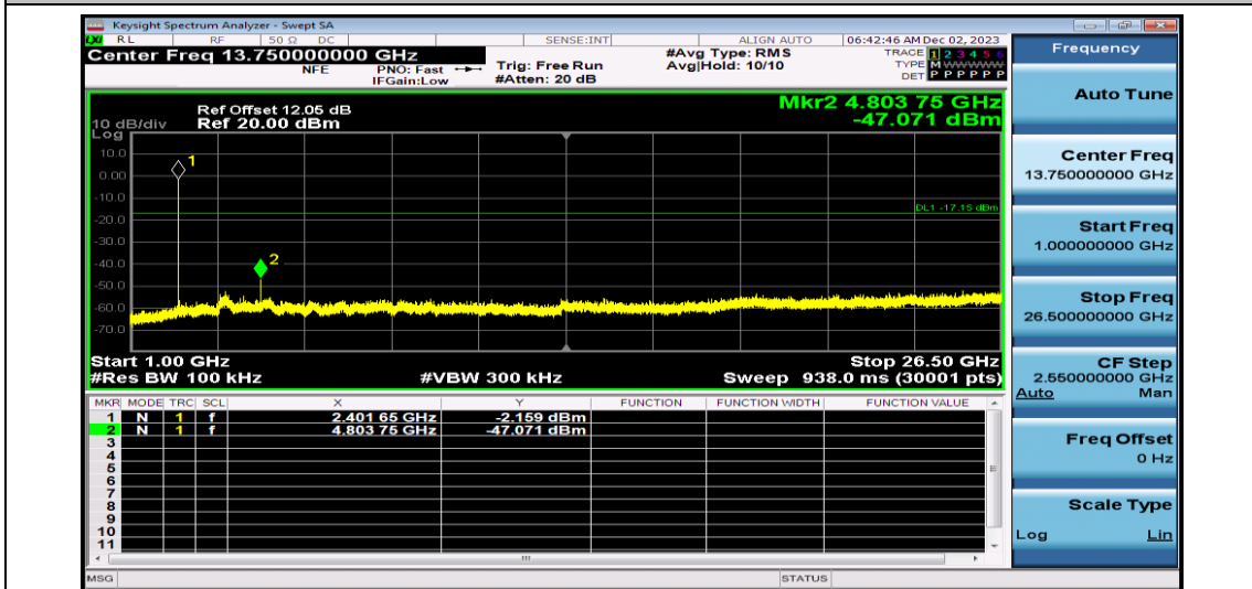
2DH5-Ant1-2402-1000~26500
