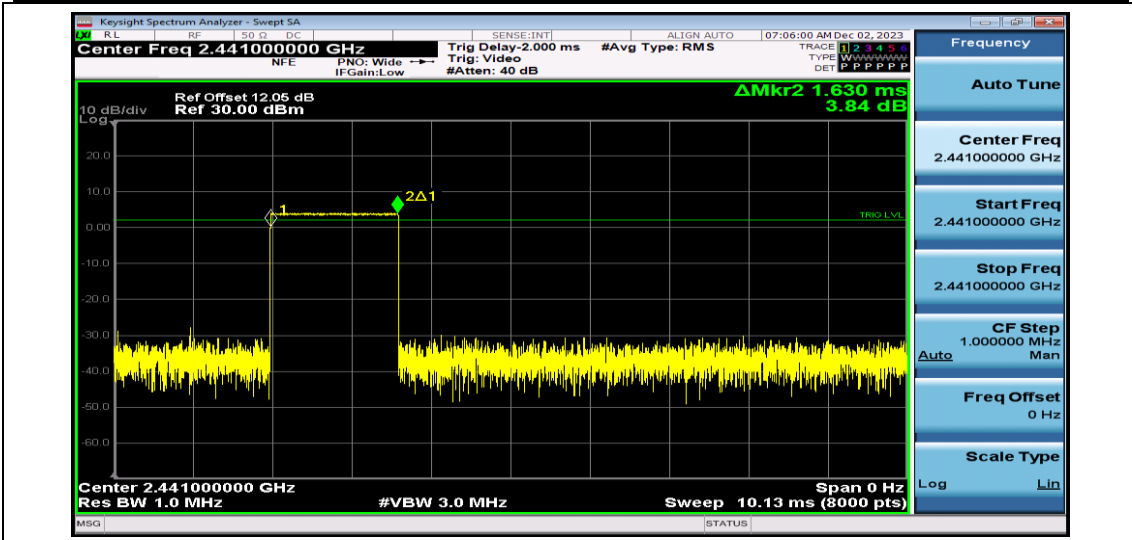
DH3-Ant1-Hop
