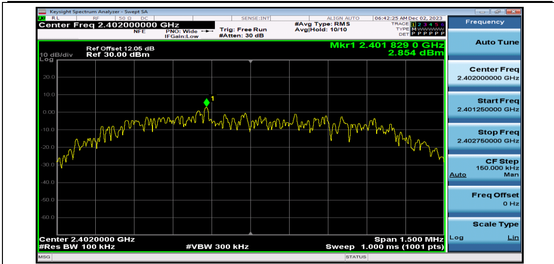
2DH5-Ant1-2402-0~Reference
