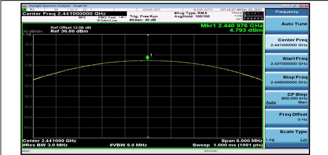
2DH5-Ant1-2441
