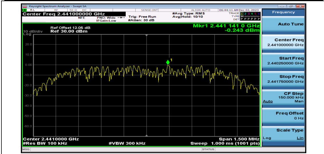
2DH5-Ant1-2441-0~Reference
