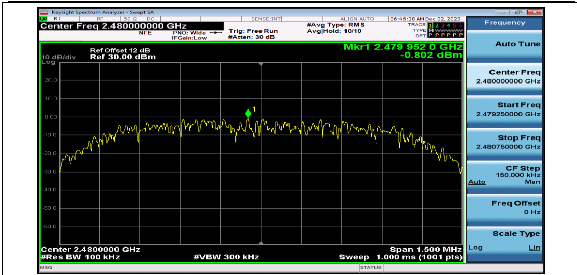
2DH5-Ant1-2480-0-Reference
