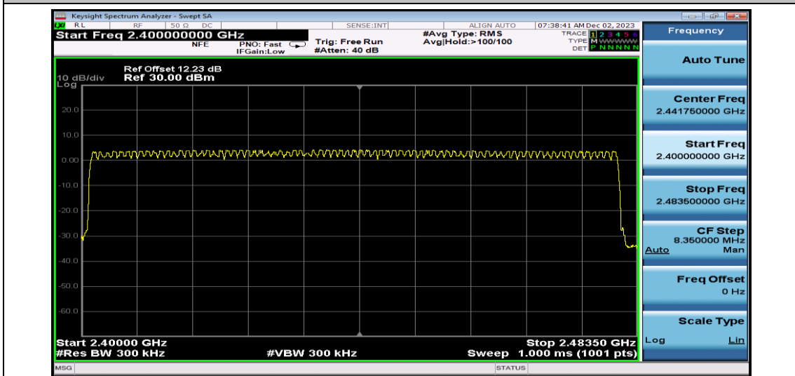
2DH5-Ant1-Hop
