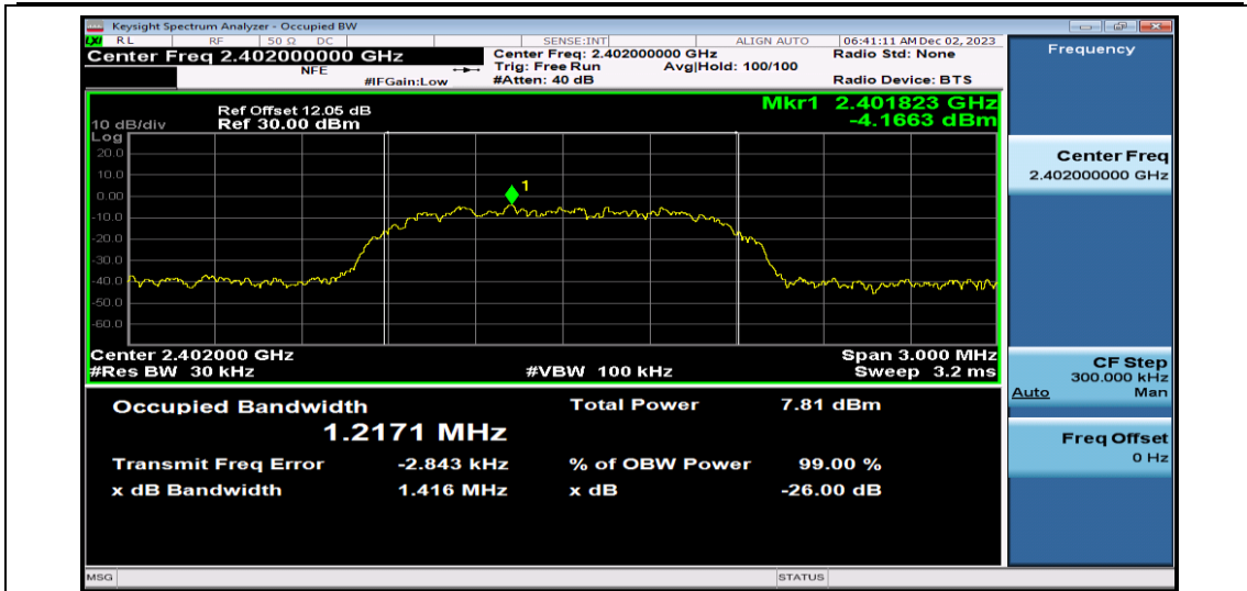
2DH5-Ant1-2402
