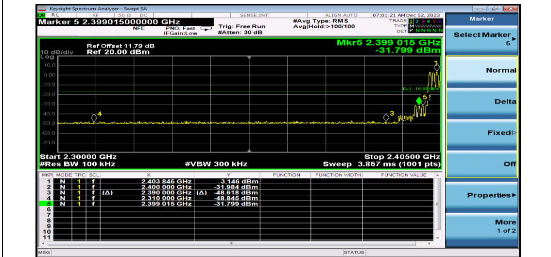
DH5-Ant1-Hop_2402
