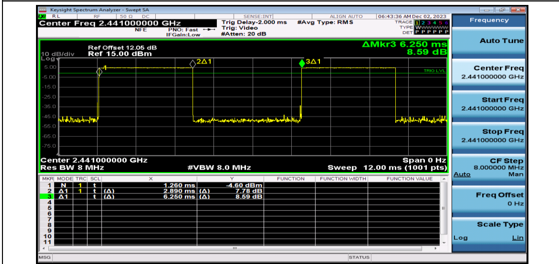
NTNV-2DH5-Ant1-2441
