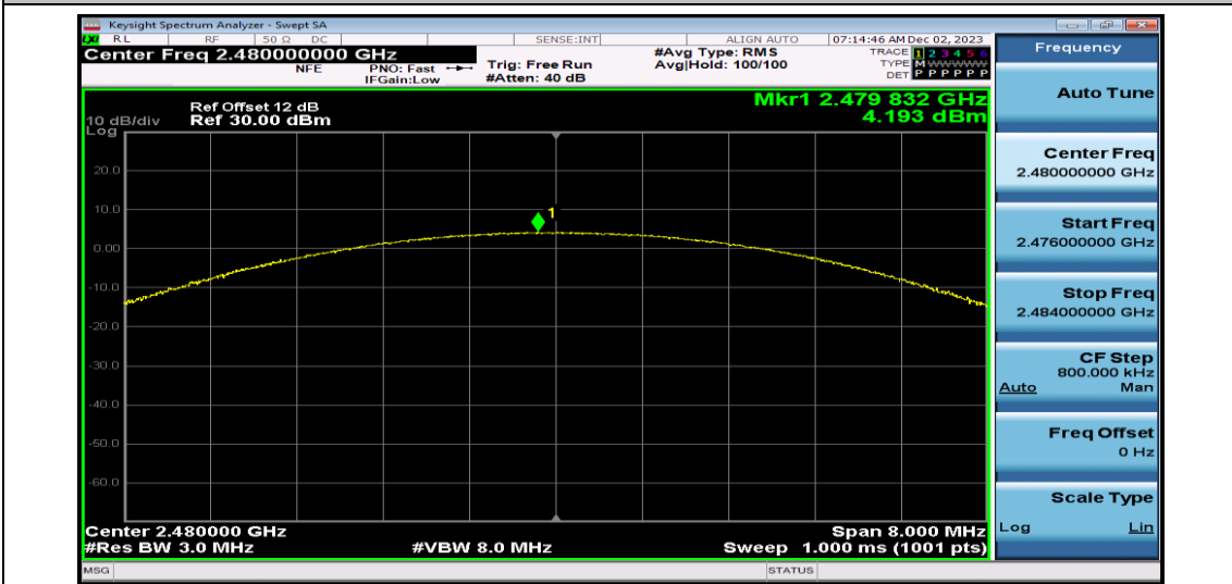
2DH5-Ant1-2480
