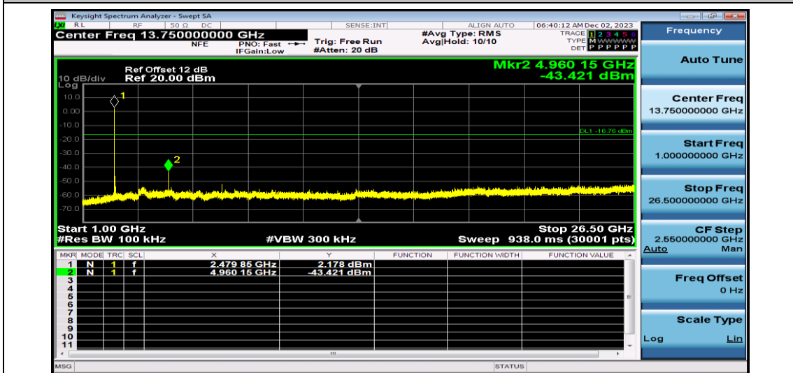
DH5-Ant1-2480-1000~26500
