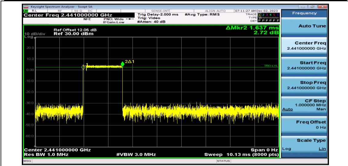
2DH3-Ant1-Hop
