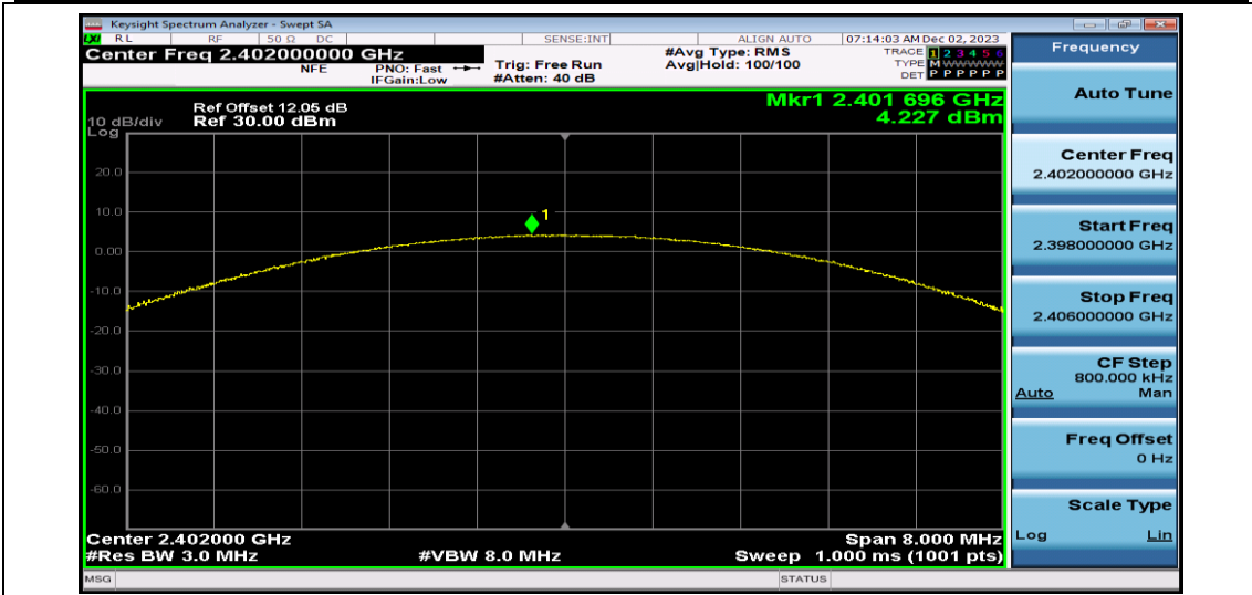
2DH5-Ant1-2402
