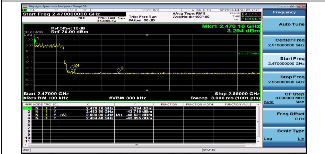
2DH5-Ant1-Hop_2480
