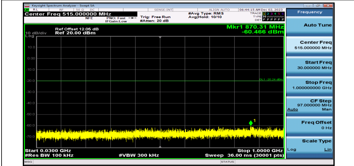
2DH5-Ant1-2441-30~1000
