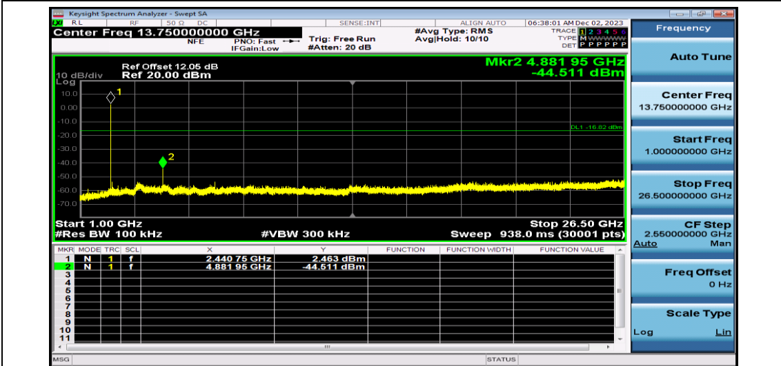
DH5-Ant1-2441-1000~26500
