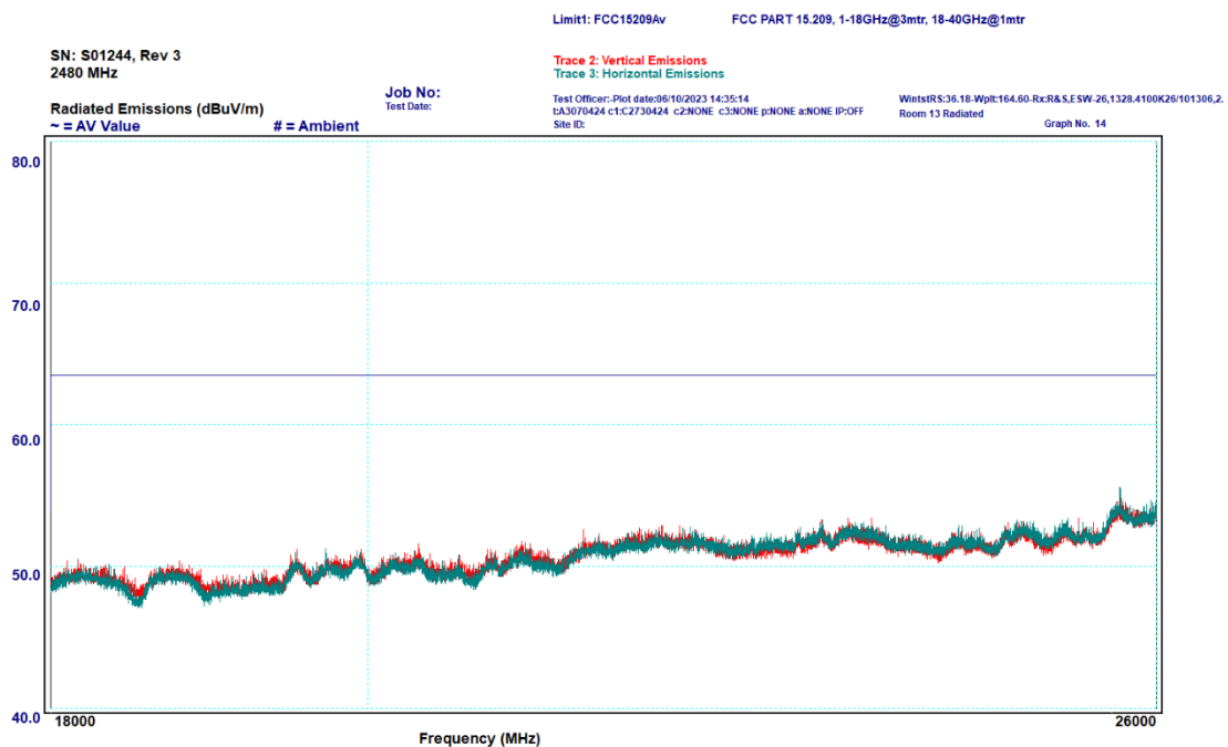
Graph 6-18: Transmitter Spurious Emissions, 18 – 26 GHz, 2480 MHz, Average
