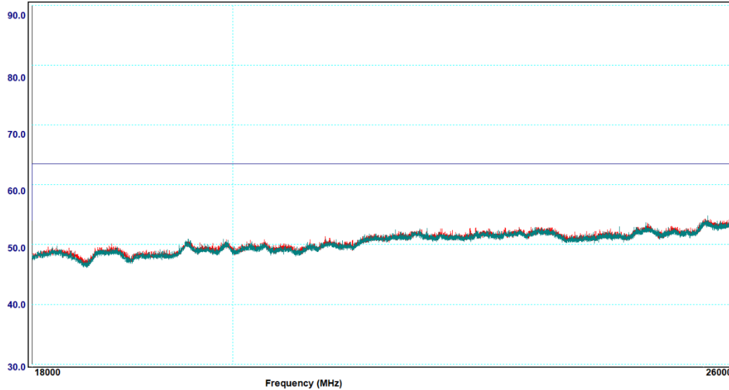
Graph 6-23: Transmitter Spurious Emissions, 18 – 26 GHz, 2440 MHz, Average
