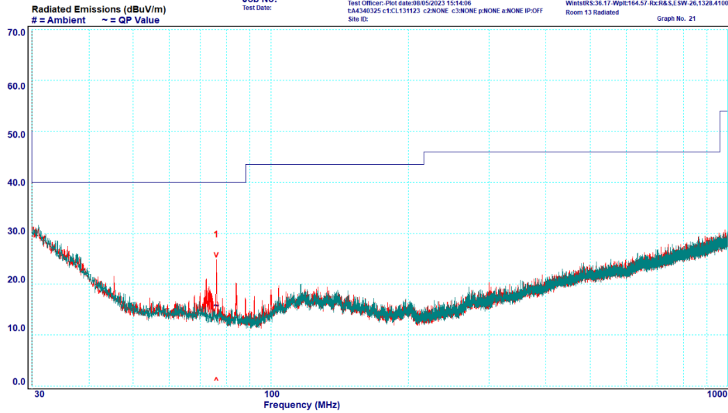
Graph 6-12: Transmitter Spurious Emissions, 30 – 1000 MHz, 2480 MHz
