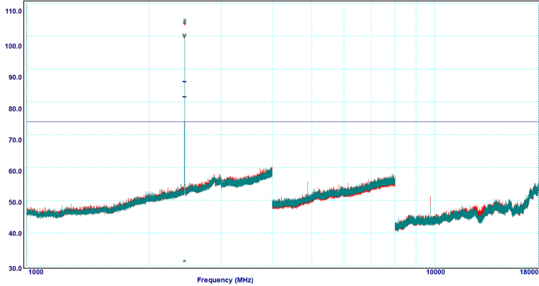
Graph 6-14: Transmitter Spurious Emissions, 1 – 18 GHz, 2440 MHz, Peak
