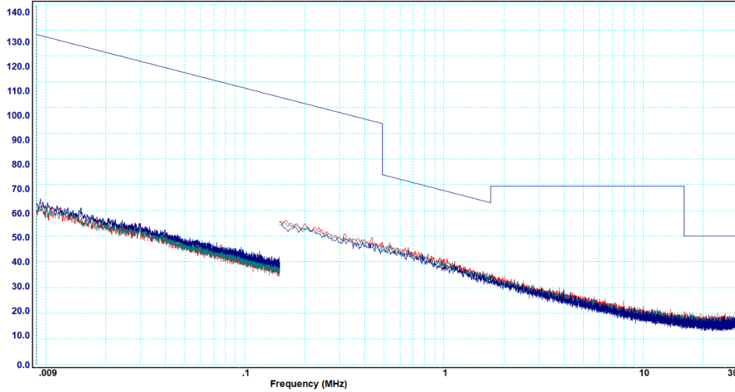
Graph 6-8: Transmitter Spurious Emissions, 9 kHz – 30 MHz, 2440 MHz
