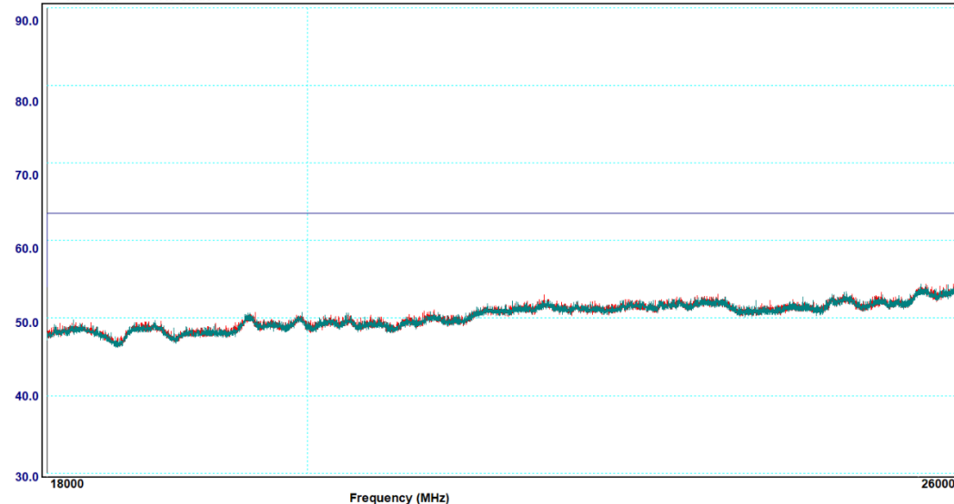
Graph 6-22: Transmitter Spurious Emissions, 18 – 26 GHz, 2402 MHz, Average
