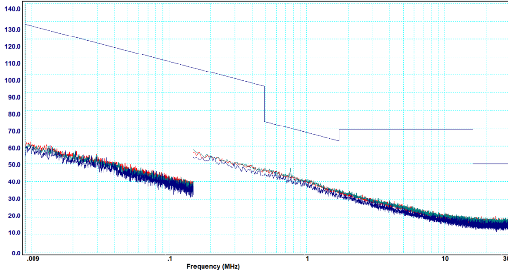
Graph 6-9: Transmitter Spurious Emissions, 9 kHz – 30 MHz, 2480 MHz
