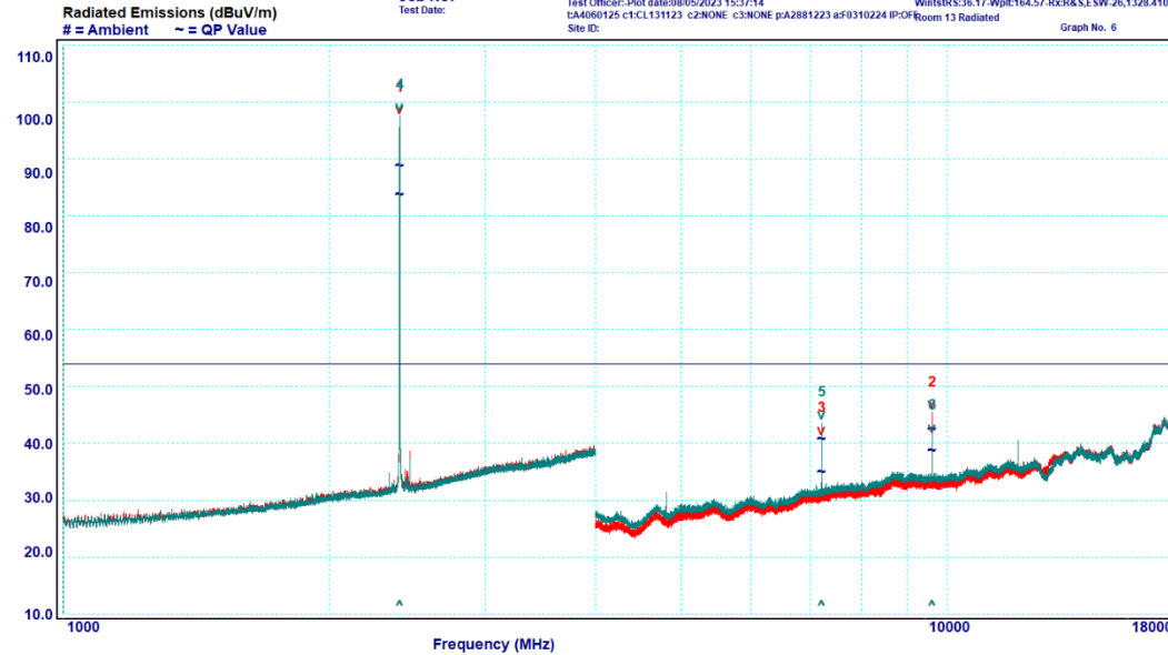
Graph 6-16: Transmitter Spurious Emissions, 1 – 18 GHz, 2402 MHz, Average
