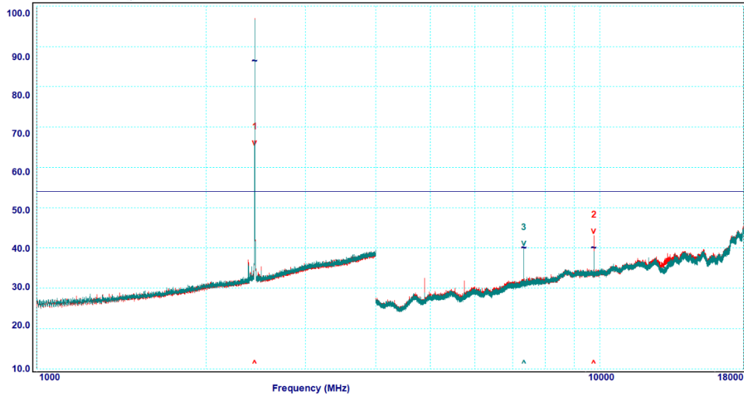
Graph 6-17: Transmitter Spurious Emissions, 1 – 18 GHz, 2440 MHz, Average
