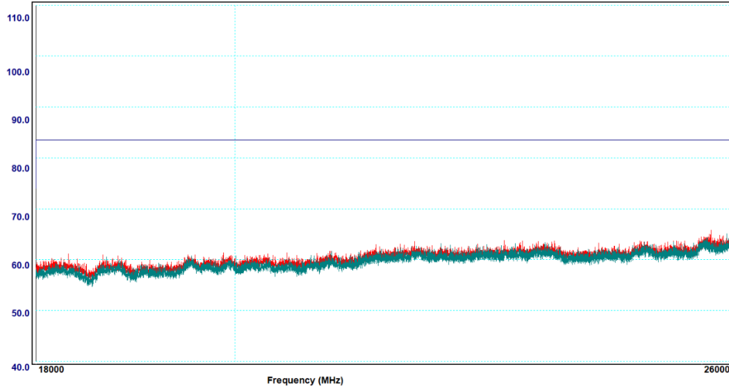
Graph 6-21: Transmitter Spurious Emissions, 18 – 26 GHz, 2480 MHz, Peak
