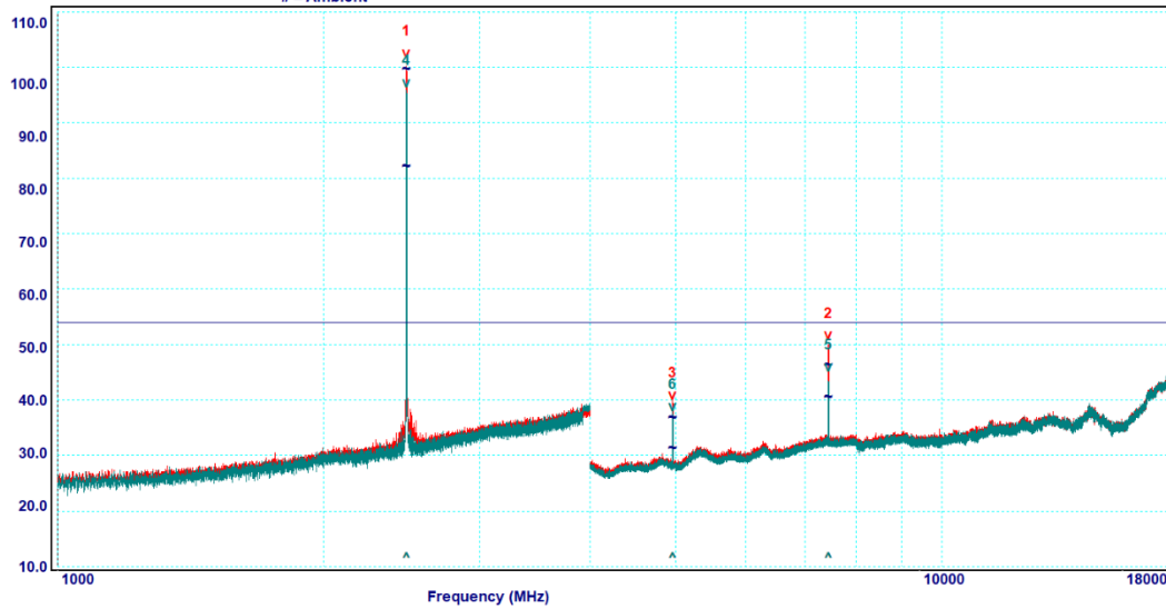
Graph 6-18: Transmitter Spurious Emissions, 1 – 18 GHz, 2480 MHz, Average
