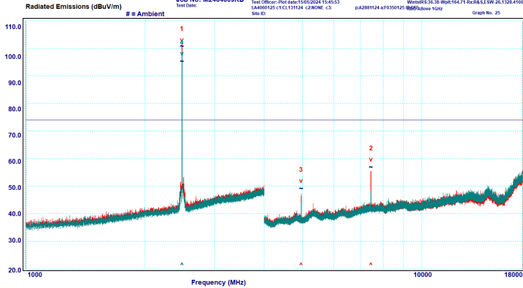
Graph 6-15: Transmitter Spurious Emissions, 1 – 18 GHz, 2480 MHz, Peak
