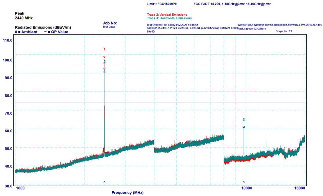
Graph 6-14: Transmitter Spurious Emissions, 1 – 18 GHz, 2440 MHz, Peak
