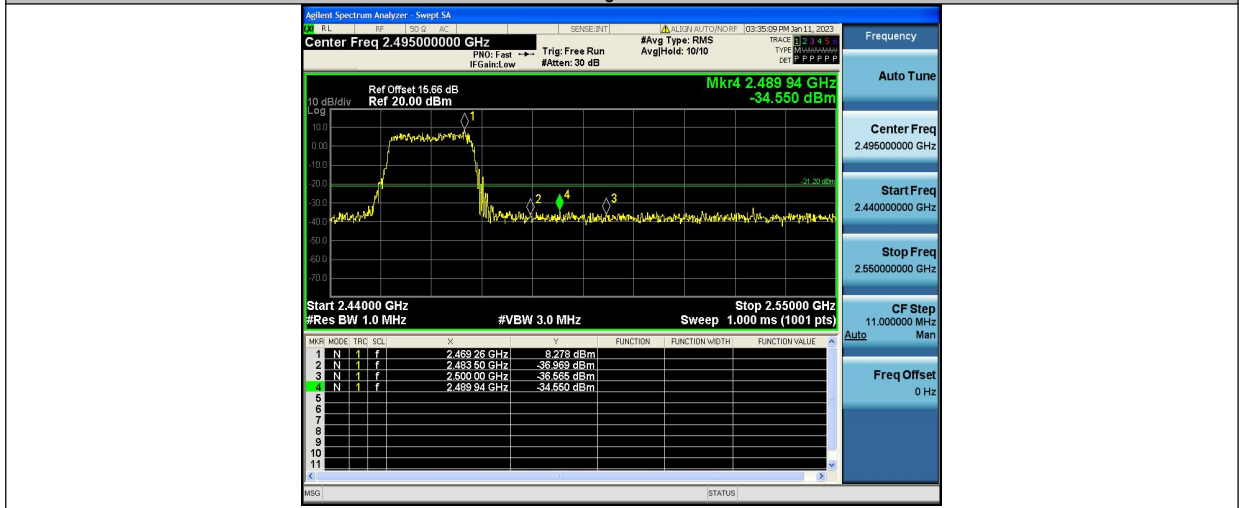
11N20SISO-Ant1-High-2462-AV-2483.500
