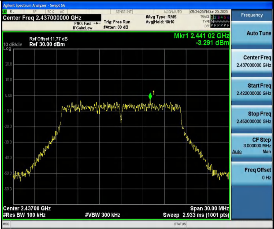
11G-Ant1-2437-0~Reference
