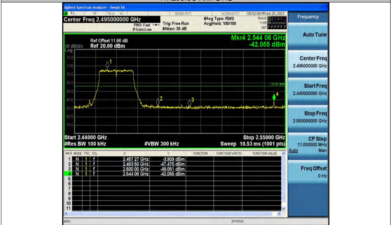
11N20SISO-Ant1-2462
