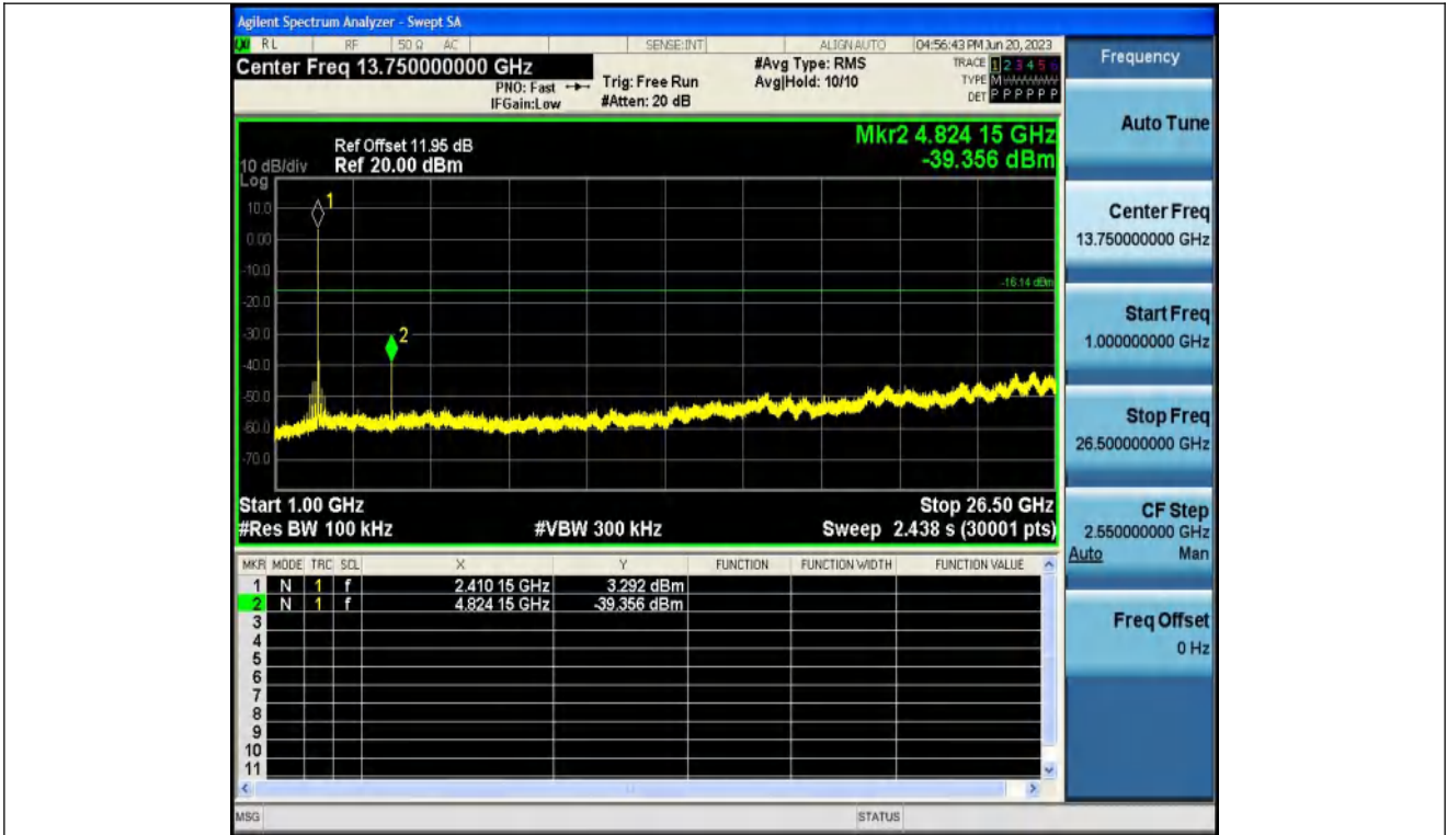
11B-Ant1-2412-1000~26500
