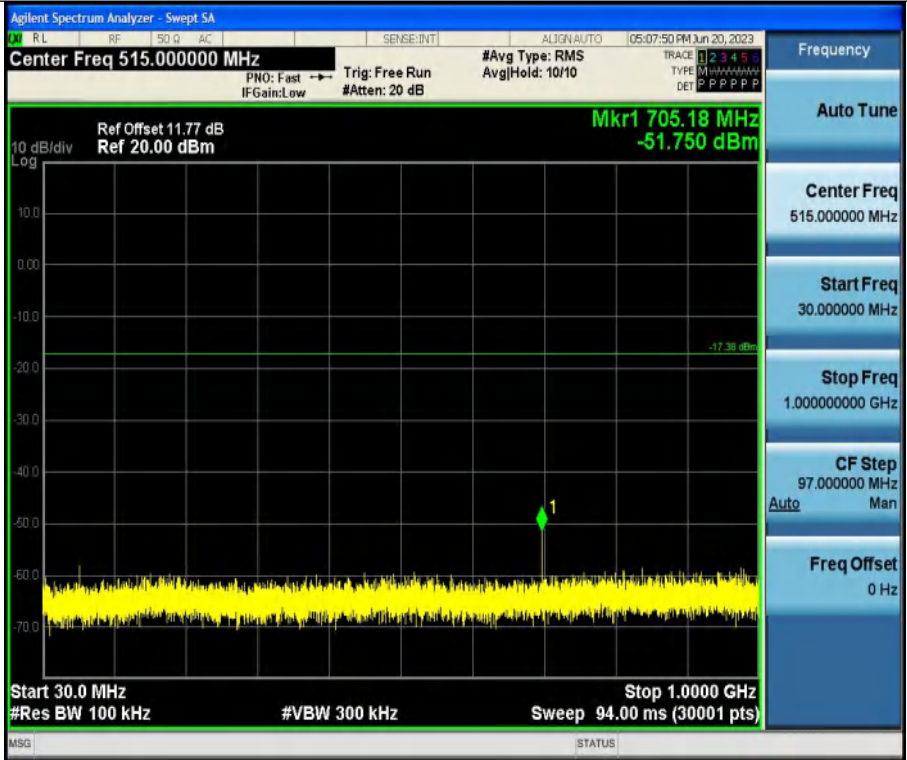
11B-Ant1-2437-30~1000
