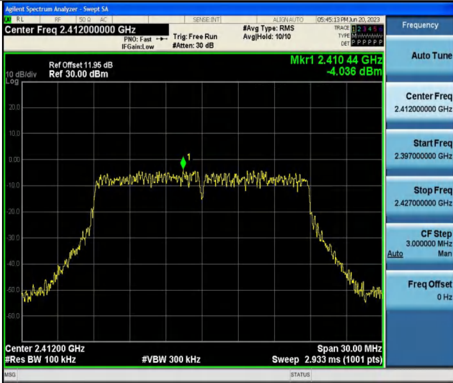
11N20SISO-Ant1-2412-0~Reference
