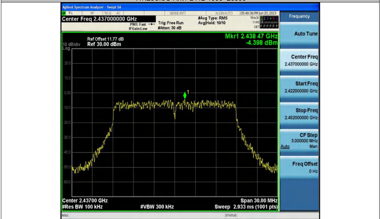
11N20SISO-Ant1-2437-0~Reference
