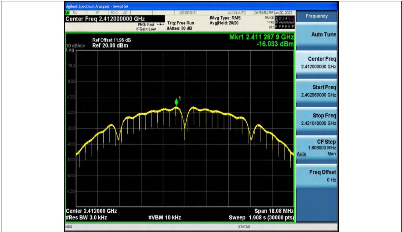
11B-Ant1-2412
