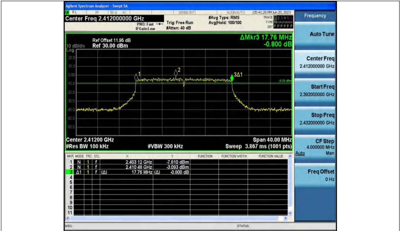
11N20SISO-Ant1-2412
