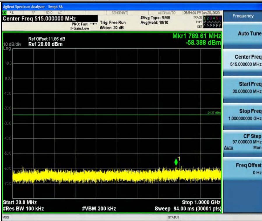
11N20SISO-Ant1-2462-30~1000
