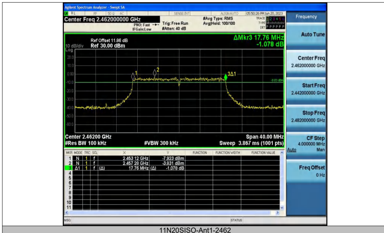
11N20SISO-Ant1-2462
