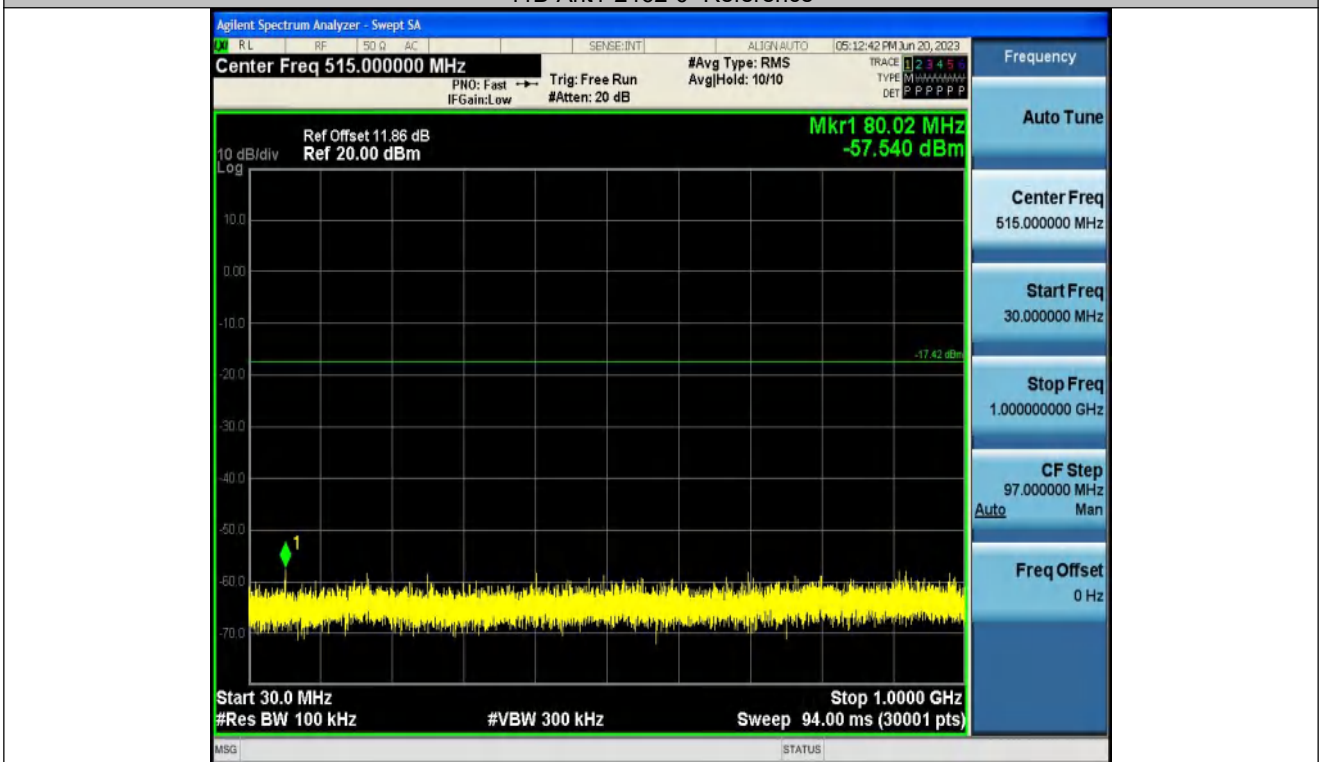
11B-Ant1-2462-30~1000
