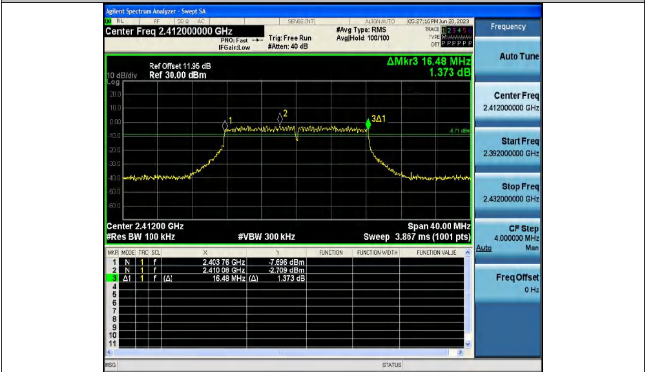
11G-Ant1-2412
