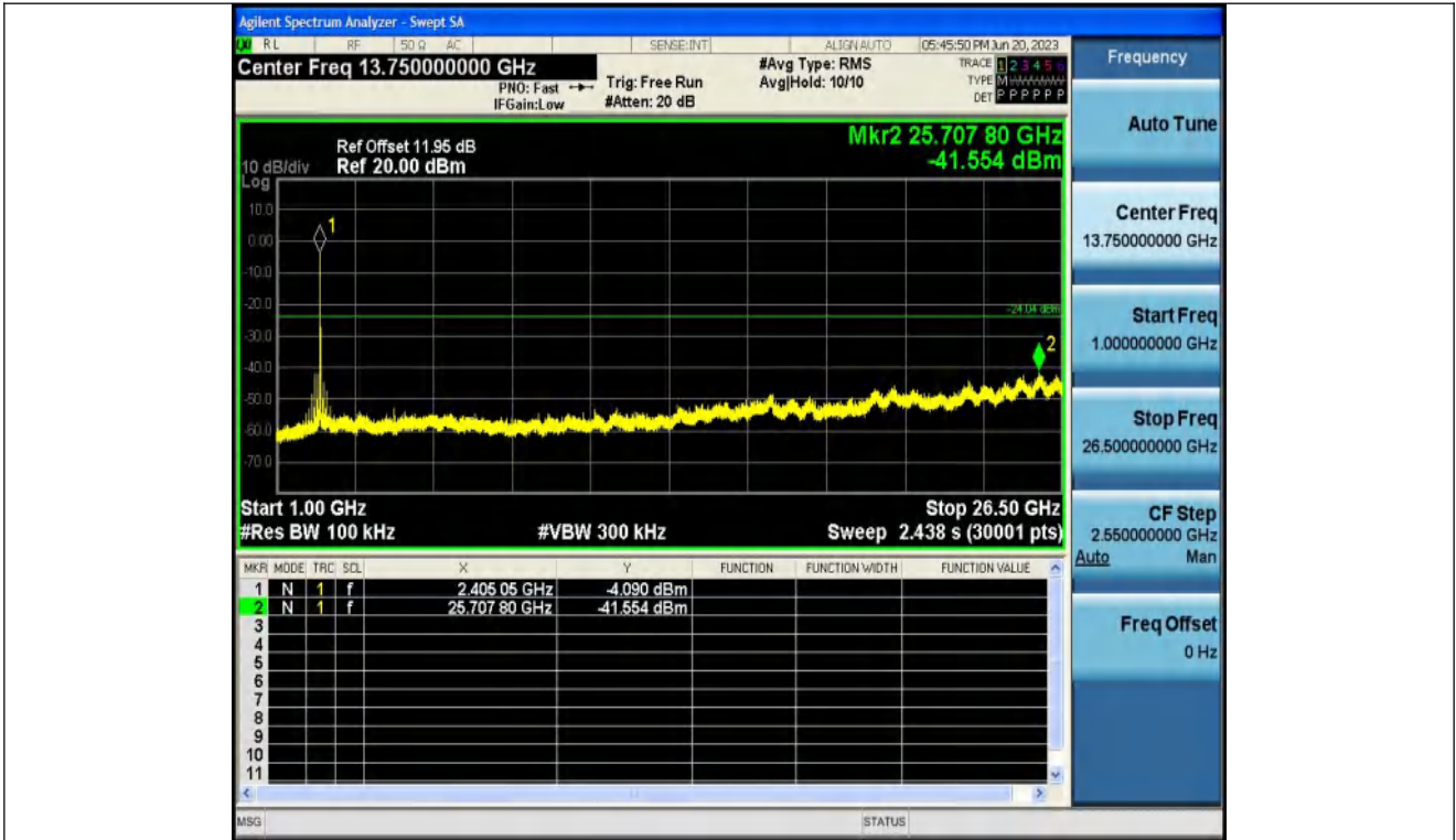
11N20SISO-Ant1-2412-1000~26500
