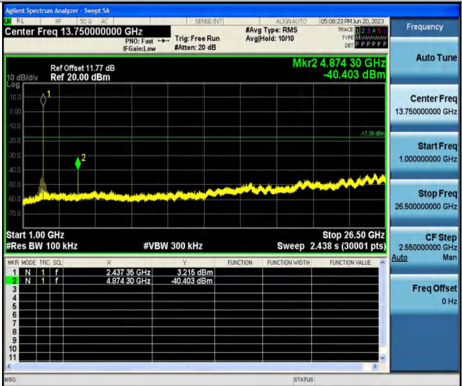
11B-Ant1-2437-1000~26500
