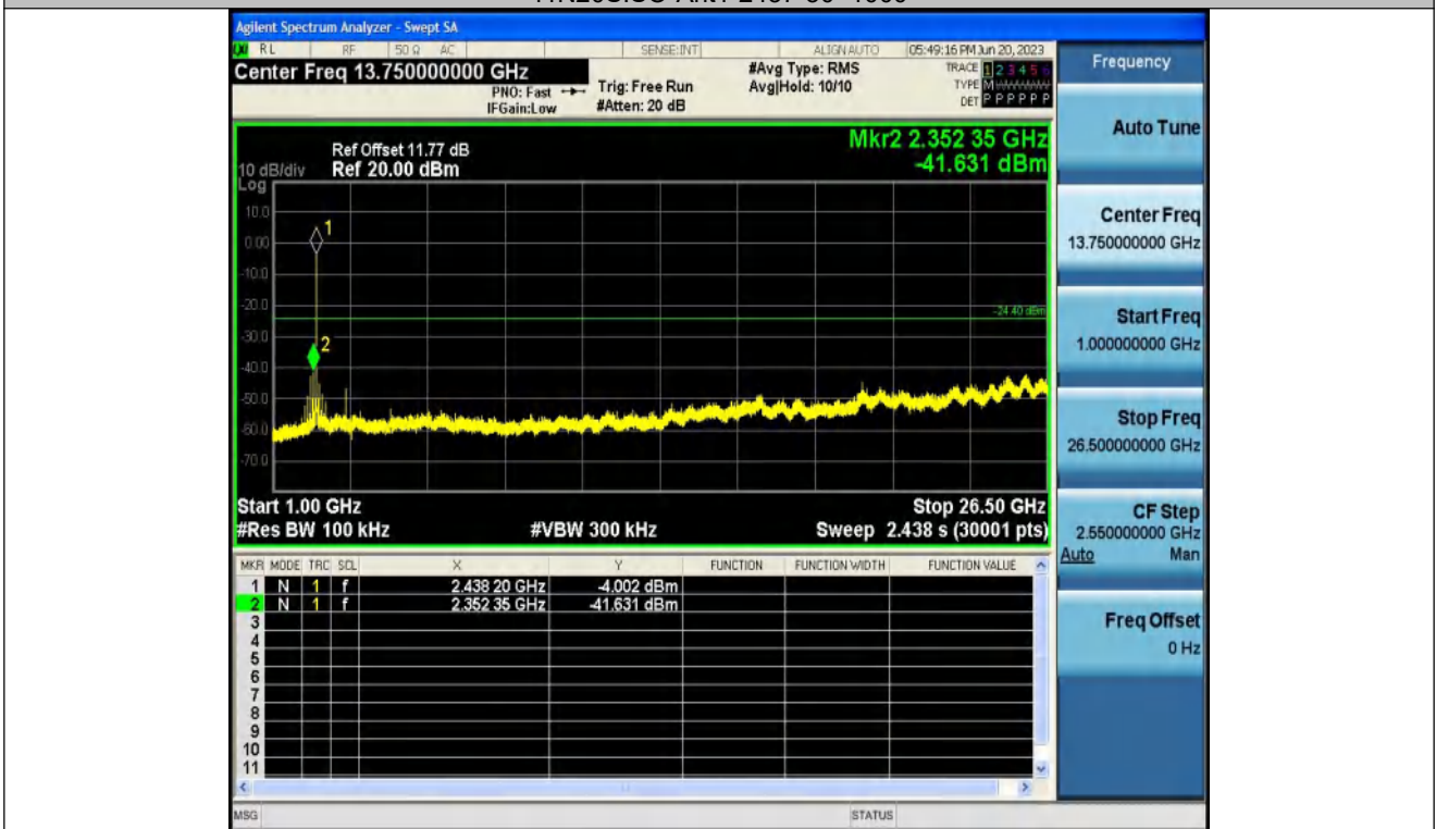
11N20SISO-Ant1-2437-1000~26500
