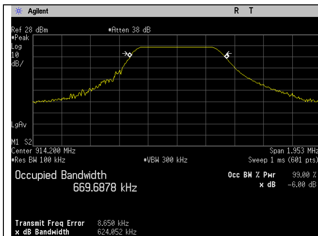
LoRa_High Ch_914.2MHz_0.5MHz BW_Occupied Bandwidth_-6dB
