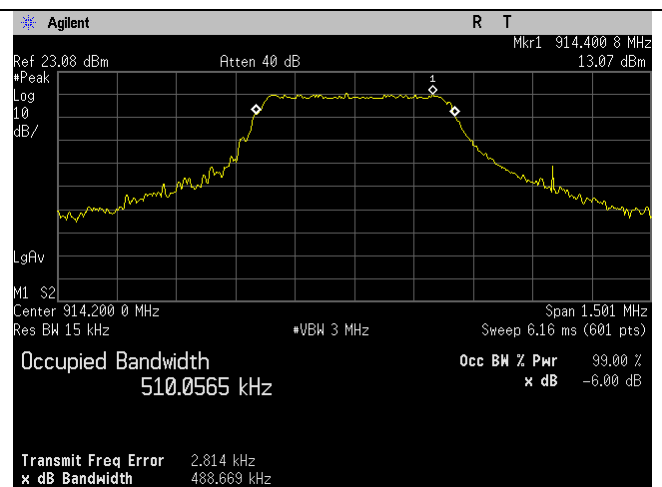
LoRa_High Ch_914.2MHz_0.5MHz BW_Occupied Bandwidth_99 percent
