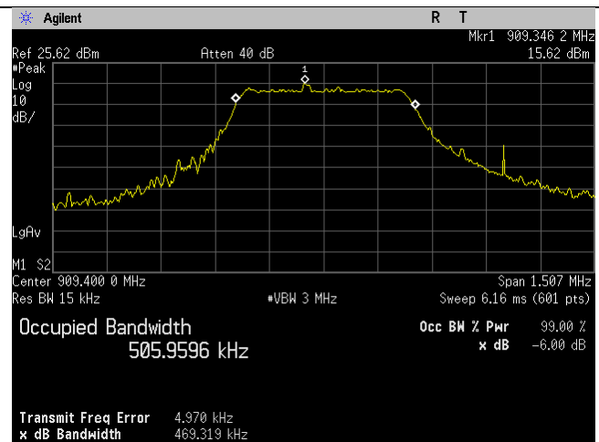
LoRa_Mid Ch_909.4MHz_0.5MHz BW_Occupied Bandwidth_99 percent
