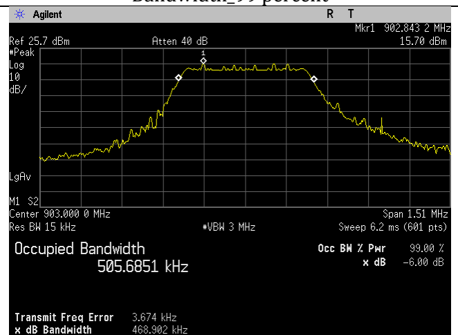
LoRa_Low Ch_903MHz_0.5MHz BW_Occupied Bandwidth_99 percent
