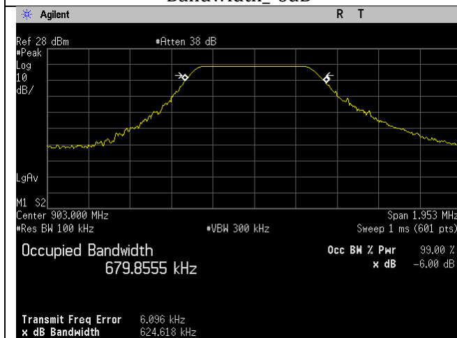
LoRa_Low Ch_903MHz_0.5MHz BW_Occupied Bandwidth_-6dB
