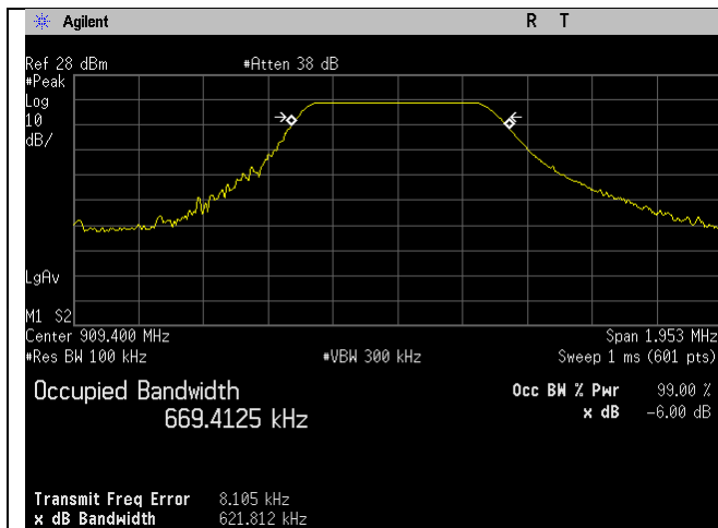
LoRa_Mid Ch_909.4MHz_0.5MHz BW_Occupied Bandwidth_-6dB
