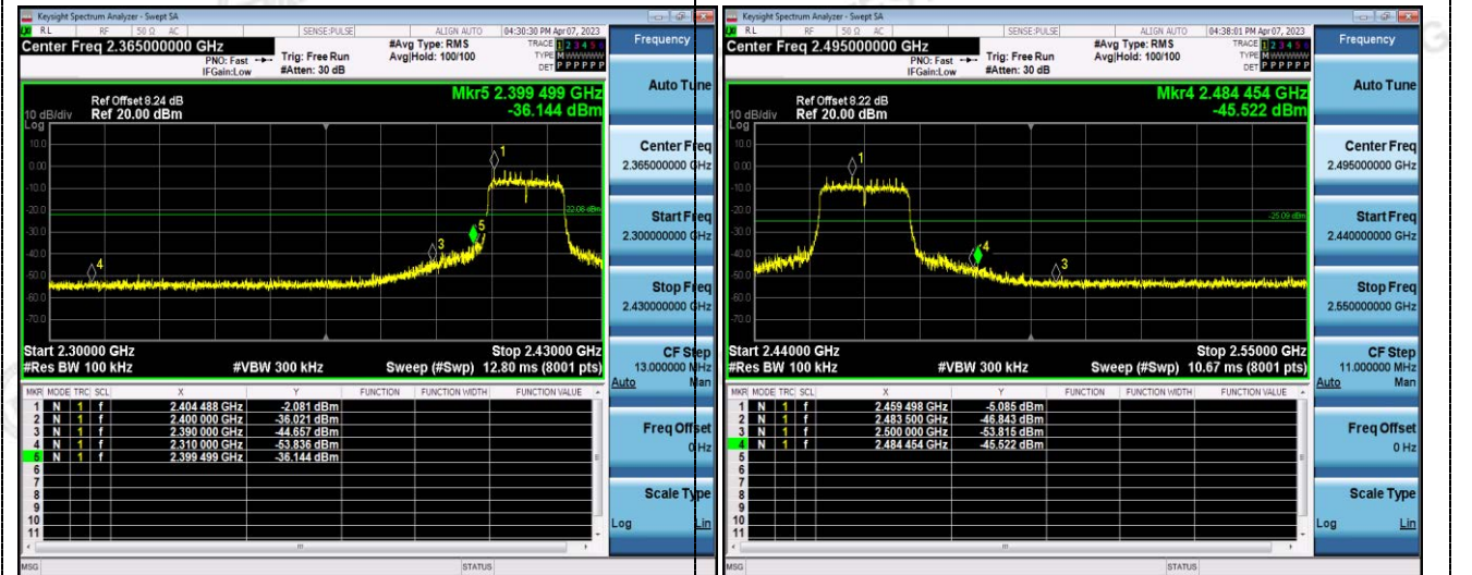
Left bandedge
