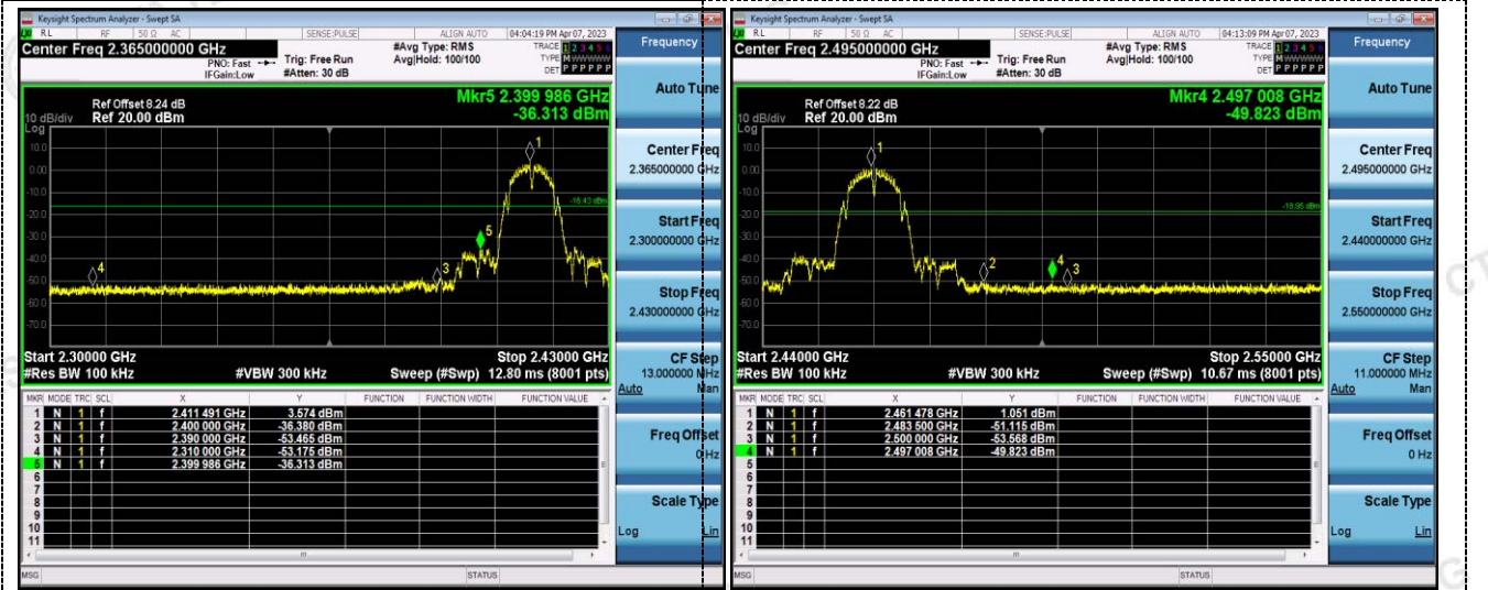
Left bandedge
