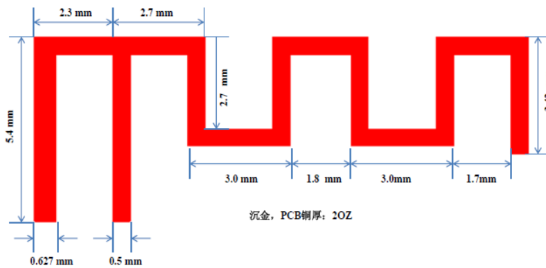
Antenna Dimension for Y00AI-ANM-T1
