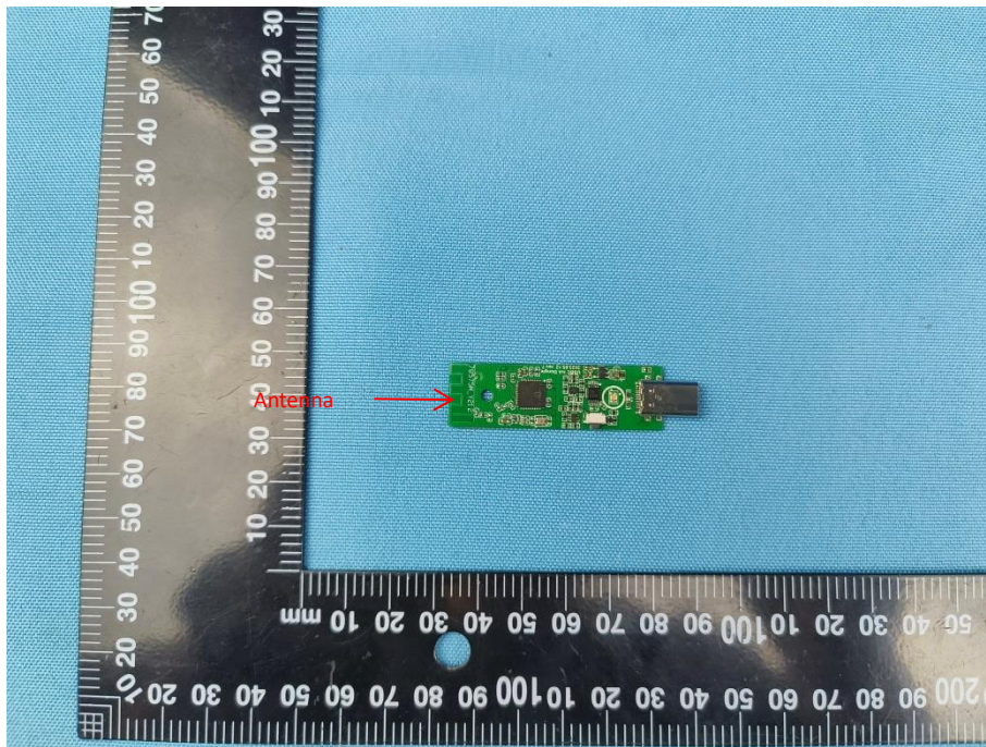
Photo 2: PCB view
