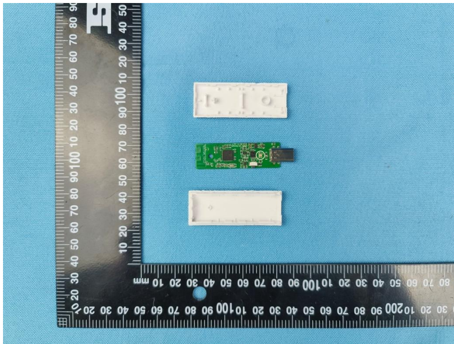
Photo 1: PCB view
