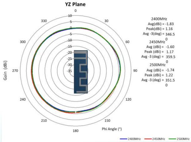
Radiation pattern Y-Z plane
