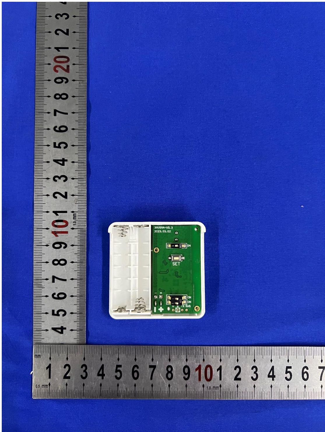
Photo 1: PCB view
