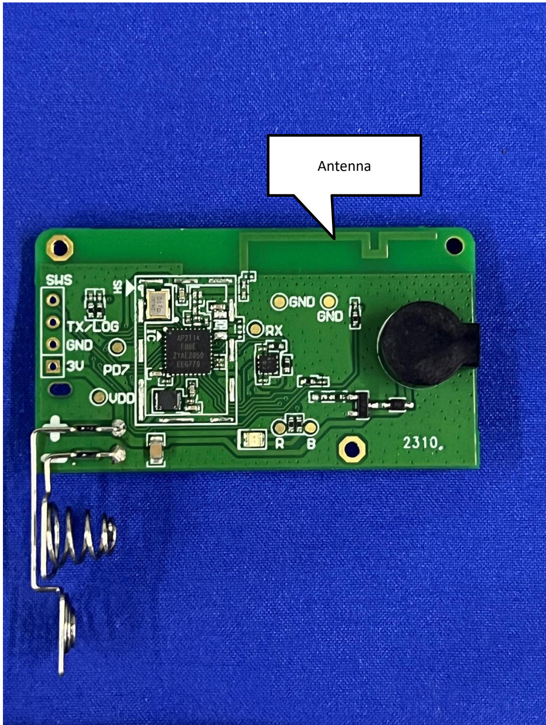
Photo 4: PCB view
