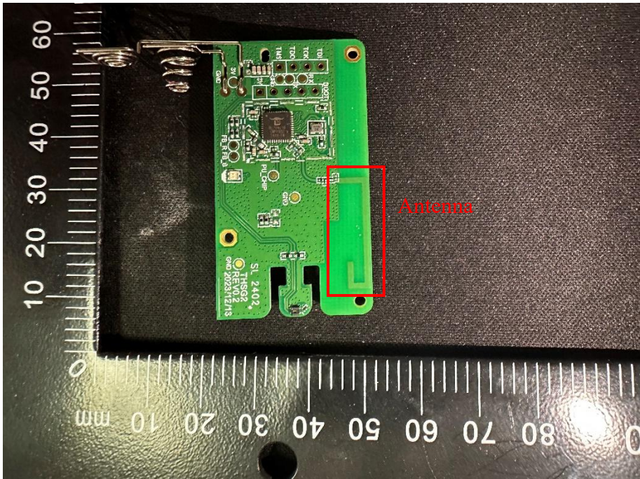
Photo 4: Antenna
