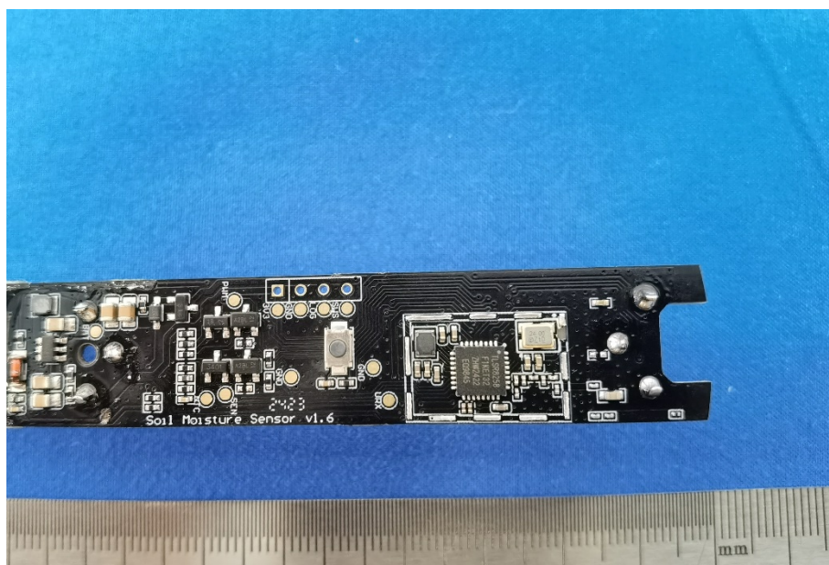
Photo 4: Internal View for PCB
