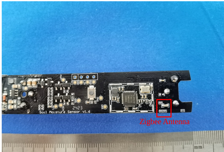
Photo 5: Antenna
