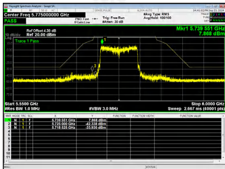
(802.11ax80) Band Edge - 5775MHz
