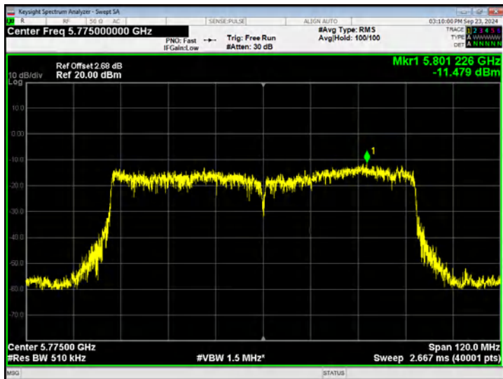
802.11ac80 - CH155
