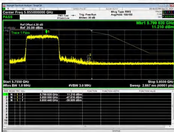
(802.11ax80) Band Edge - 5775MHz
