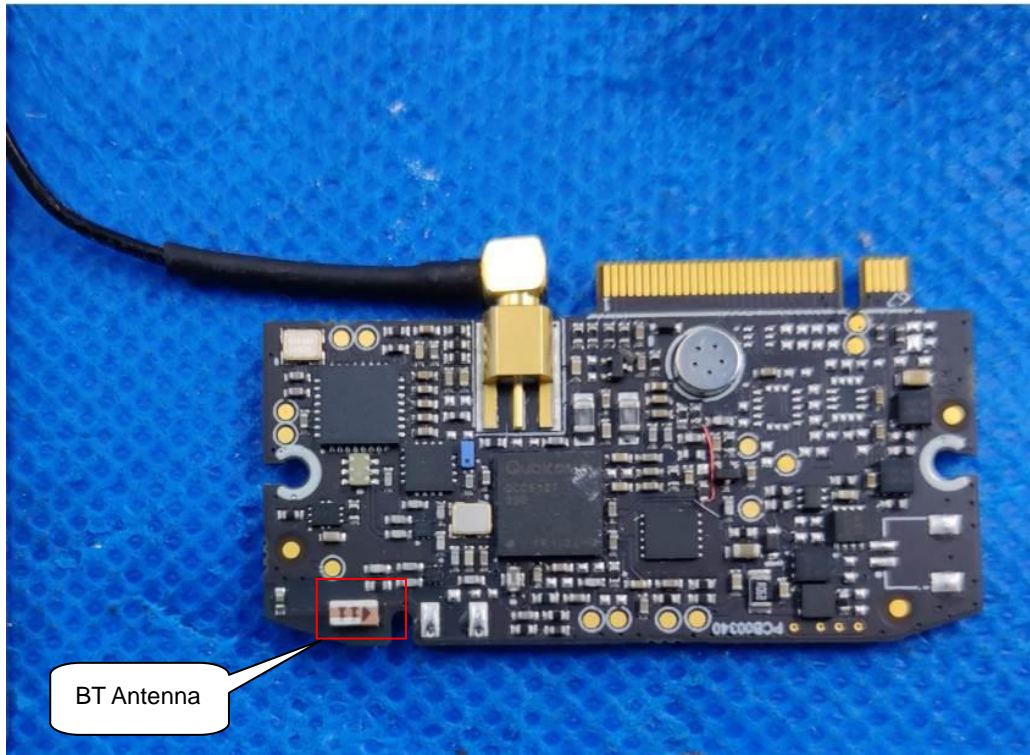
BT Antenna
