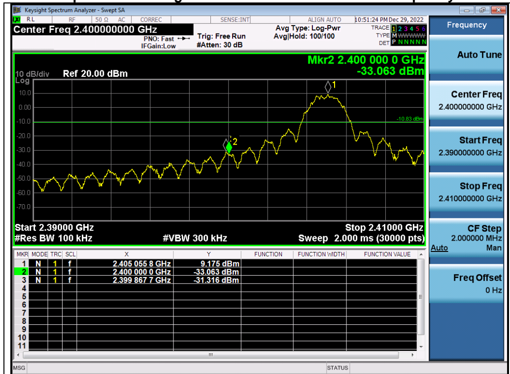
Test_Graph_Zigbee_ANT1_2405_OQPSK_Lower Band Edge Emissions
