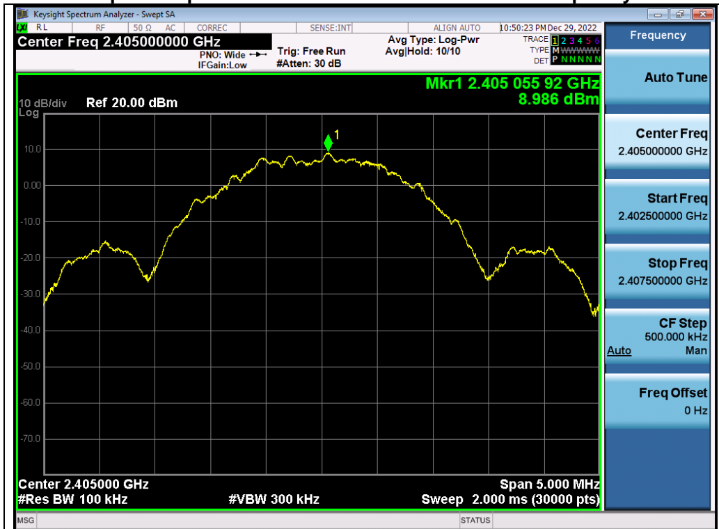
Test_Graph_Zigbee_ANT1_2405_OQPSK_Reference Level
