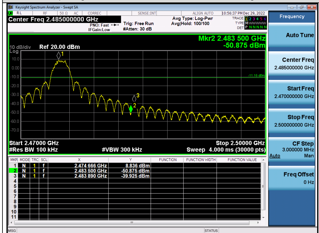
Test_Graph_Zigbee_ANT1_2475_OQPSK_Higher Band Edge Emissions
