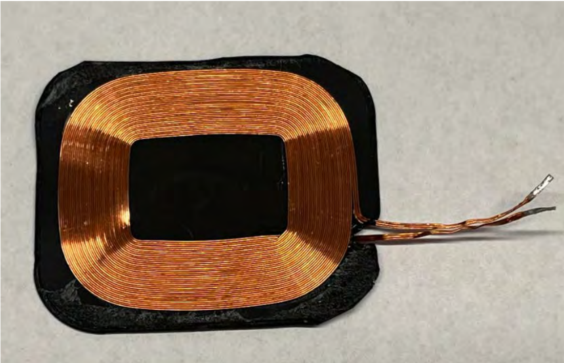
EUT Coil Antenna View
