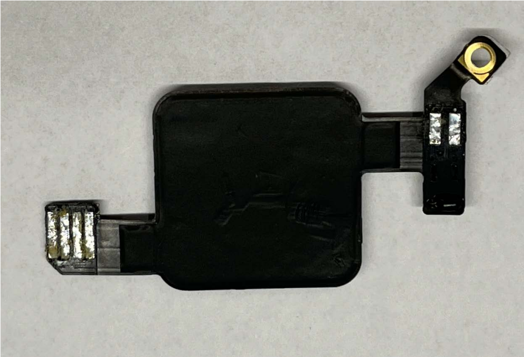
EUT Battery PCB Top View
