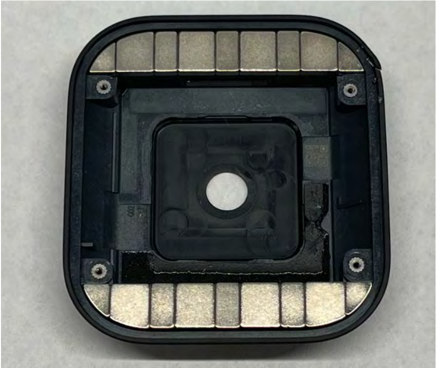
EUT Coil Antenna View
