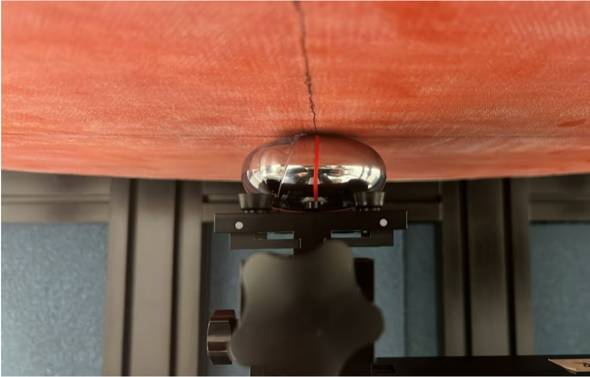
Photograph 15: Body, HU0123 + HU0223 + HU0623, Front, 0 mm
