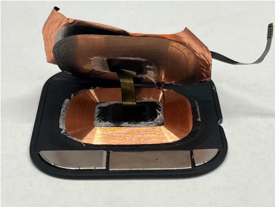
EUT Rx Coil Antenna View
