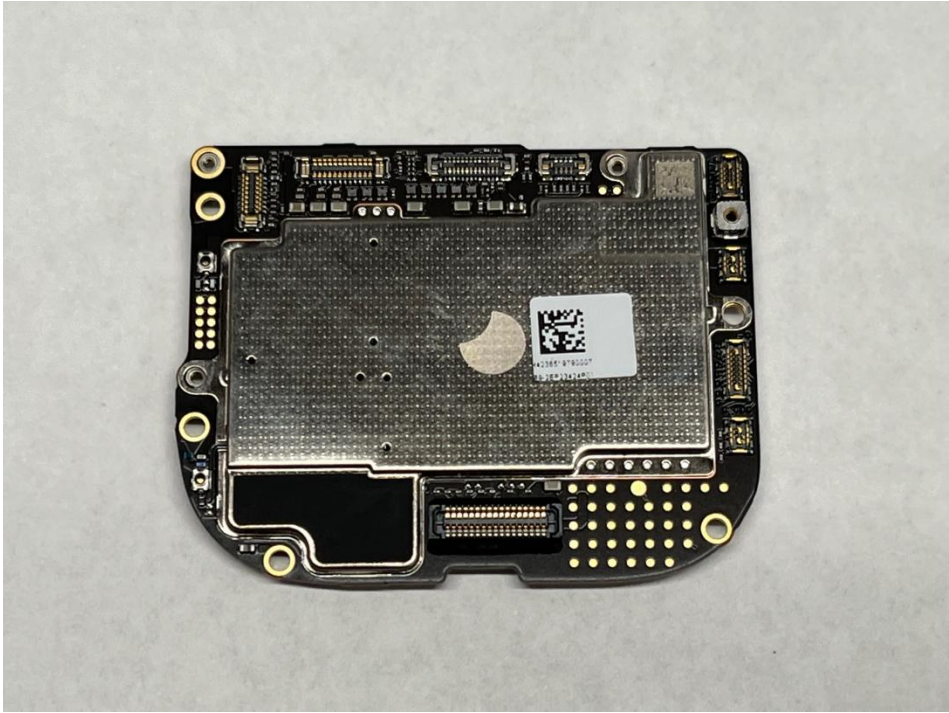
EUT PCB with Shield Can Bottom View
