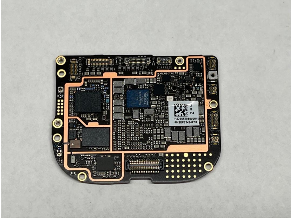
EUT PCB without Shield Can Bottom View
