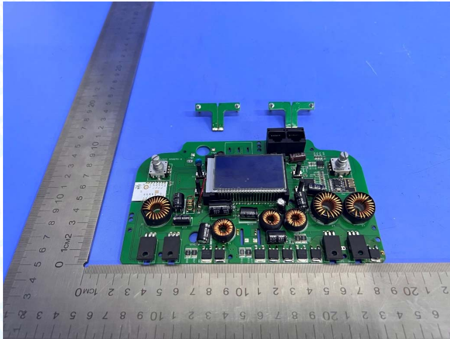
Photo 10 Appearance PCB
