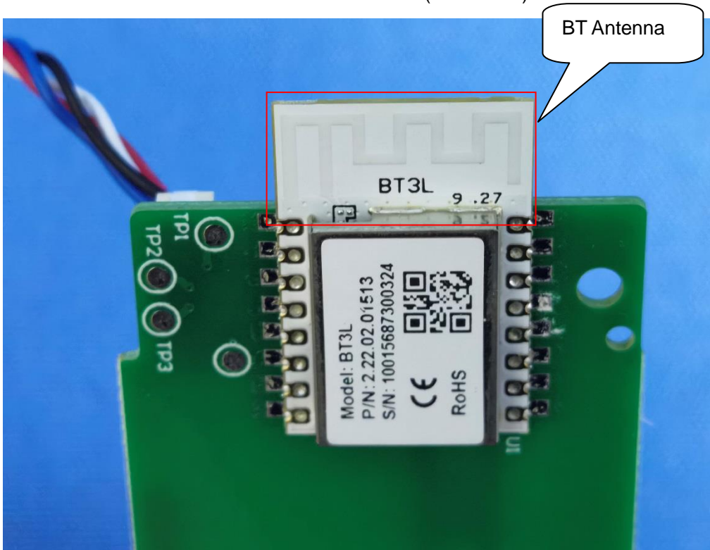
INTERNAL VIEW OF EUT (FIGURE 8)
