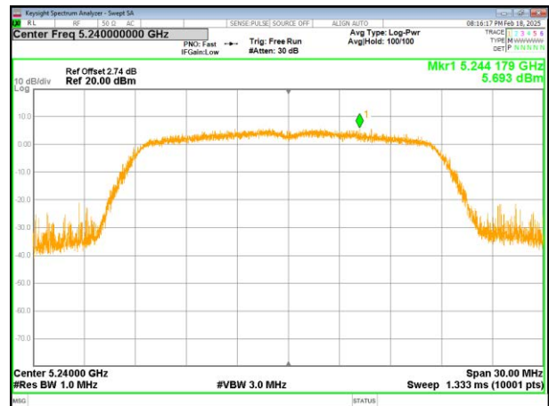
(802.11ax20) PSD plot on channel 48
