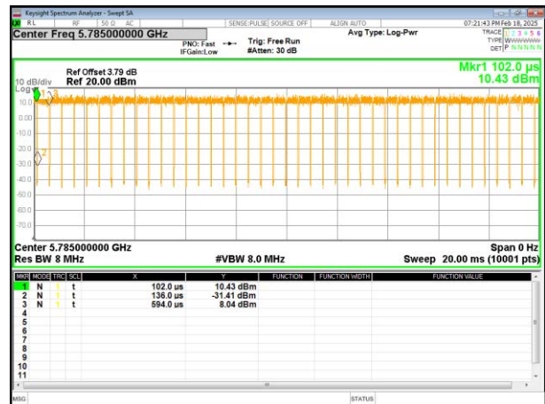
(802.11 ax20) plot
