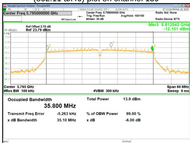
(802.11 ax40) plot on channel 159
