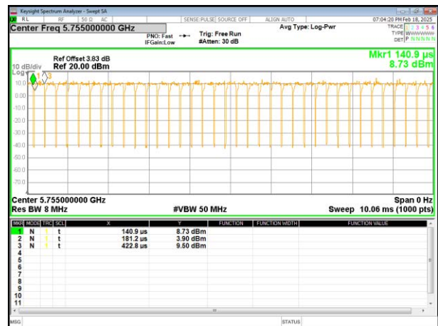
(802.11 ac40) plot
