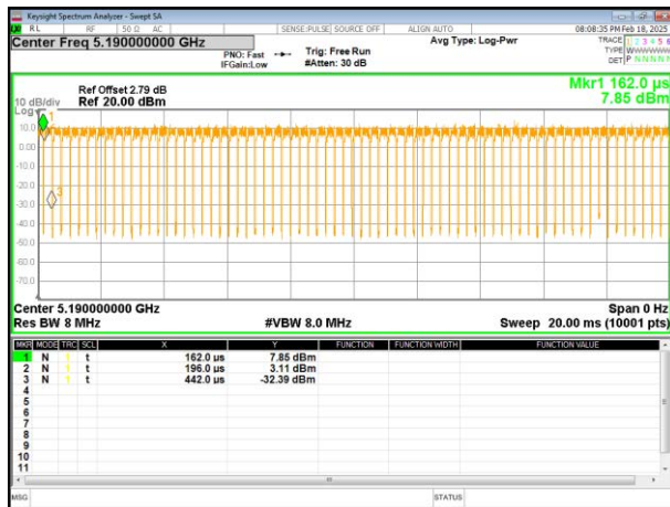
(802.11ax40) plot
