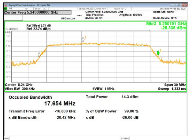
(802.11ax20) plot on channel 48
