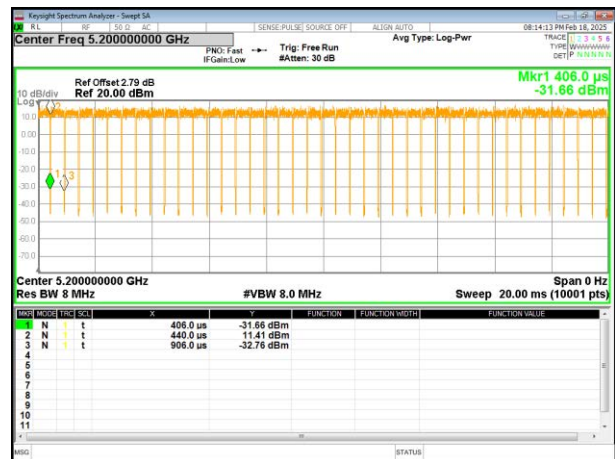
(802.11 ax20) plot
