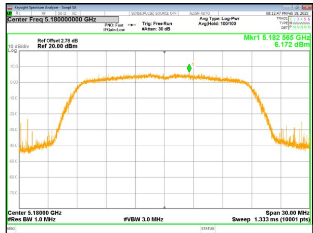
(802.11ax20) PSD plot on channel 36
