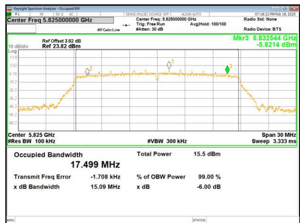
(802.11ax20) plot on channel 165
