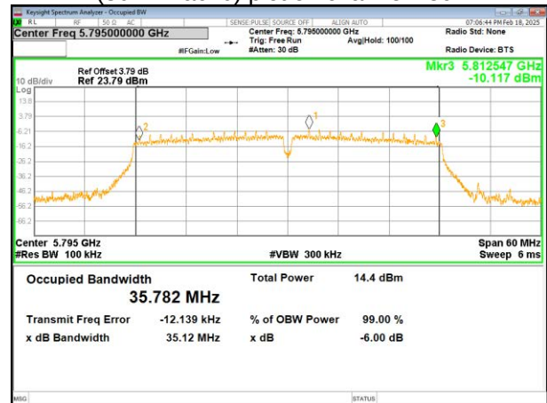
(802.11 ac40) plot on channel 159
