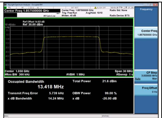
LTE band 25 - Low CH 16QAM-15
