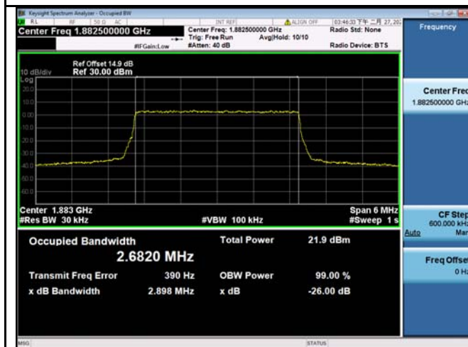
LTE band 25 - Middle CH QPSK-3
