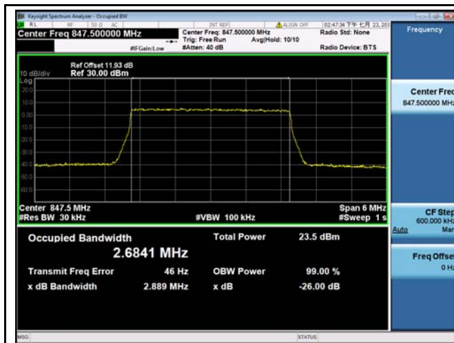
LTE band 26 - High CH QPSK-3
