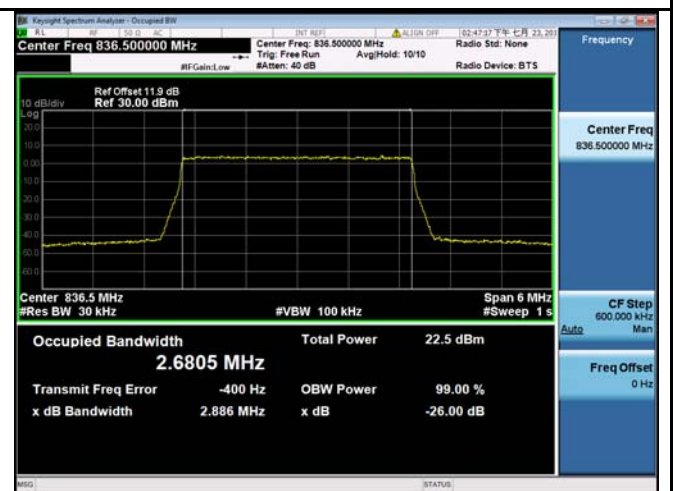
LTE band 26 - Middle CH 16QAM-3
