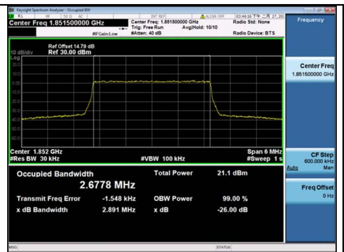
LTE band 25 - Low CH 16QAM-3
