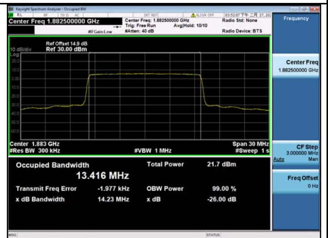
LTE band 25 - Middle CH 16QAM-15
