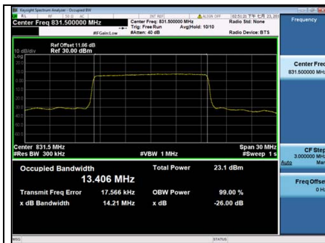
LTE band 26 - Low CH QPSK-15
