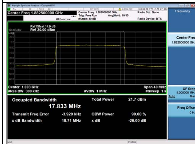
LTE band 25 - Middle CH QPSK-20
