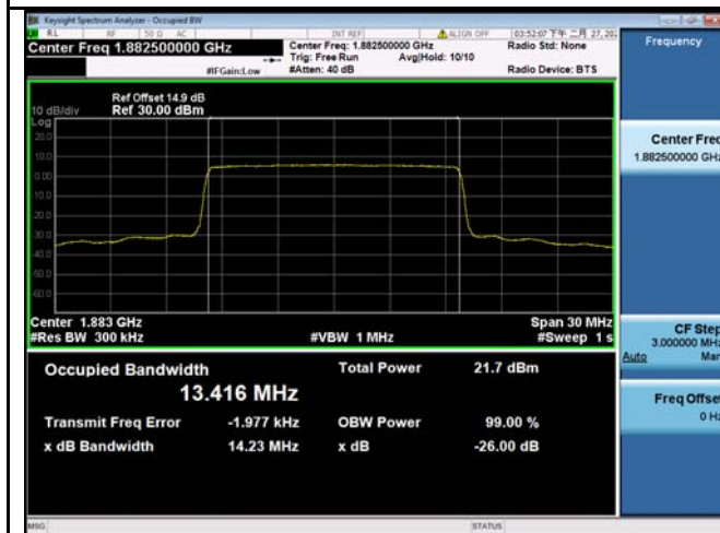
LTE band 25- Middle CH QPSK-15
