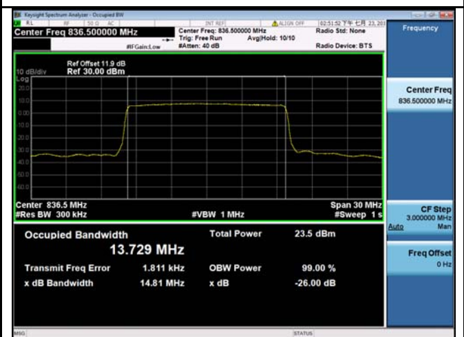
LTE band 26 - Middle CH 16QAM-15
