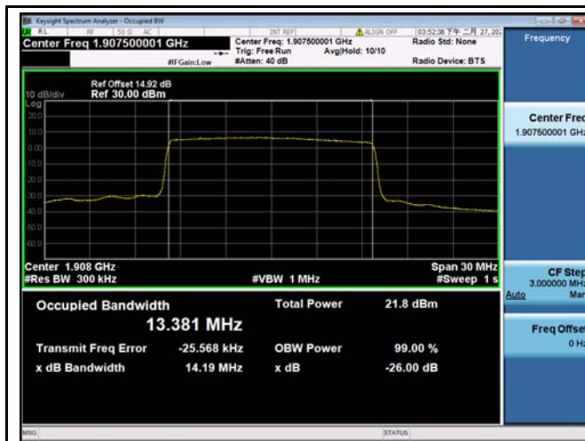
LTE band 25 - High CH QPSK-15
