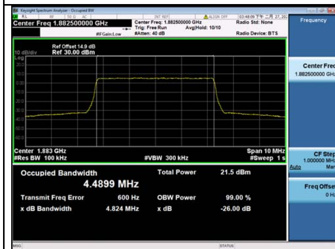
LTE band 25 - Middle CH QPSK-5
