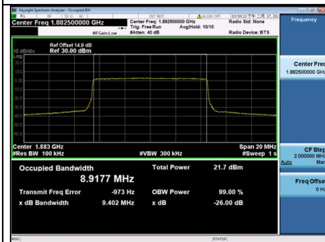
LTE band 25 - Middle CH QPSK-10
