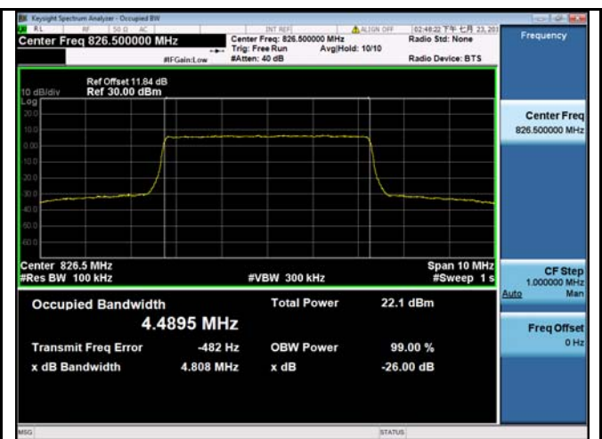
LTE band 26 - Low CH 16QAM-5
