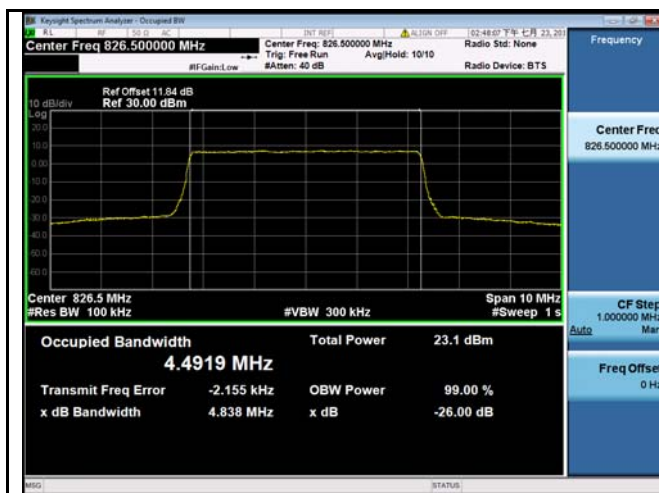
LTE band 26 - Low CH QPSK-5
