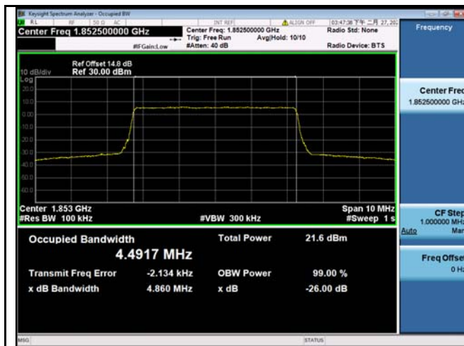
LTE band 25 - Low CH QPSK-5
