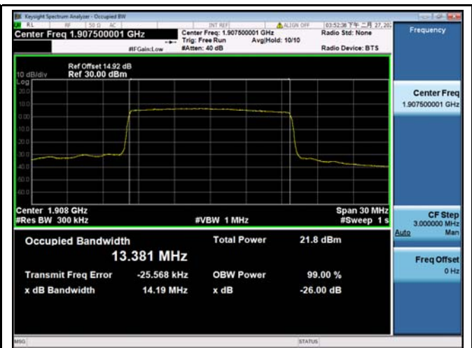
LTE band 25 - High CH 16QAM-15
