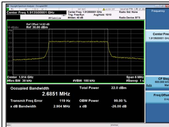
LTE band 25 - High CH QPSK-3
