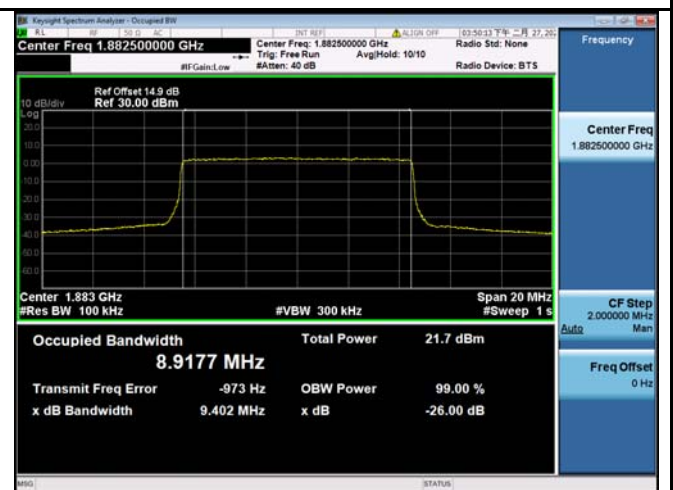
LTE band 25 - Middle CH 16QAM-10
