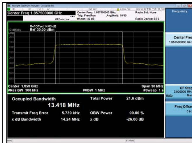
LTE band 25 - Low CH QPSK-15
