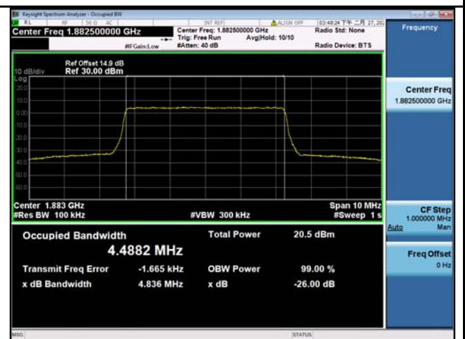
LTE band 25 - Middle CH 16QAM-5
