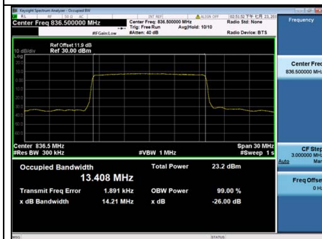
LTE band 26 - Middle CH QPSK-15
