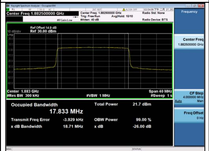
LTE band 25 - Middle CH 16QAM-20
