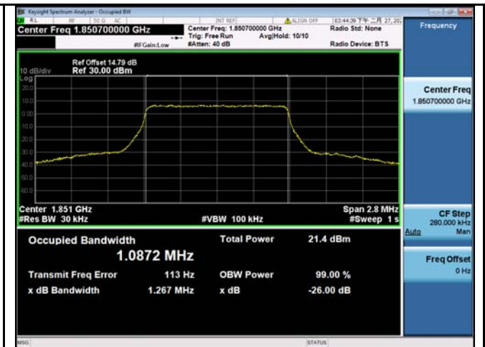
LTE band 25 - Low CH 16QAM-1.4
