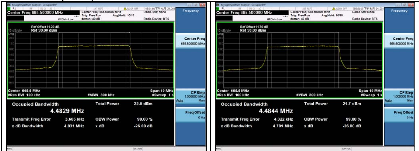
LTE band 71 - Low CH QPSK-5
