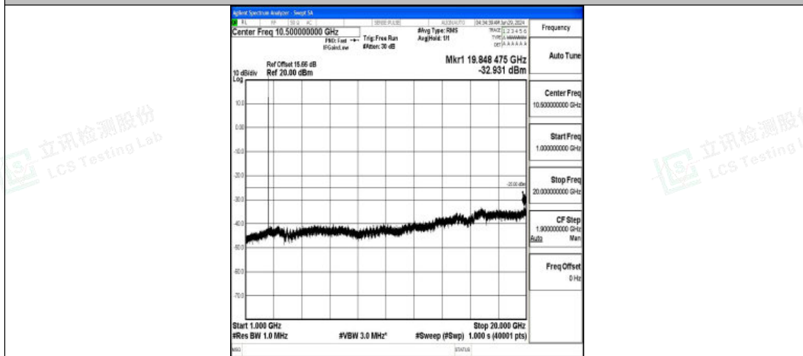
Band7_5MHz_16QAM_21425_1RB#0_1000~20000_1000~20000
