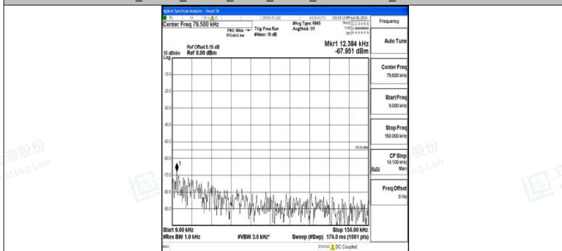
Band7_15MHz_QPSK_20825_1RB#0_0.009~0.15_0.009~0.15
