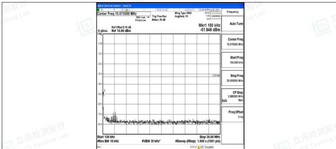
Band4_15MHz_16QAM_20175_1RB#0_0.15~30_0.15~30
