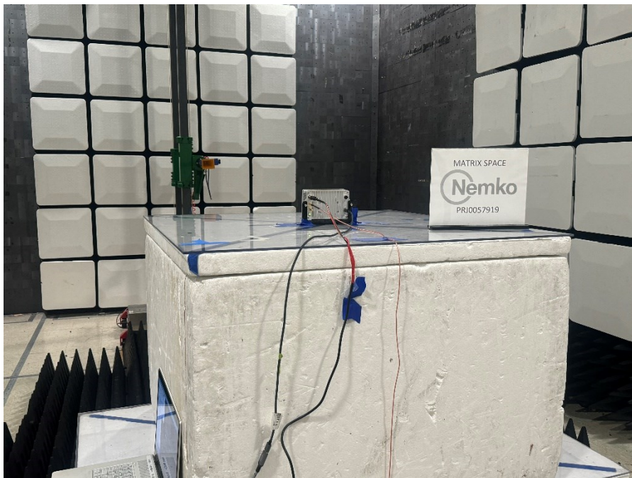
Figure 3 – Power, bandwidth and emission mask testing, rear view.
