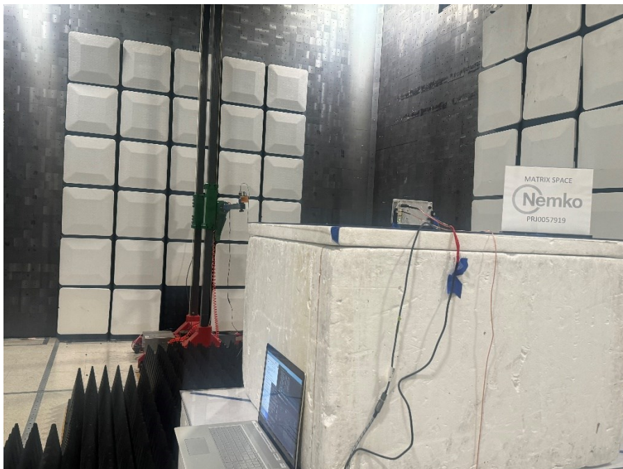
Figure 11 - Radiated emissions above 1 GHz (26.5 – 40 GHz), rear view.
