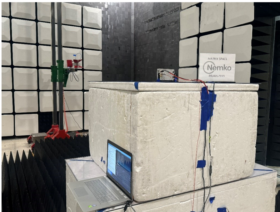
Figure 7 - Radiated emissions above 1 GHz (1–18 GHz), rear view.
