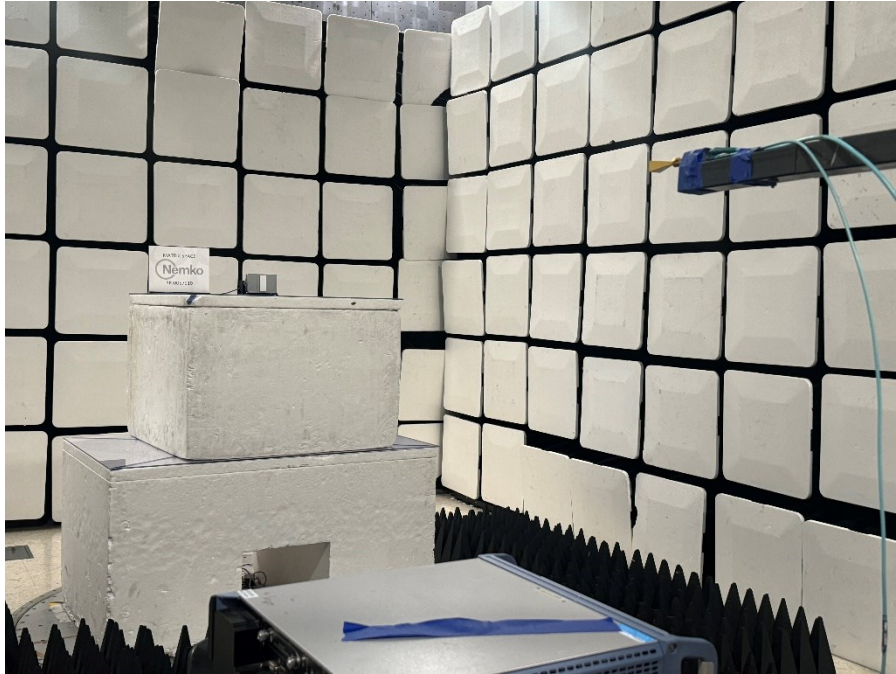
Figure 14 - Radiated emissions above 1 GHz (50 – 75 GHz), front view.
