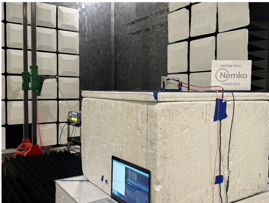
Figure 13 - Radiated emissions above 1 GHz (40 – 50 GHz), rear view.
