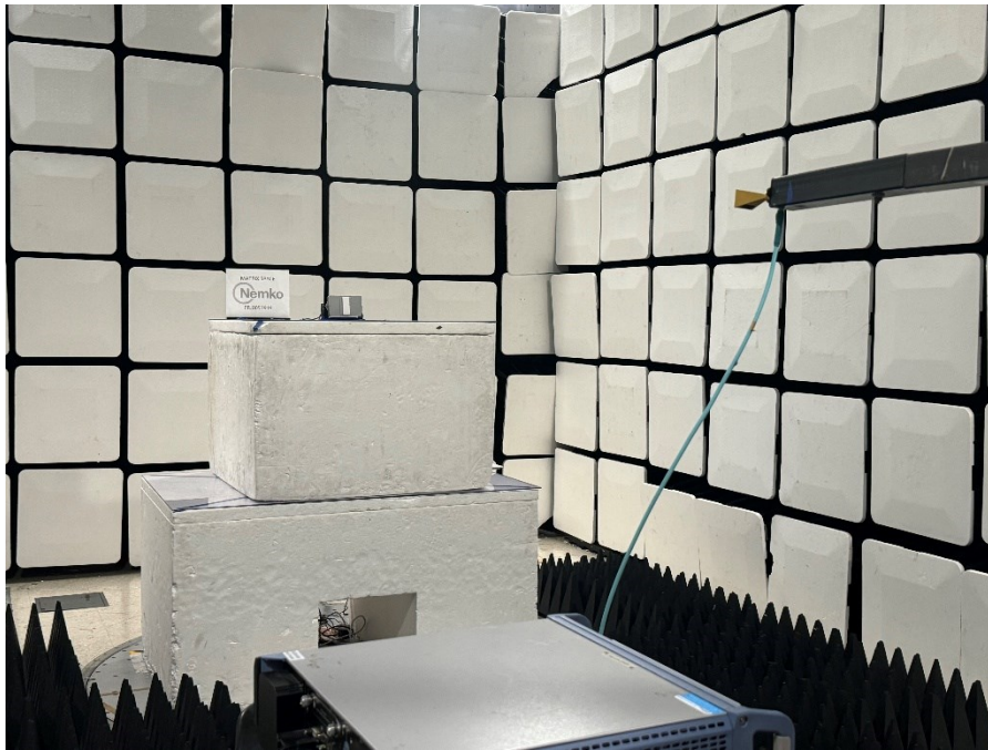
Figure 12 - Radiated emissions above 1 GHz (40 – 50 GHz), front view.
