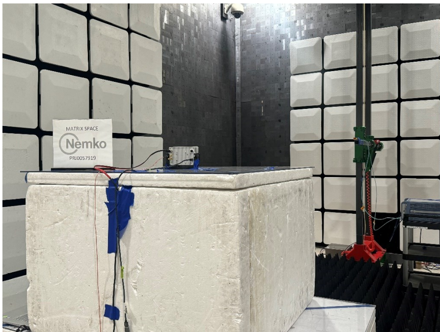
Figure 17 - Radiated emissions above 1 GHz (75 – 100 GHz), rear view.
