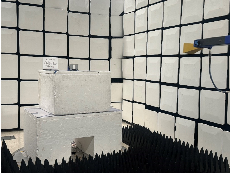
Figure 8 - Radiated emissions above 1 GHz (18 – 26.5 GHz), front view.
