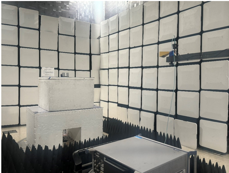
Figure 10 - Radiated emissions above 1 GHz (26.5 – 40 GHz), front view.
