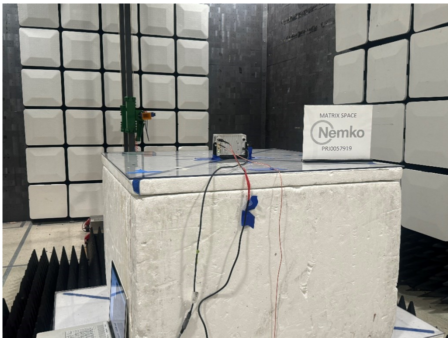
Figure 9 - Radiated emissions above 1 GHz (18 – 26.5 GHz), rear view.
