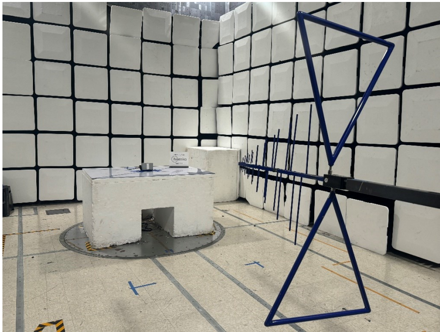
Figure 4 - Radiated emissions below 1 GHz (0.03 – 1 GHz), front view.
