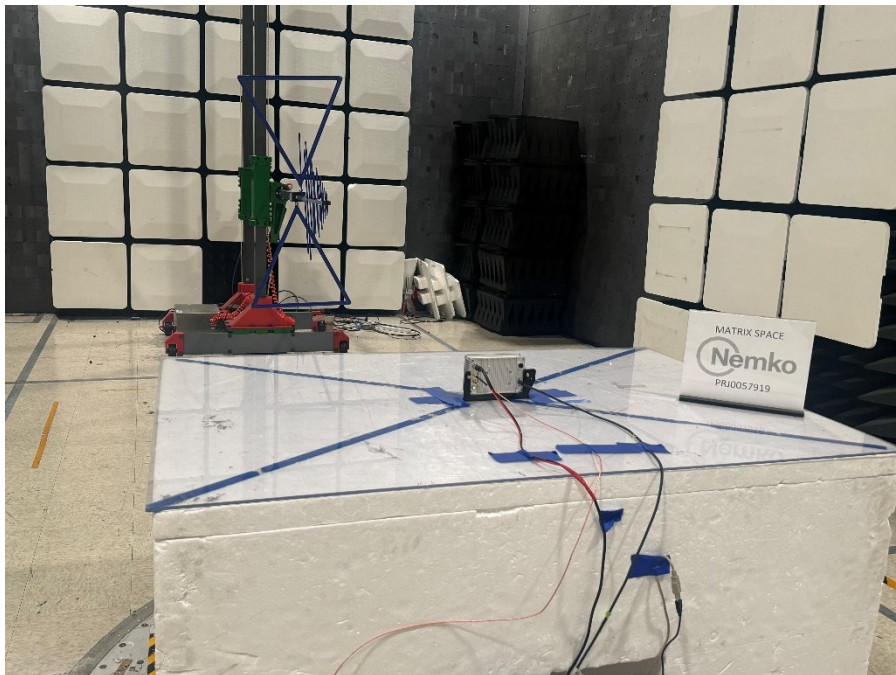
Figure 5 - Radiated emissions below 1 GHz (0.03 – 1 GHz), rear view.
