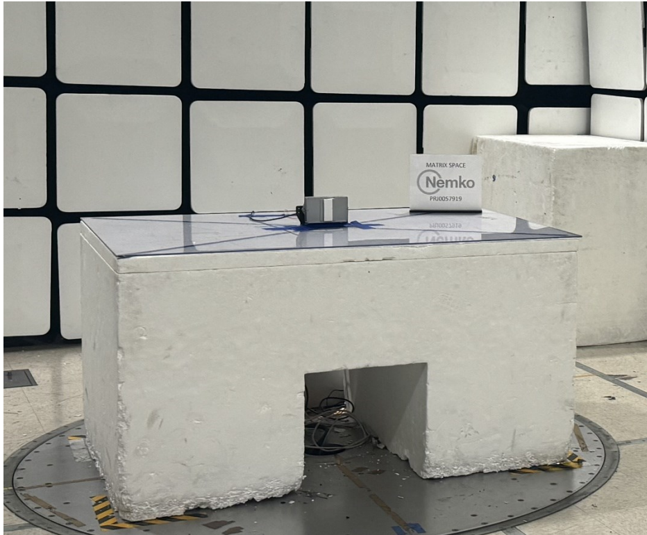
Figure 1 – Test setup.
