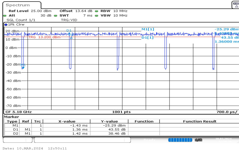
NTNV-11A-Ant1-5180-1.36-1.42
