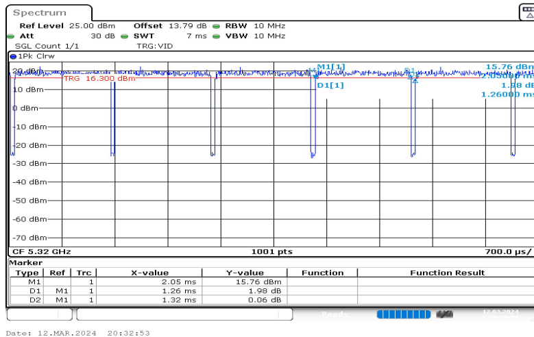
NTNV-11N20SISO-Ant1-5320-1.26-1.32
