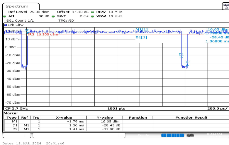
NTNV-11A-Ant1-5700-1.36-1.41
