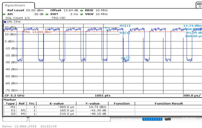
NTNV-11N20SISO-Ant1-5200-0.16-0.21
