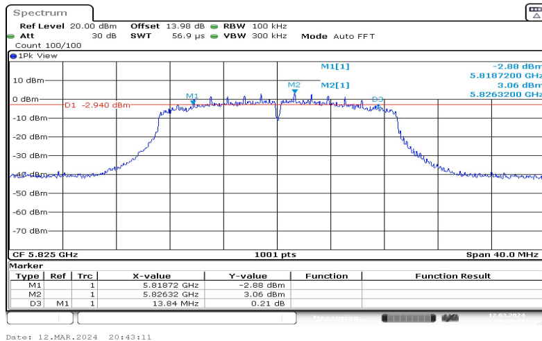
11N20SISO-Ant1-5825
