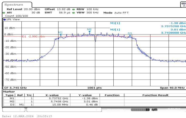
11N20SISO-Ant1-5745
