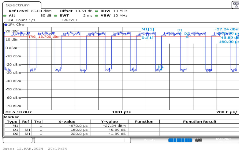
NTNV-11N20SISO-Ant1-5180-0.16-0.22
